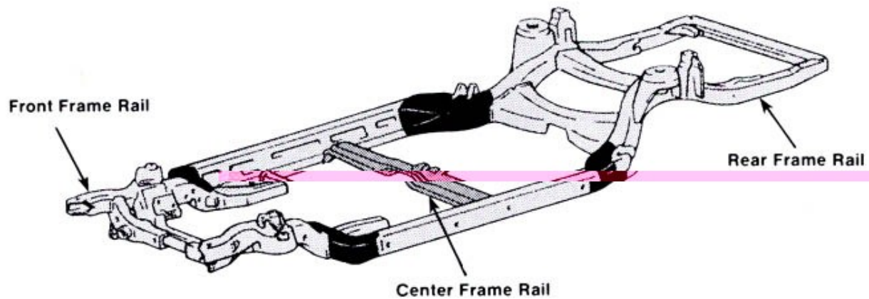
FIGURE 2-18 Perimeter frame featuring a center rail. Shaded portions are torque box structure. (Courtesy of Toyota Motor Corp.)
