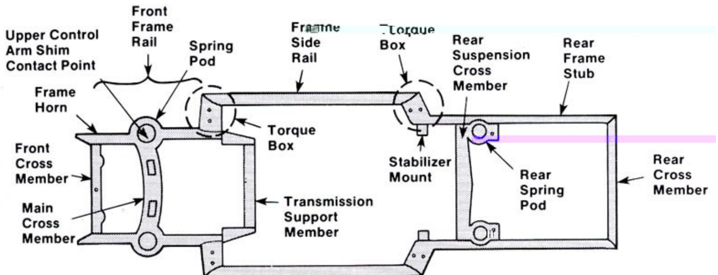
FIGURE 2-17 Perimeter frame terminology
