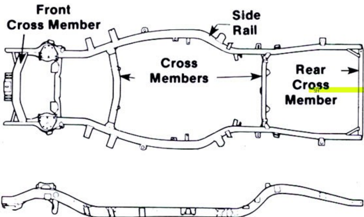
FIGURE Modern ladder frame used in some small trucks
