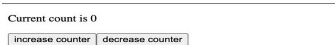
Figure 4.1: Counter app
