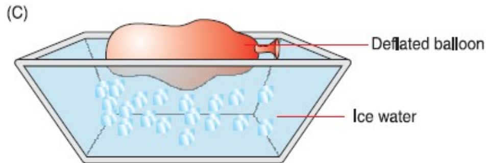
Figure: Relationship between the volume of air in the balloon and its temperature
