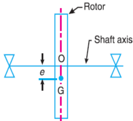
(a) When shaft is stationary.
