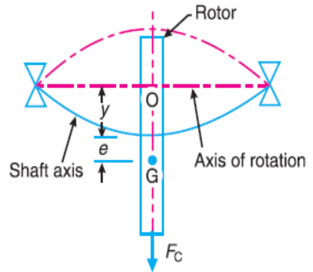
(b) When shaft is rotating.
