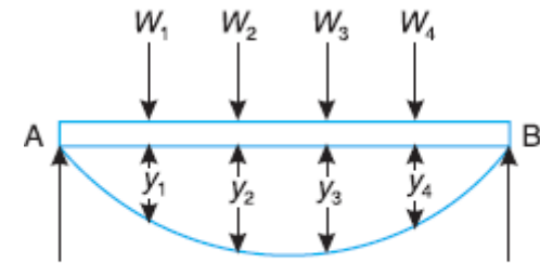
■ Fig. 23.11. Shaft carrying a number of point loads.
