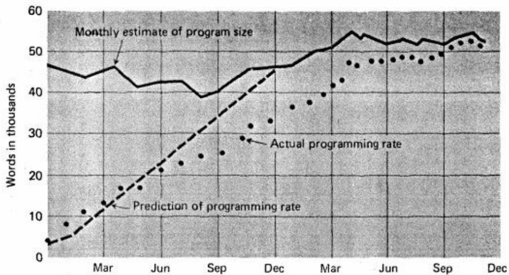
Fig. 8.4 ESS predicted and actual debugging rates
