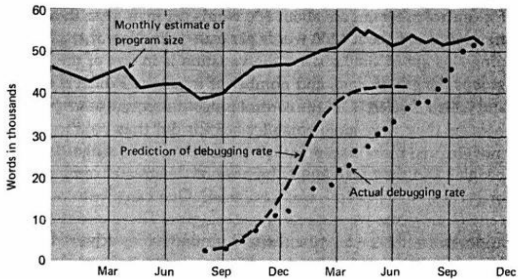
Fig. 8.3 ESS predicted and actual programming rates
