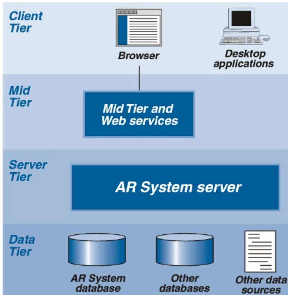
F. AR System architecture[24]
