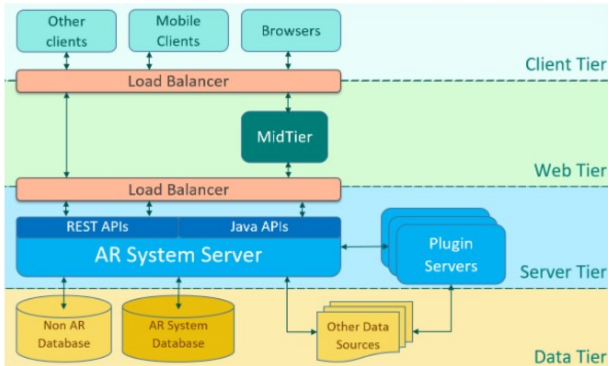
F. High-level architecture of the AR System
