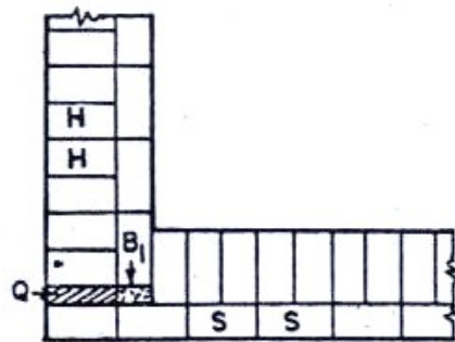
(b) Plan for 1\frac{1}{2} Brick Thick Wall
