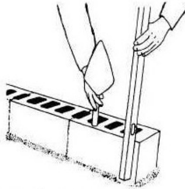
2. Plumbing Block
