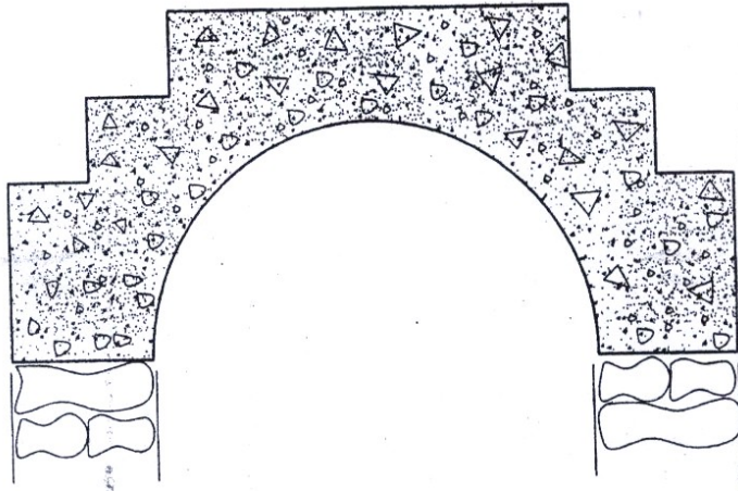
Precast concrete arch lintel
