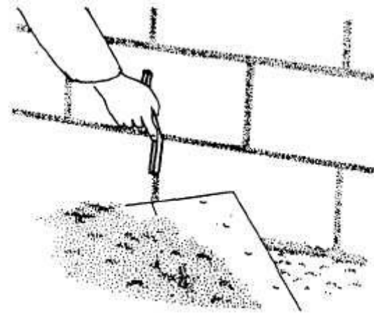
2. Striking Vertical Joints
