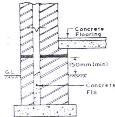
(c) Cavity Concreted Upto G.L.
