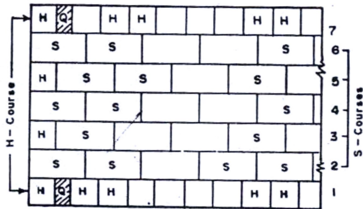
(a) Garden Wall English Bond
