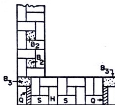
(b) Plan for 1\frac{1}{2} Brick Thick Wall
