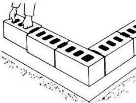
1. PLACING BLOCKS WITHOUT MORTAR (CHASING THE BOND)
