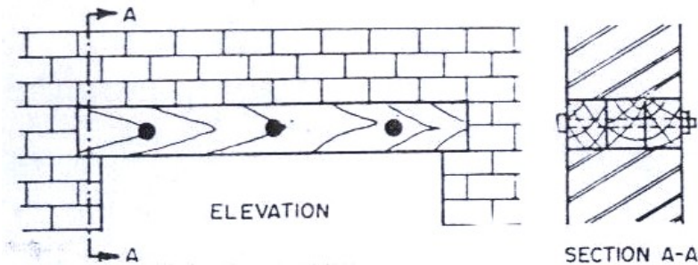
Timber lintel
