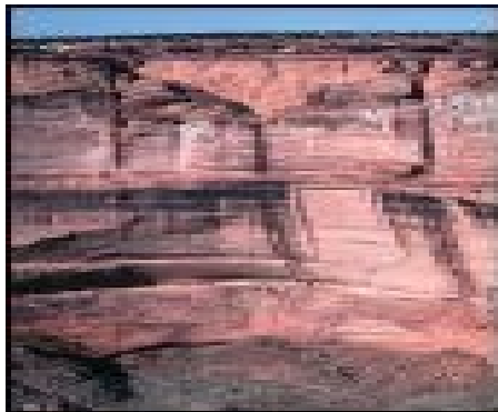
Sedimentary rock e.g. limestone, shale
