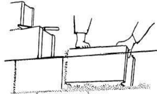
Filling in the walls b/n corners
