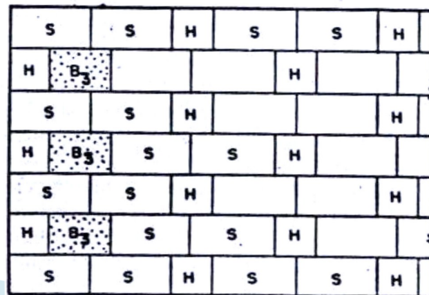
(c) Monk Bond
