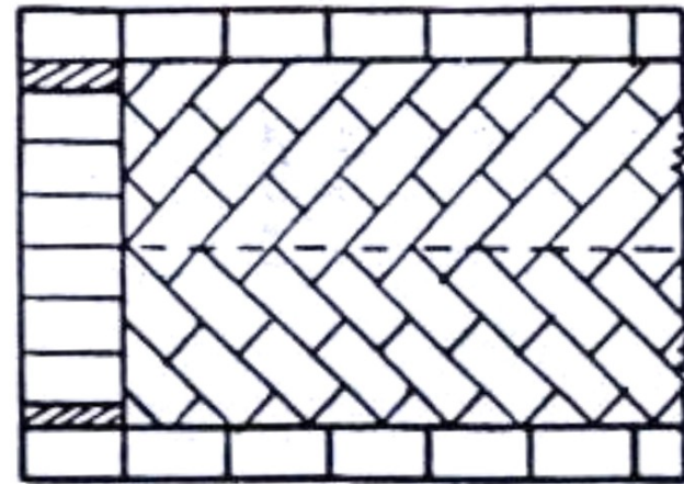
(b) Herring-bone Bond
