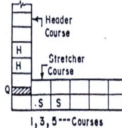
(a) Plan for 1 Brick Thick Wall
