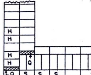
(c) Plan for 2-Brick Thick Wall
