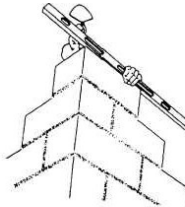
2. Leveling
