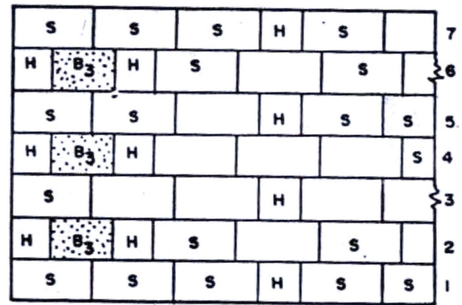
(b) Garden Wall Flemish Bond
