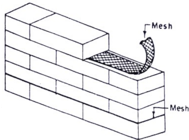
(b) Steel Mesh Reinforcement
