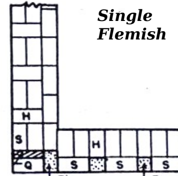
1, 3, 5 --- Courses
