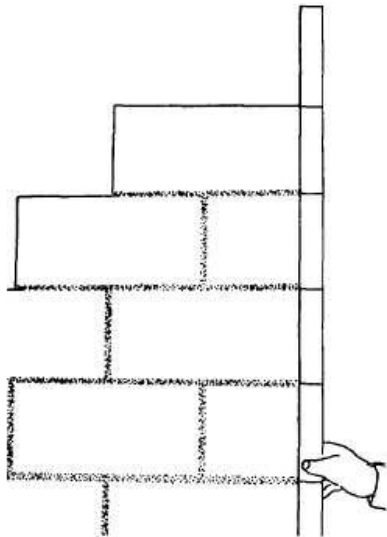
Story or course pole
