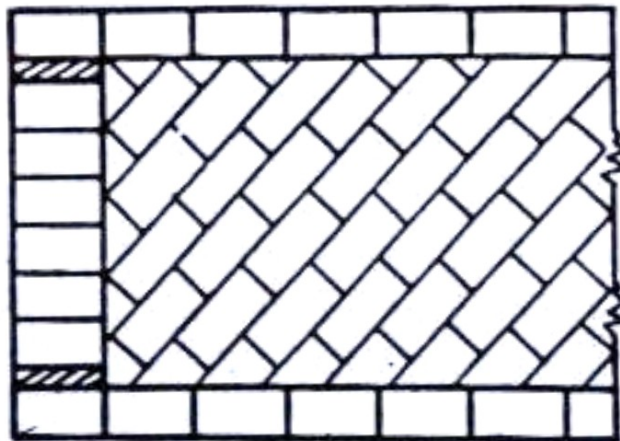
(a) Diagonal Bond
