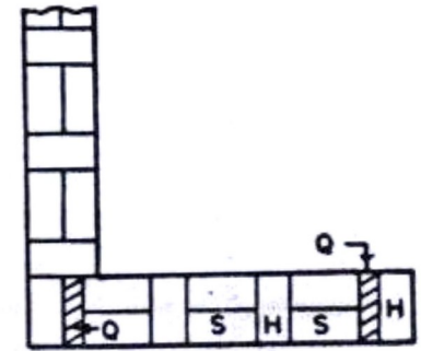
2, 4, 6 --- Courses
