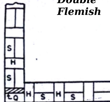
1, 3, 5 --- Courses
