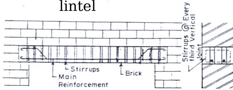
Reinforced brick lintel
