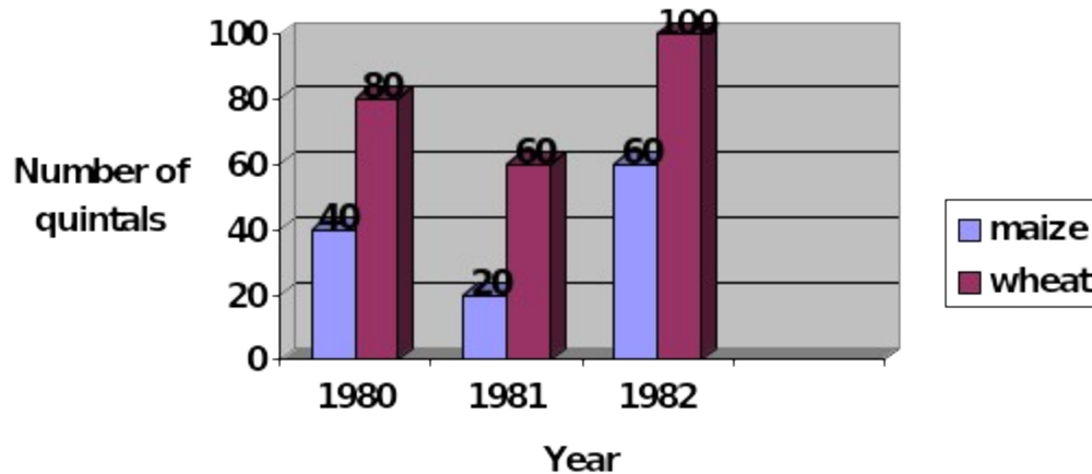
The number of quintals(in thousands) of wheat and maize production
