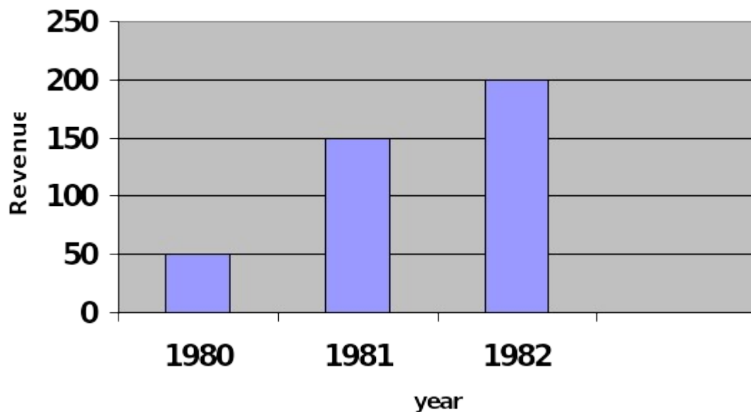
A simple bar chart showing revenues of company X from 1980 to 1982
