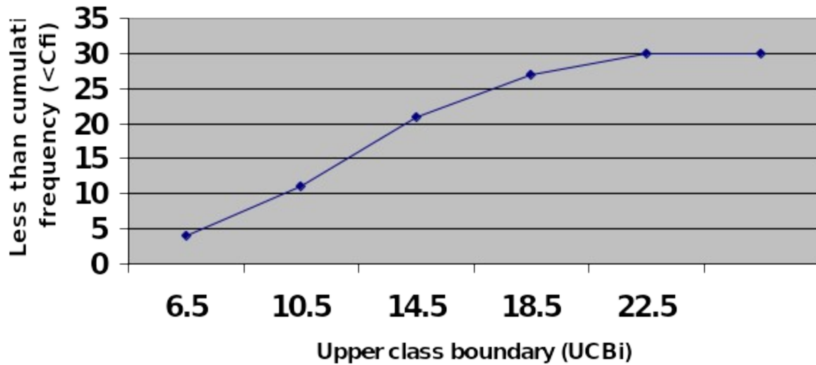
A less than ogive showing the frequency distribution above
