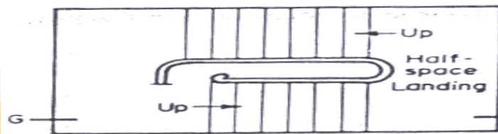
(a) With Landing
