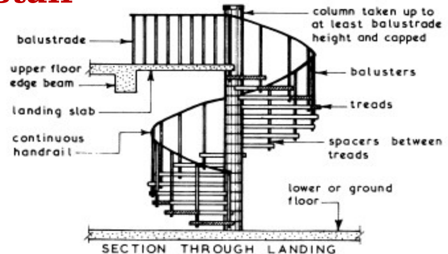
Spiral stair
