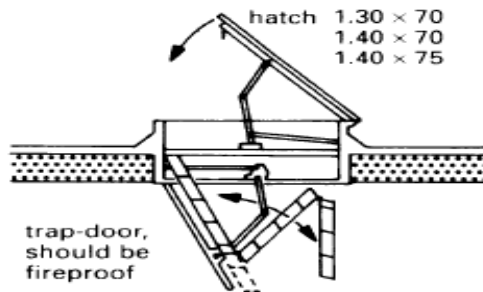
⑧ Flat roof exit with loft steps
