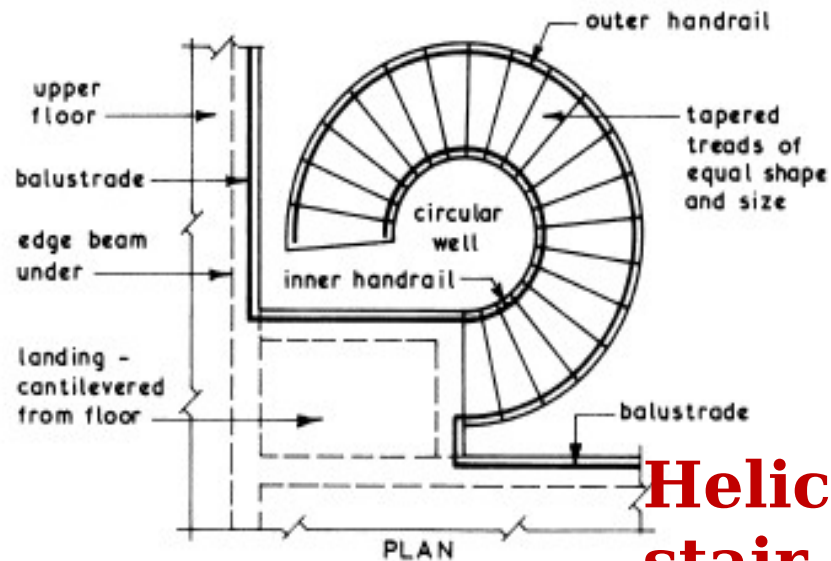
Typical Example of a Helical Stair -
