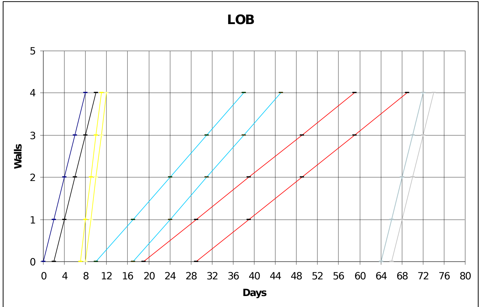
Fig___ LOB Schedule for construction of retaining wall
