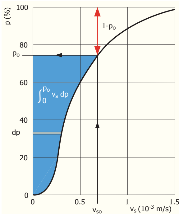
Figure 9 - Cumulative frequency distribution of settling velocities
