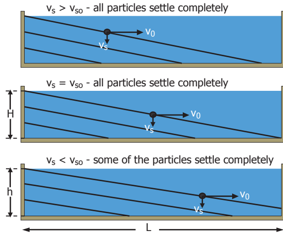
Figure 7 - Settling of a suspension in a horizontal flow settling tank
