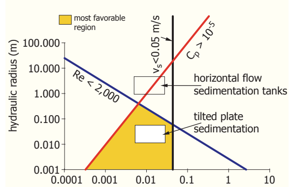
Figure 31 - Hydraulic conditions for optimal settling
