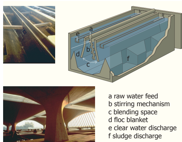
Figure 27 - Floc blanket installation at Berenplaat
