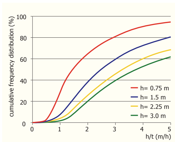
Figure 17 - Cumulative frequency distribution of settling velocities at different tank depths
