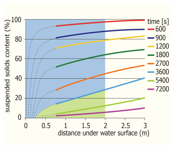
Figure 18 - The relative particle concentration
