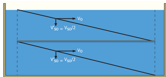
Figure 28 - Tray settling
