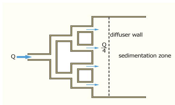
Figure 20 - Inlet construction
