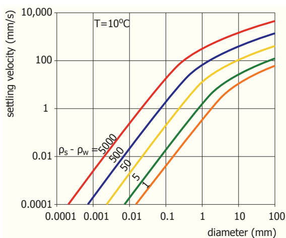
Figure 5 - Settling velocity of discrete spherical particles
