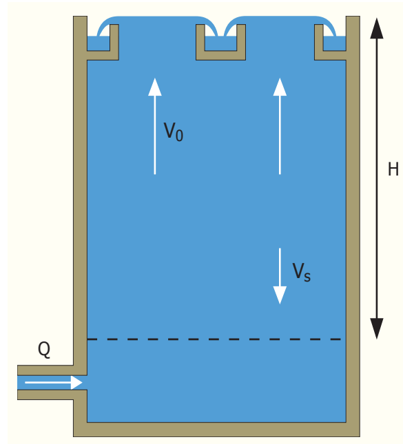
Figure 25 - Vertical flow settling
