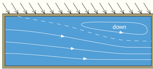
Figure 14 - Short-circuit flow caused by wind
