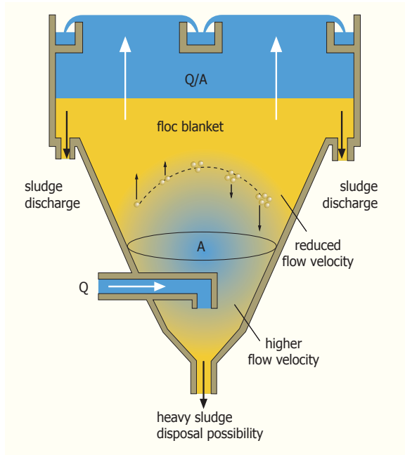
Figure 26 - Floc blanket installation
