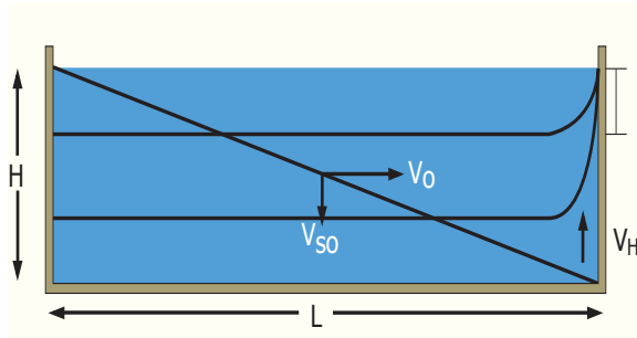
Figure 23 - Upward velocity to overflow weir
