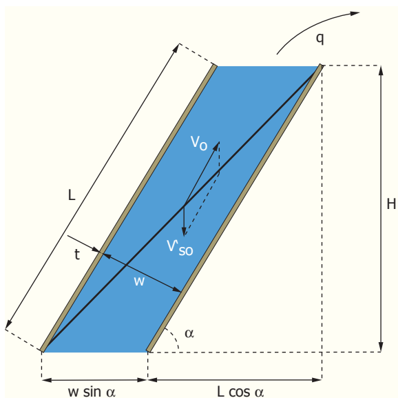
Figure 30 - Flow through a tilted plate settler
