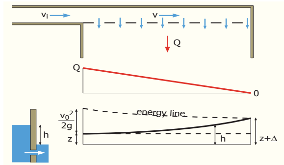
Figure 21 - Diffuser wall
