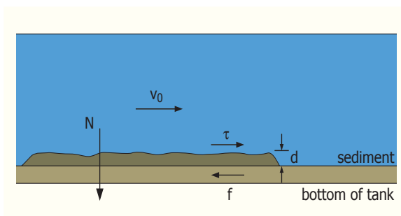
Figure 15 - Bottom scour
