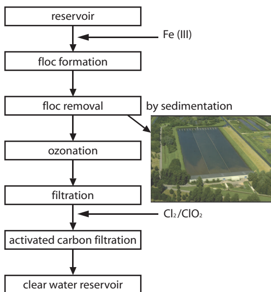
Figure 1 - Process scheme of a surface water treatment plant
