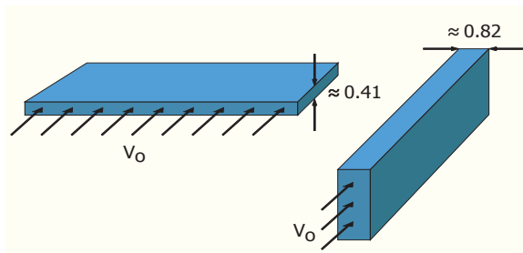
Figure 19 - Settling tanks with laminar and stable flows
