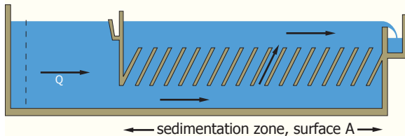
Figure 29 - Counter-current tilted plate settling
