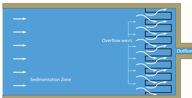
Figure 24 - Outlet construction: overflow weir for effluent discharge
