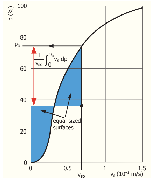
Figure 10 - Efficiency of partial settling
