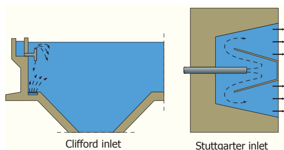
Figure 22 - Clifford and Stuttgarter inlet
