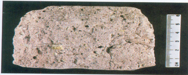
FIGURE 1.35 Rhyolite tuff.
