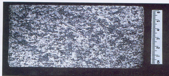
FIGURE 1.57 Granulite.
