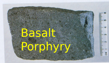
FIGURE 1.32 Basalt porphyry.
