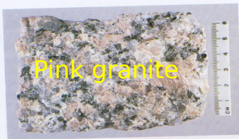
FIGURE 1.25 Pink granite.
