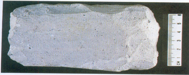
FIGURE 1.33 Rhyolite.
