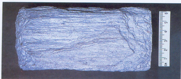
FIGURE 1.54 Phyllite.
