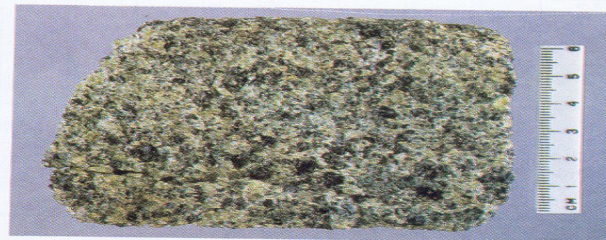
FIGURE 1.40 Peridotite.
