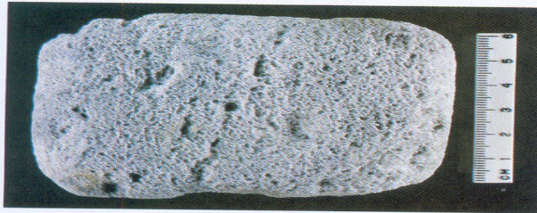
FIGURE 1.37 Pumice.
