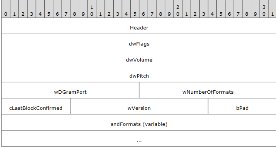
Fig. 6. RDPSND Server Audio Formats and Version PDU structure.
