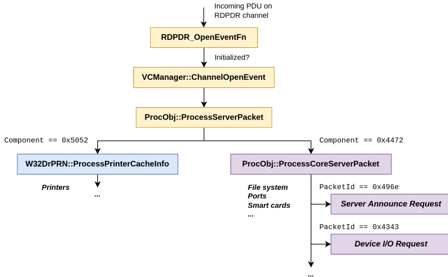
Fig. 8. RDPDR channel architecture in mstscax.dll and header structure.
