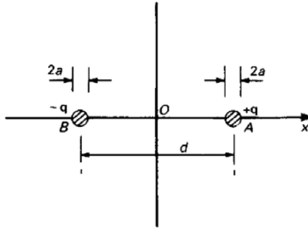
Fig. 2.3 Cross-sectional view of a parallel-wire transmission line
