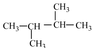
2,3-Dimethylbutane
