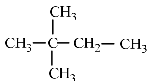
2,2-Dimethylbutane
