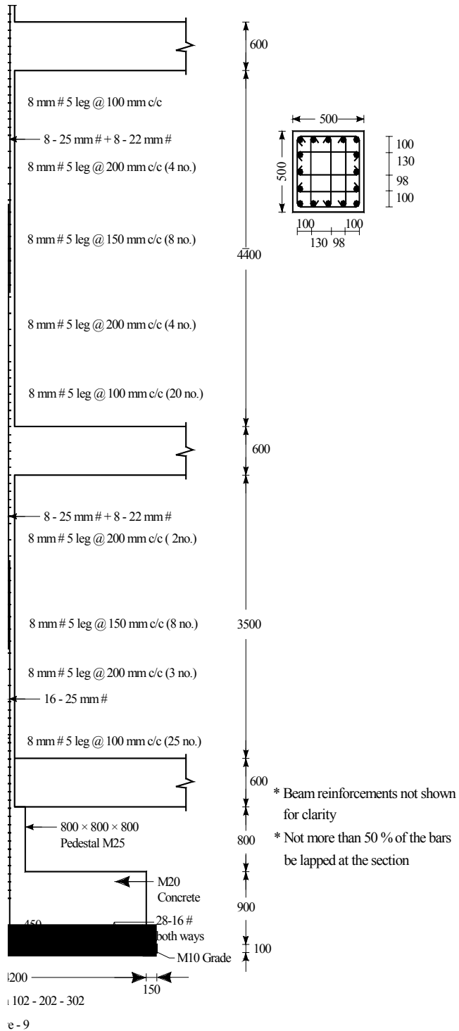
Figure 12 Reinforcement Details
