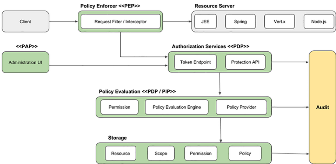
Figure C-2. Keycloak authorization architecture
