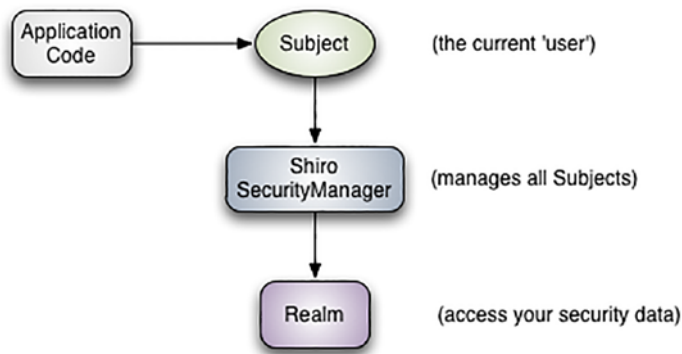
Figure B-1. Shiro concepts
