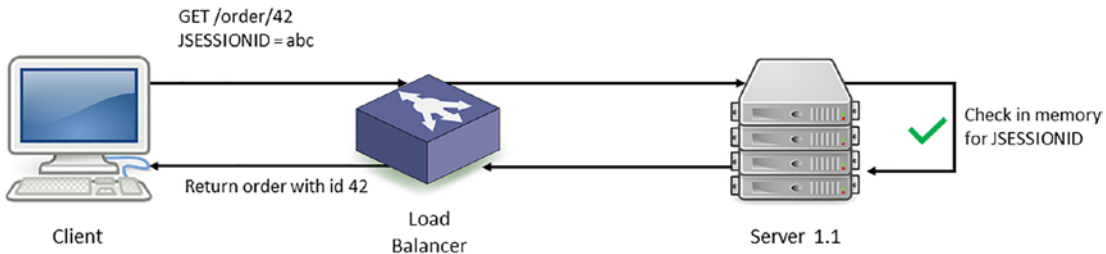
Figure 8-3. Single server behind a load balancer
