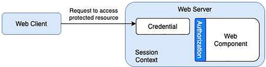
Figure 2-4. URL authorization
