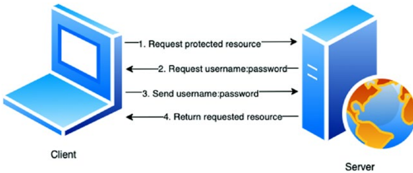
Figure 2-10. Basic authentication
