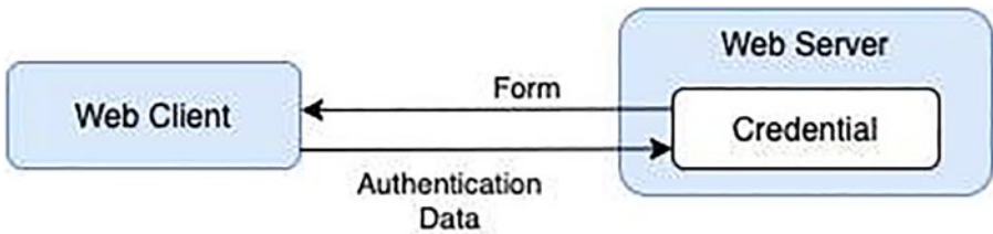
Figure 2-3. Initial authentication
