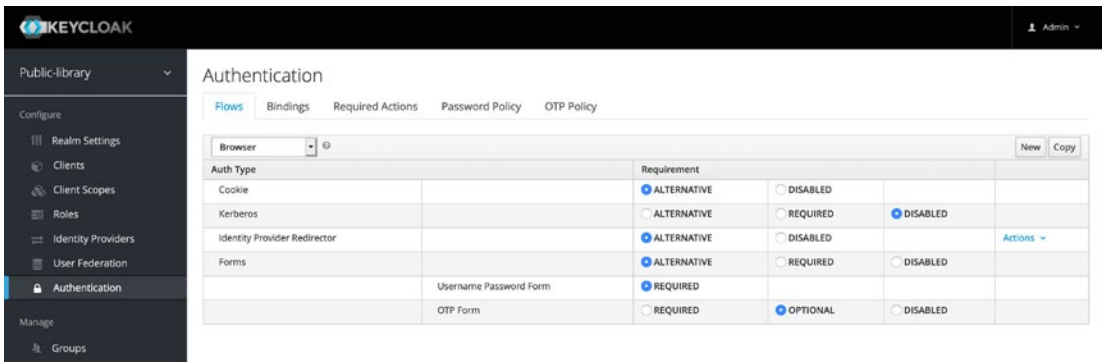
Figure C-1. Browser authentication flows
