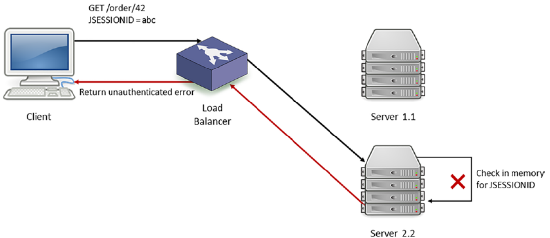
Figure 8-4. New server behind LB, user not recognized
