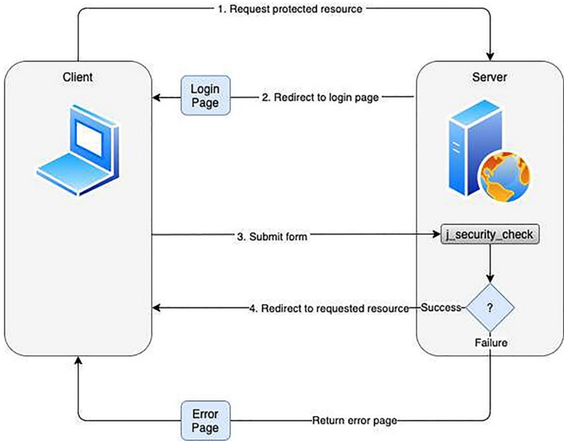
Figure 2-11. Form-based authentication
