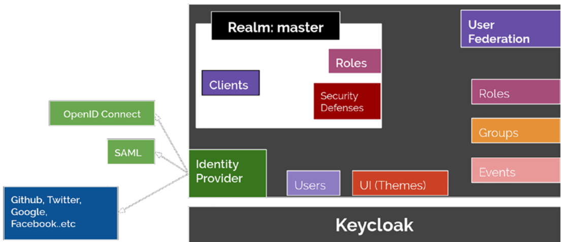
Figure C-3. Keycloak features
