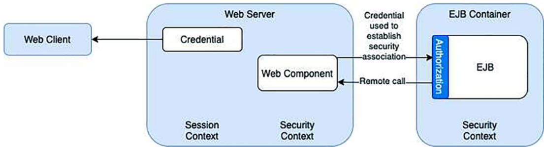
Figure 2-6. Invoking Bean Business Methods
