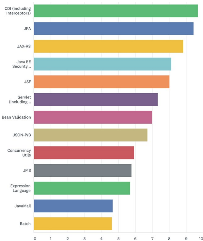
Figure 7-3. APIs most liked to be updated in the next version(s) of Jakarta EE
