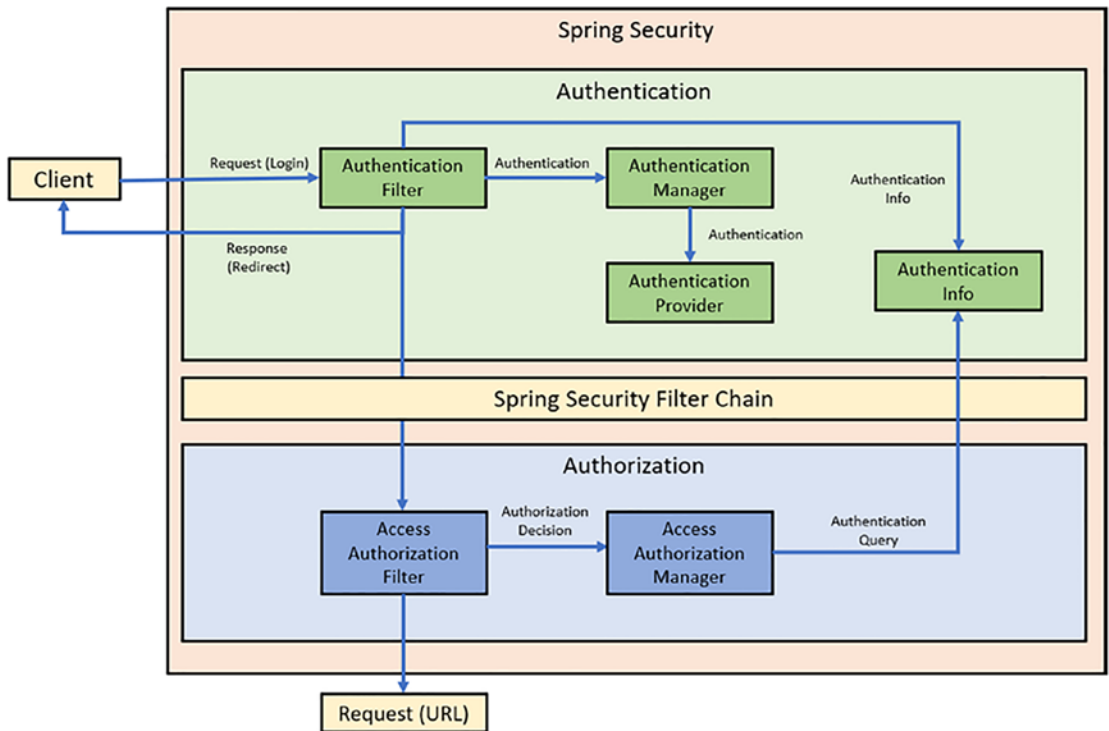
Figure A-1. Spring Security authentication/authorization flow
