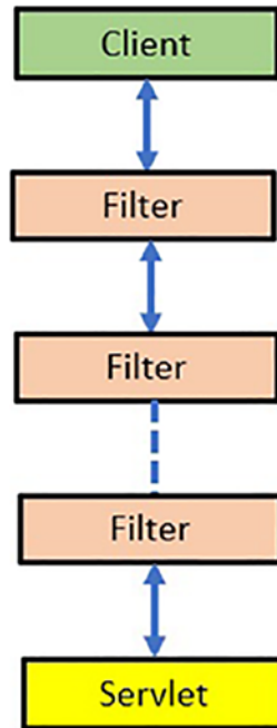
Figure A-3. Filter chain for a single HTTP request
