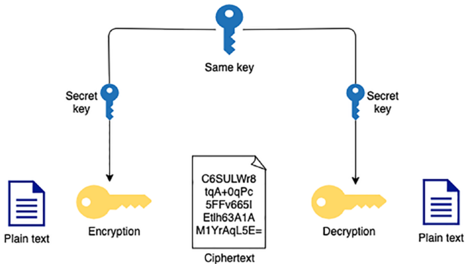
Figure 6-2. Symmetric encryption
