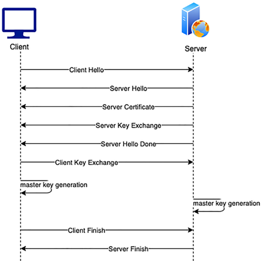
Figure 6-8. TLS Handshake
