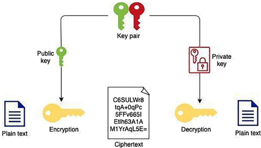
Figure 6-3. Asymmetric encryption
