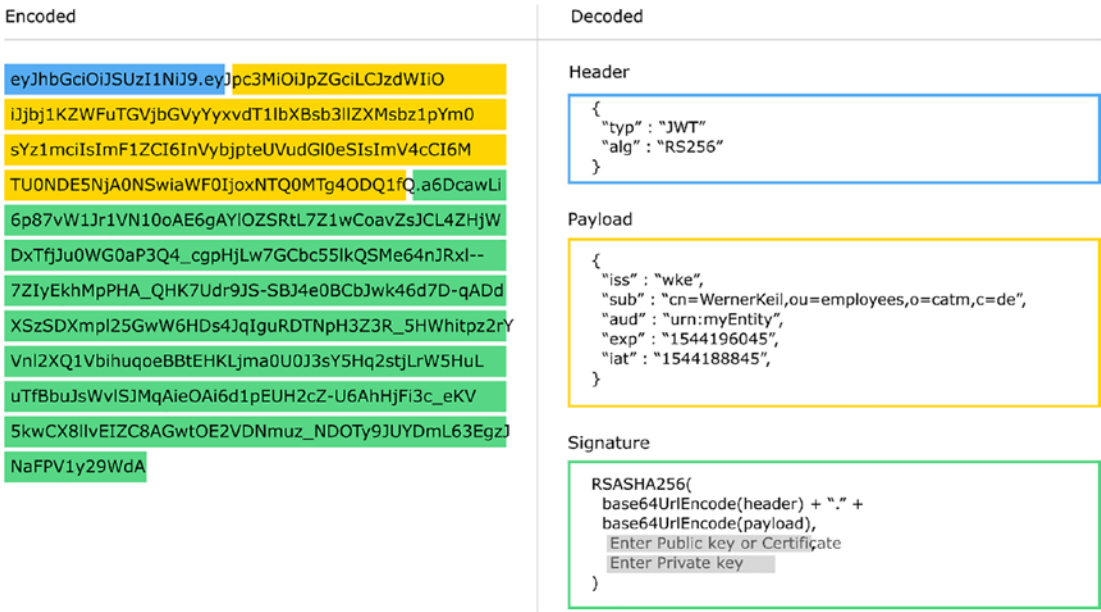
Figure 8-5. JWT structure
