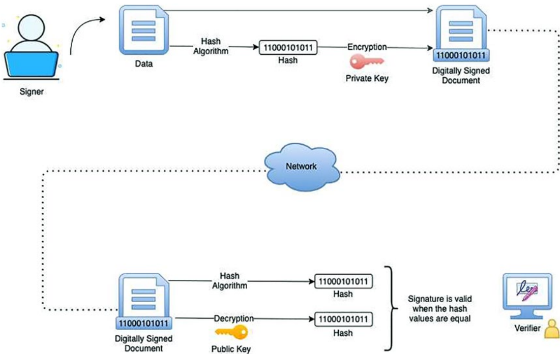
Figure 2-8. Signing process
