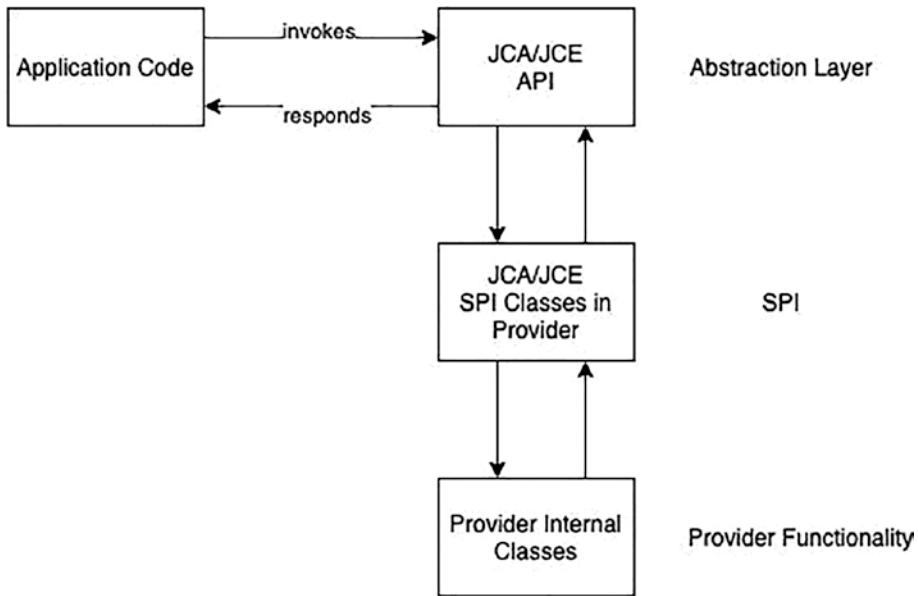
Figure 6-6. JCE providers architecture
