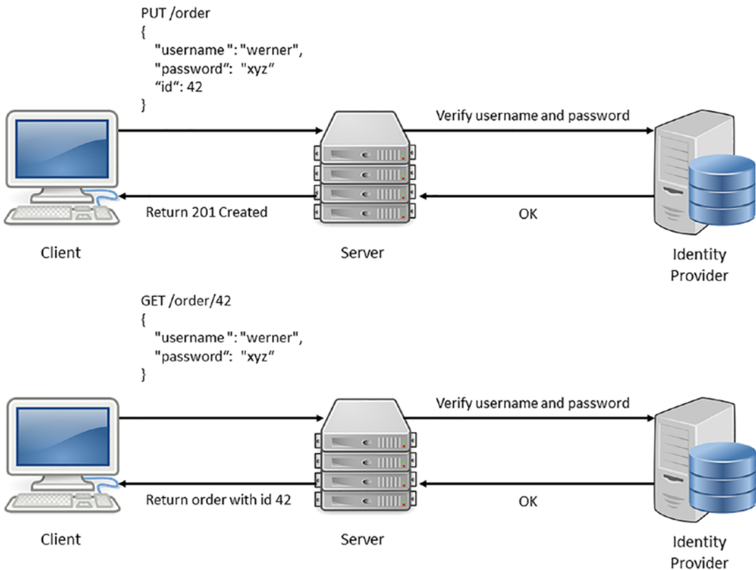
Figure 8-1. Repeating authentication for every new HTTP API request
