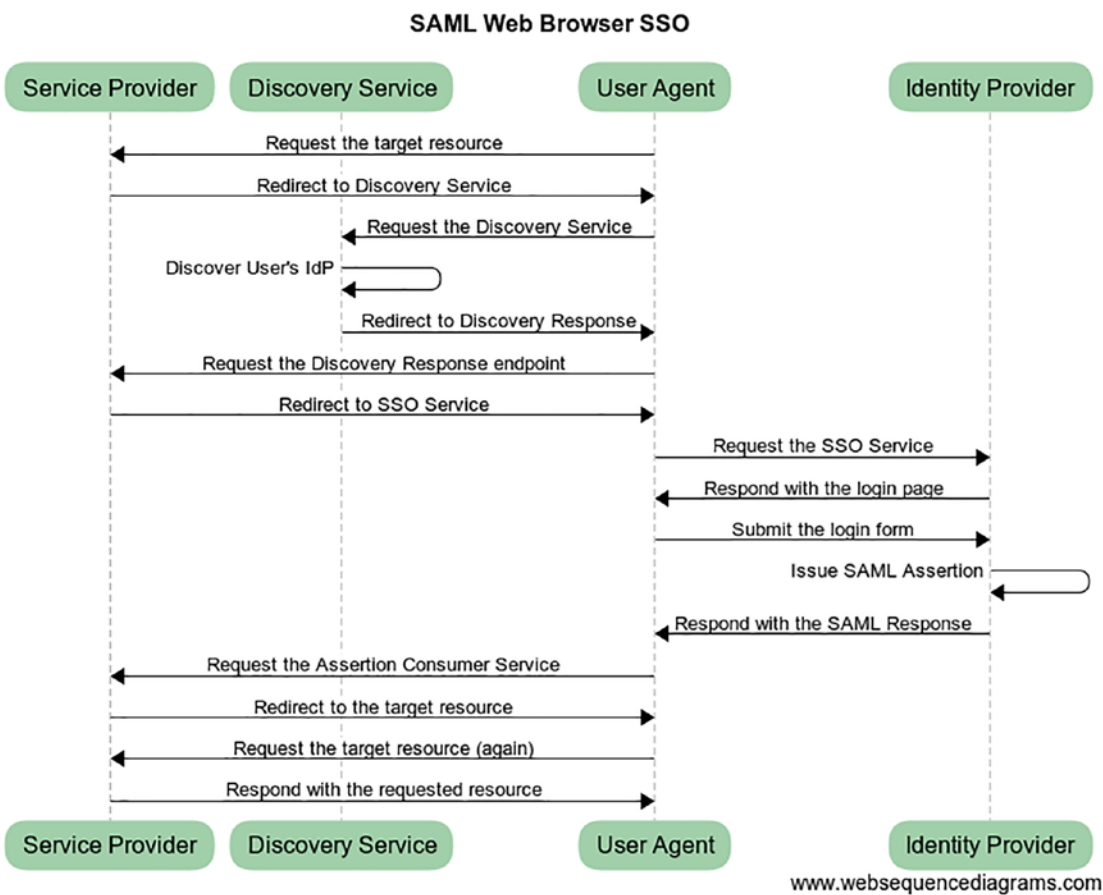
Figure C-5. SAML Web Browser interactions
