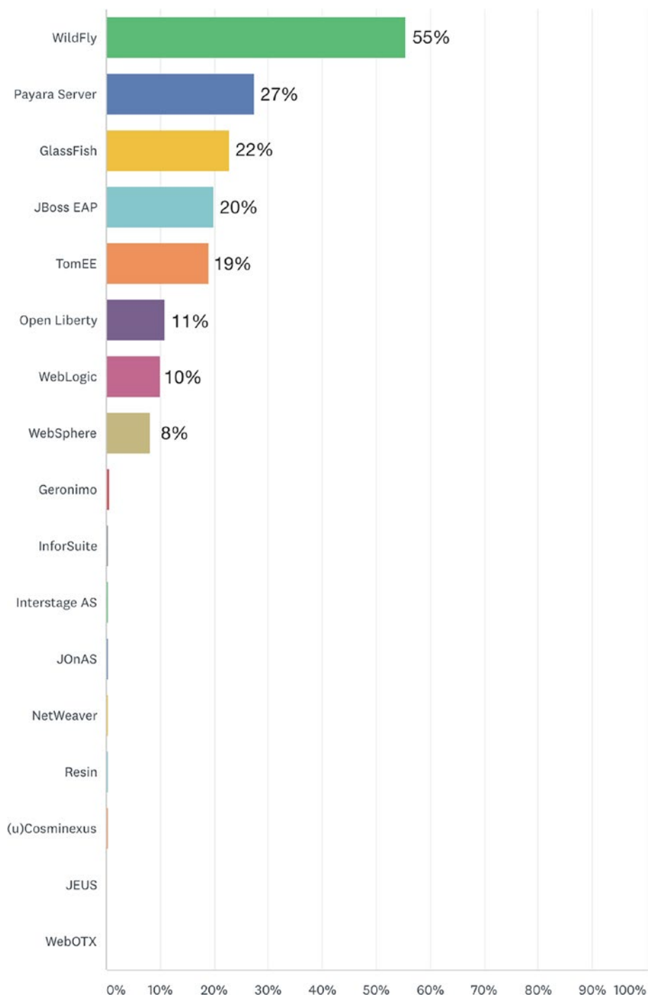
Figure 7-11. Usage of Java EE/Jakarta EE application servers in 2020
