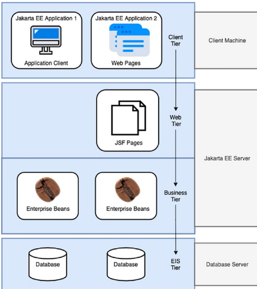
Figure 2-1. Multitiered applications
