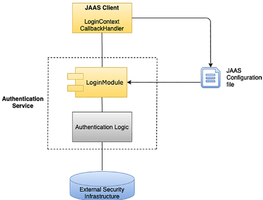
Figure 6-1. JAAS Authentication architecture diagram
