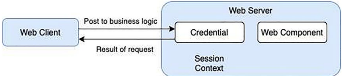
Figure 2-5. Fulfilling the original request
