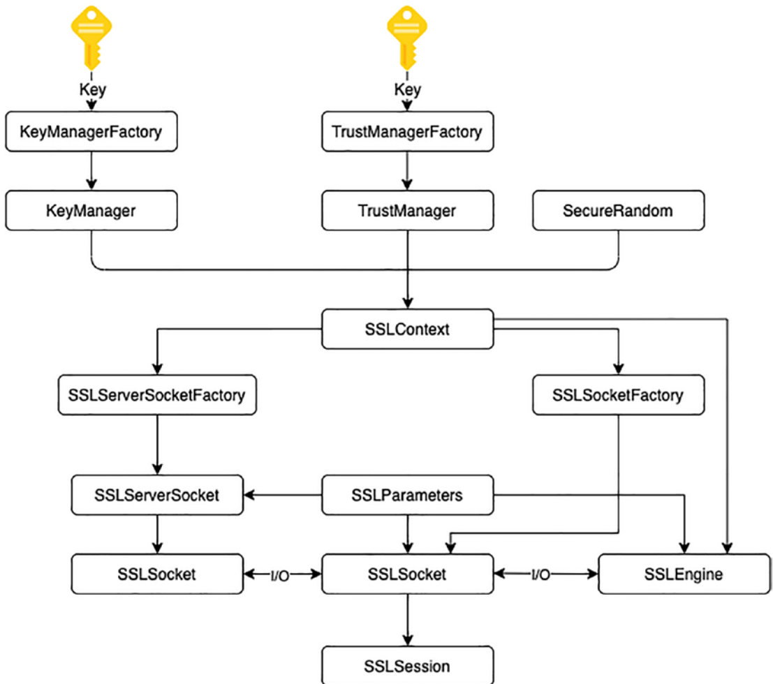
Figure 6-9. JSSE API overview
