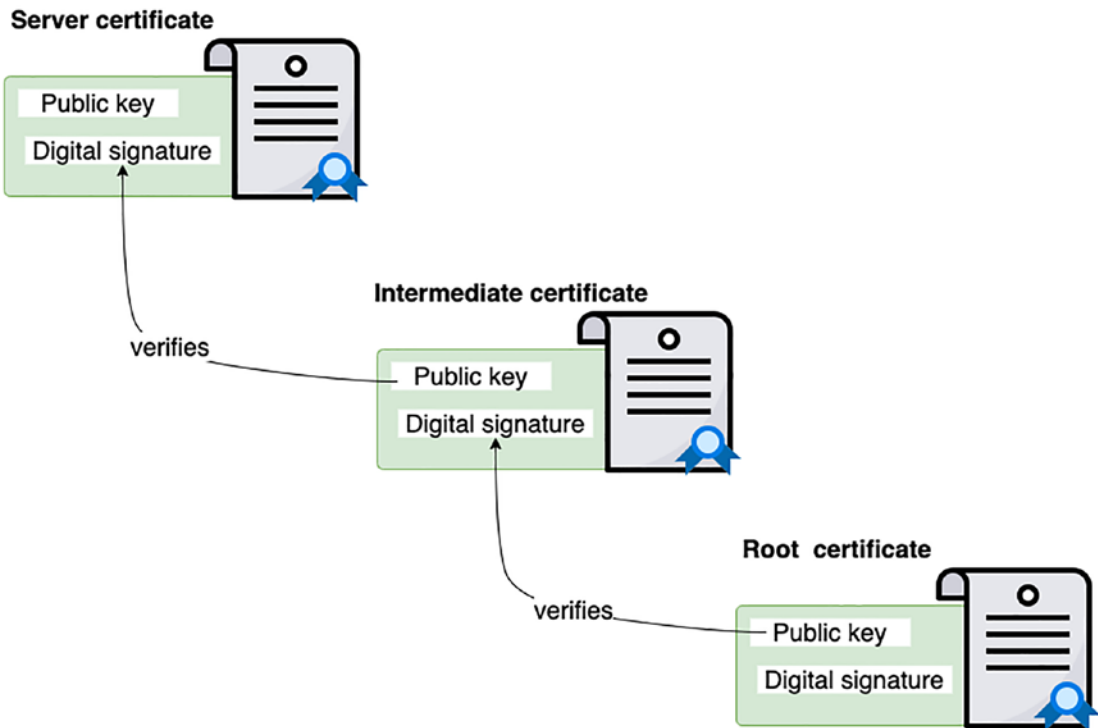
Figure 6-4. Certificate chain for a two-tier CA
