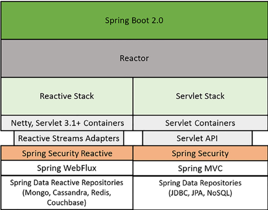
Figure A-5. Spring Security 5 stacks
