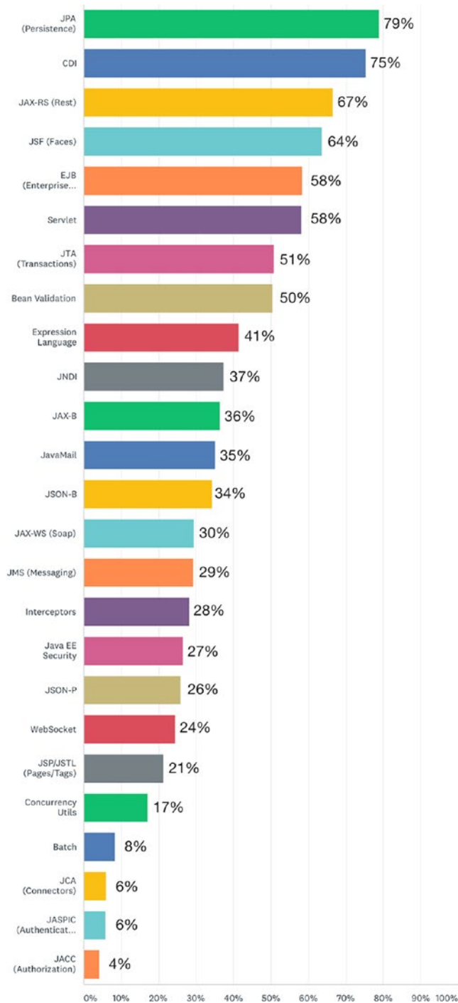
Figure 7-2. Usage of Java EE/Jakarta EE APIs
