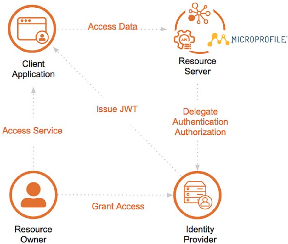
Figure 8-6. Accessing a service protected by MP-JWT
