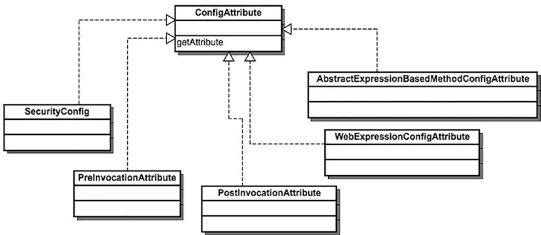
Figure A-2. Config Attribute hierarchy
