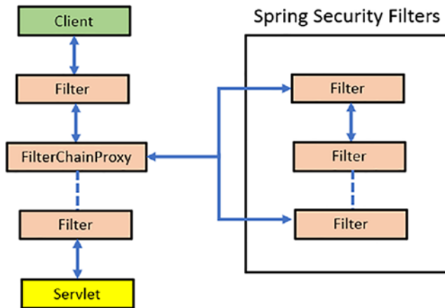
Figure A-4. Filter chain proxy
