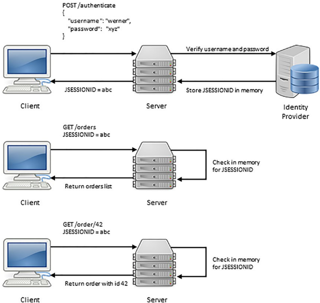
Figure 8-2. Using SSS, reducing the number of authentications against the Identity Provider
