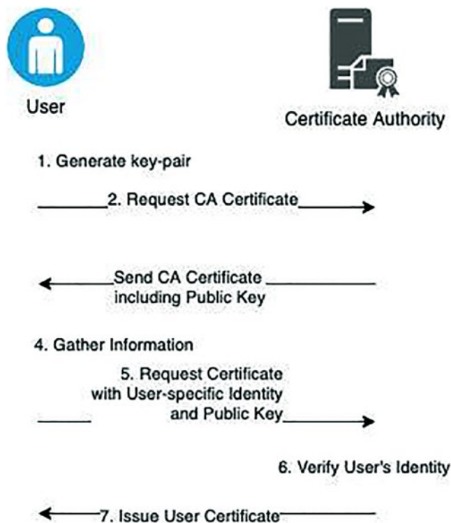
Figure 2-9. Requesting a certificate from a CA
