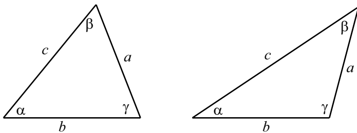
Figure 3.15: General Triangles
