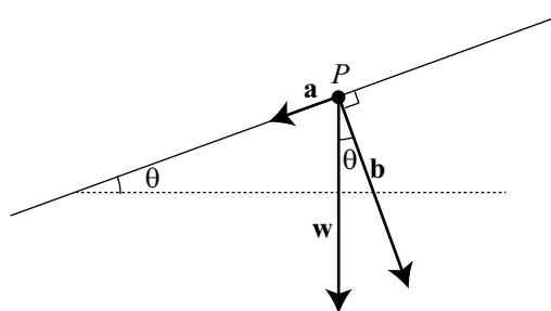
Figure 3.20: Inclined Plane
