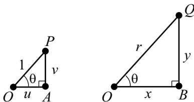
Figure 3.3: Similar Triangles from Figure 3.2
