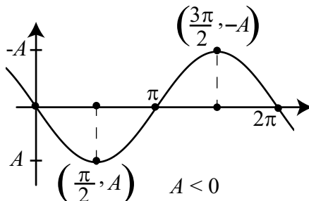
Figure 2.7: Graphs of y = A \sin(t) .
