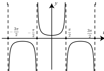
Figure 2.29: Graph of y = \sec(t)
