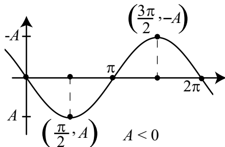
Figure 2.3: Graphs of y = A \sin(t) .
