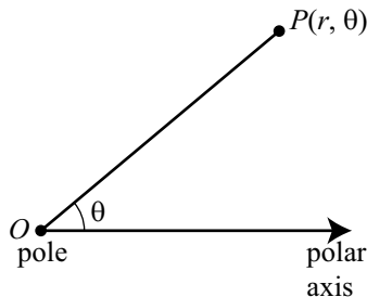
Figure 5.5: Polar Coordinates
