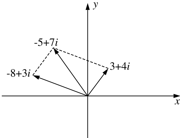
Figure 5.2: The Sum of Two Complex Numbers.
