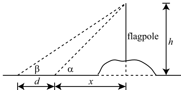
Figure 3.11: Flagpole on a hill
