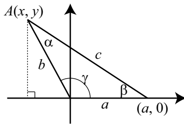
Figure 3.17: Diagram for the Law of Cosines
