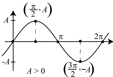
Figure 2.3: Graphs of y = A \sin(t) .
