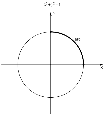
Figure 1.5: An arc on the unit circle
