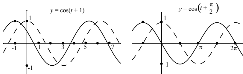
Figure 2.14: Graphs of y = \cos(t + 1) and y = \cos\left(t + \frac{\pi}{2}\right) . The graph of y = \cos(t) is also shown (dashes).
