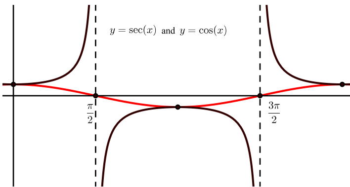
Figure 2.27: Graph of One Period of y = \sec(x) with 0 \leq x \leq 2\pi
