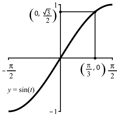
Figure 2.34: Graphical Version of \arcsin\left(\frac{\sqrt{3}}{2}\right) = \frac{\pi}{3}
