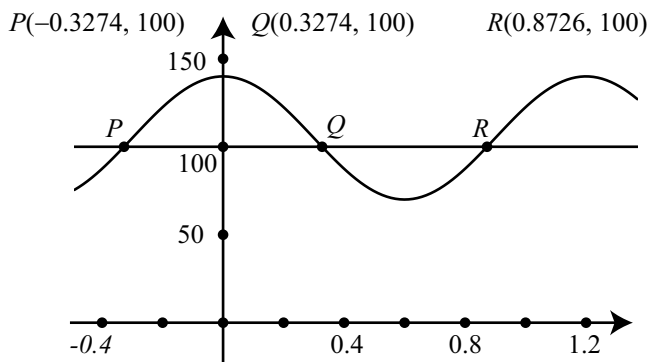
Figure 2.20: Graph of V(t) = 35 \cos\left(\frac{5\pi}{3}t\right) + 105 and y = 100
