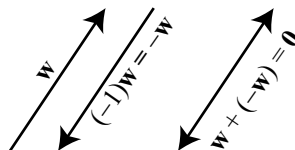
Figure 3.22: The Sum of a Vector and Its Negative
