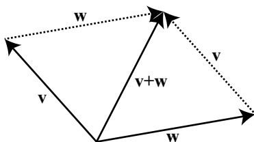
Figure 3.21: Sum of Two Vectors Using a Parallelogram
