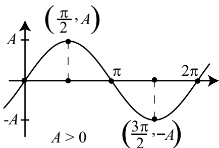
Figure 2.7: Graphs of y = A \sin(t) .
