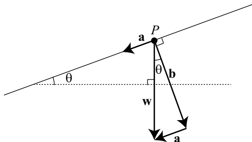
Figure 3.26: Inclined Plane
