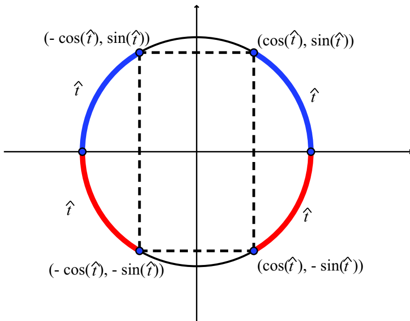
Figure 1.22: Reference arcs.
