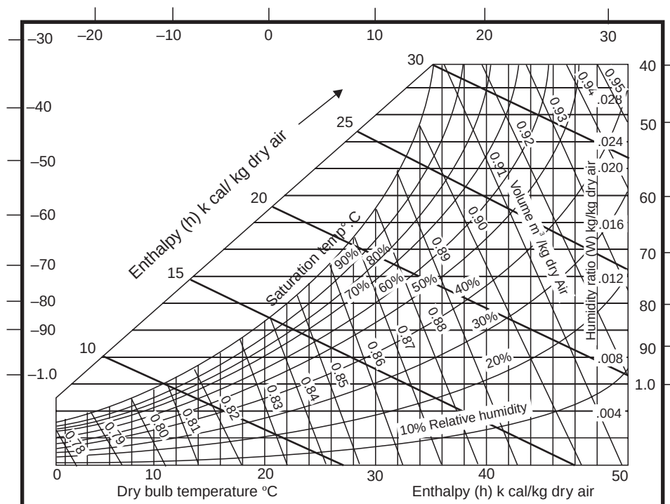
Fig. 10.5. Carrier chart.
