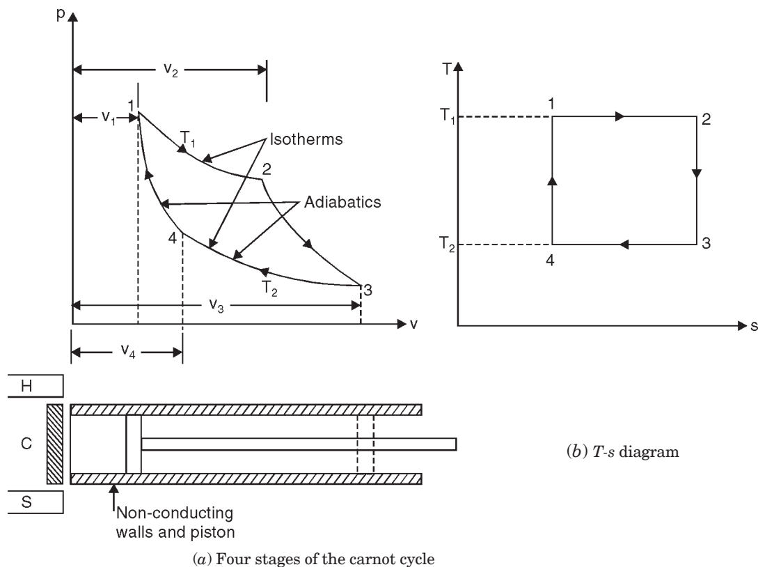
Fig. 13.1. Carnot cycle.
