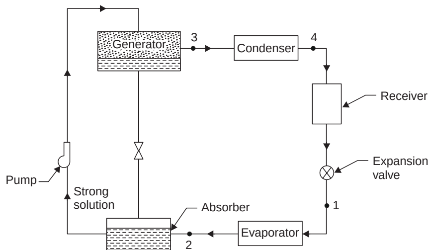
Fig. 14.21. (a) Simple vapour absorption system.
