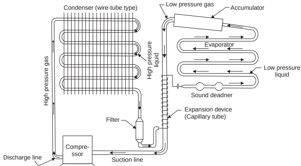
Fig. 1.9. Domestic refrigerator.
