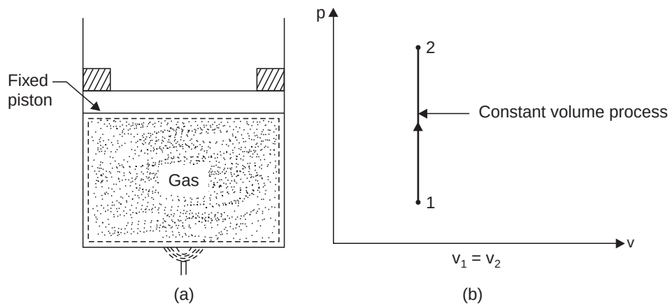
Fig. 4.5. Reversible constant volume process.
