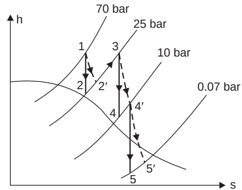
(c) h-s diagram (Pump work not shown)
