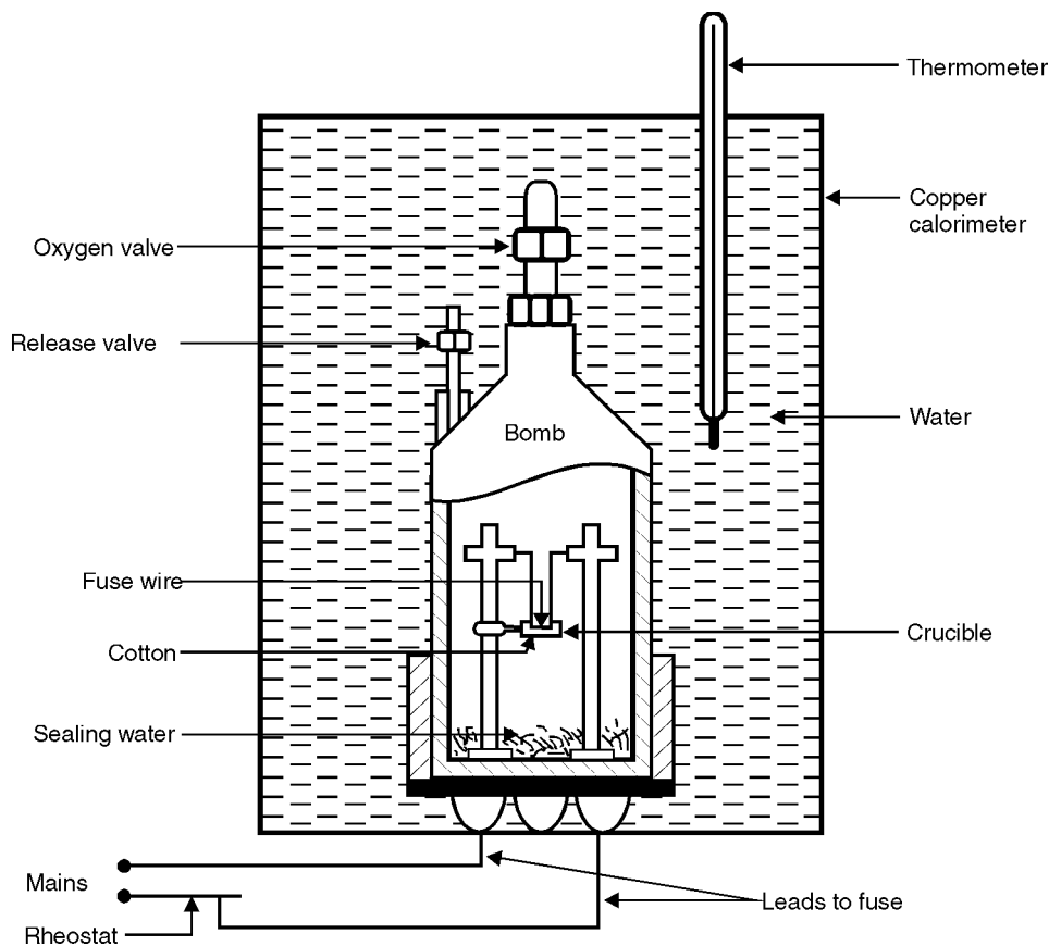
Fig. 11.5. Bomb calorimeter.
