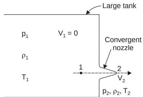
Fig. 16.8. Flow of fluid through a convergent nozzle.
