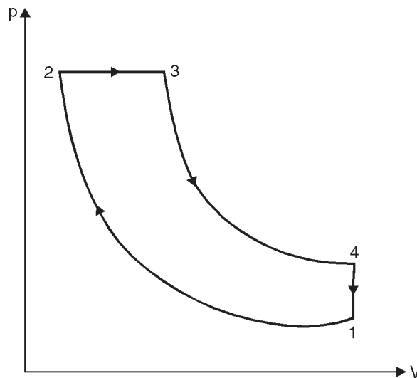
Fig. 13.18. Diesel cycle.
