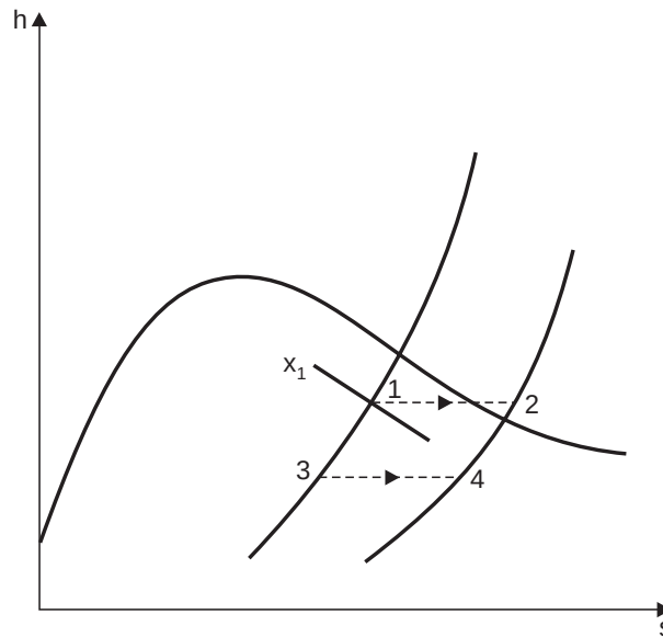
Fig. 3.16. Throttling process.
