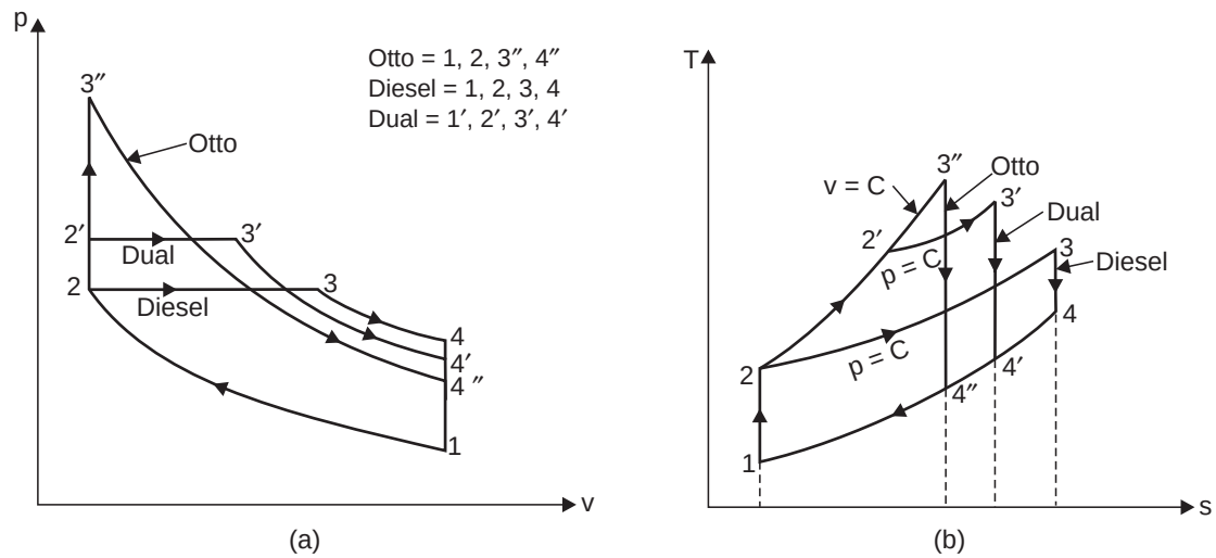
Fig. 13.27. (a) p-v diagram, (b) T-s diagram.
