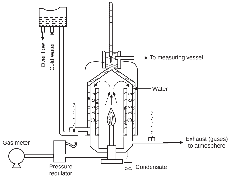
Fig. 11.6. Junker's gas calorimeter.
