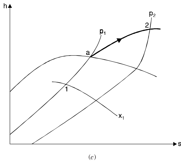
Fig. 4.62. Constant temperature or isothermal expansion.
