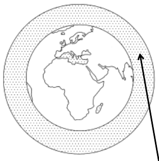
Fig. 10.3 The atmosphere
