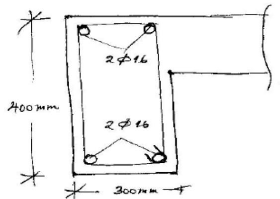
Sec 2-2.
