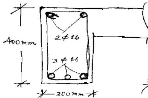
Sec 1-1.
