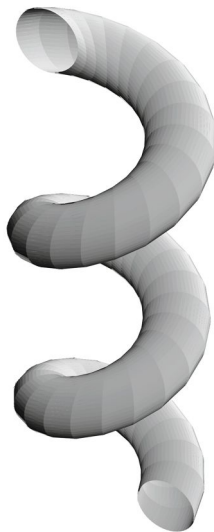
The tube around a circular helix
