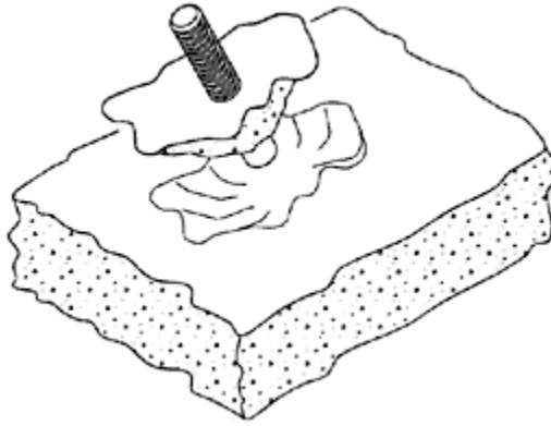
Figure 6-16 Concrete Failure by Tension, Insufficient Embedment Depth
