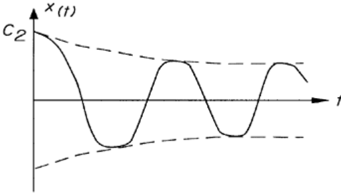
Figure 8-3 Forced Vibration of Single Degree of Freedom
