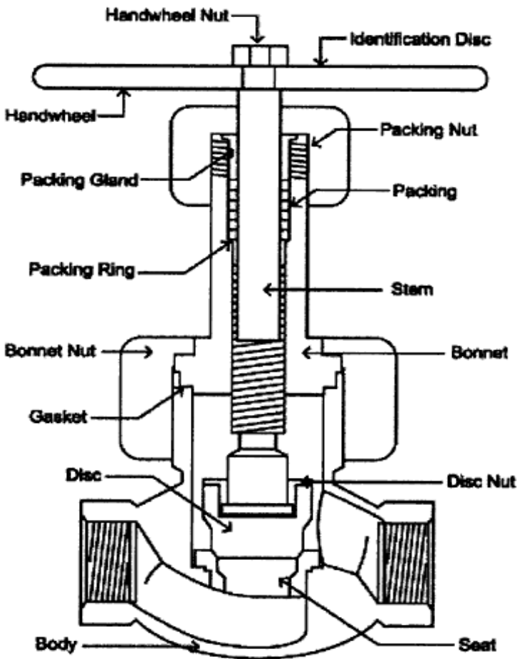
Figure 25-2 Globe Valve
