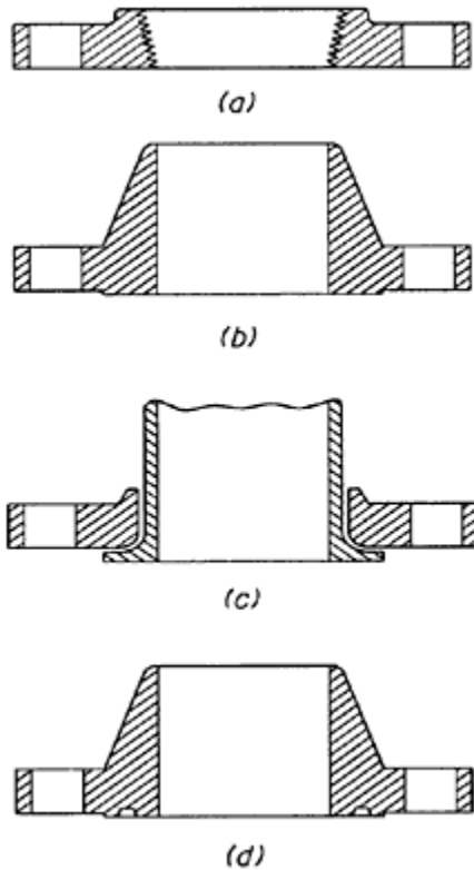
Figure 17-3 Typical Flange Faces
