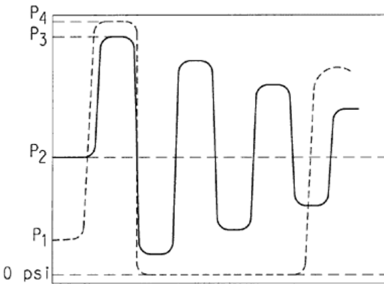
Figure 9-5 Pressure Trace During a Waterhammer
