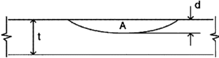
Figure 21-3 Parameters for B31G Evaluation
