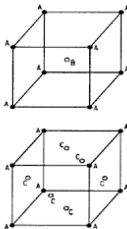
Figure 3-6 Atomic Structure of Carbon Steel
