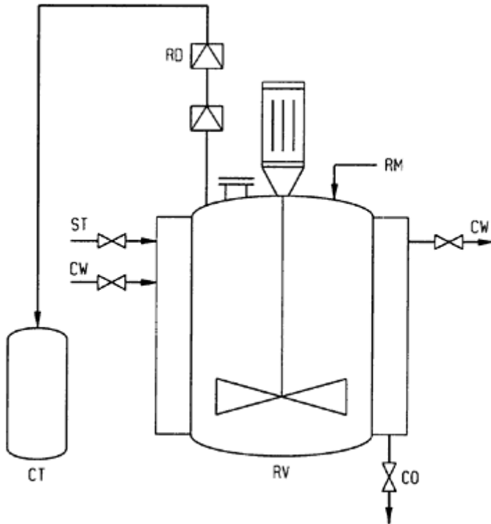
Figure 4-12 Simplified Diagram of Dye Manufacture Vessel
