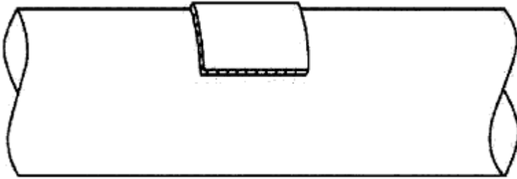
Figure 23-8 Fillet Welded Patch
