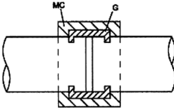
Figure 18-3 Grooved Fitting
