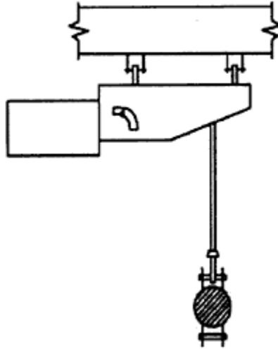
Figure 6-5 Constant Load Hanger
