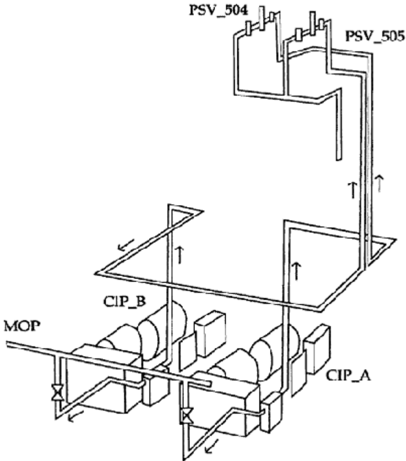
Figure 17-4 Simplified Schematic of Condensate Injection Pumps
