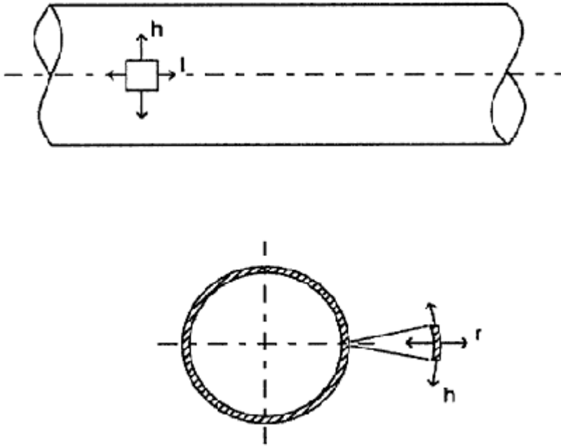
Figure 4-1 Hoop (h), Longitudinal (l) and Radial (r) Stress Directions
