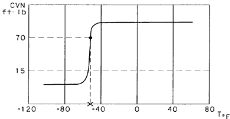
Figure 3-11 Variation of Charpy Toughness with Temperature—Example
