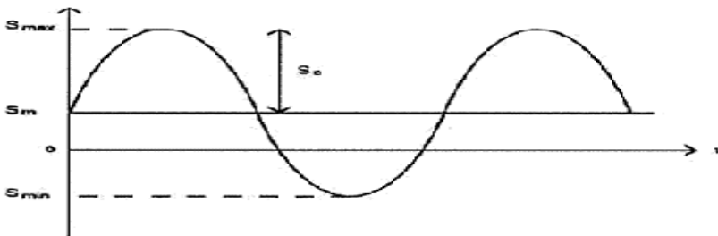
Figure 7-6 Stress Amplitude S_a and Mean Stress S_m
