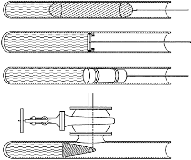
Figure 19-4 Line Isolation Techniques
