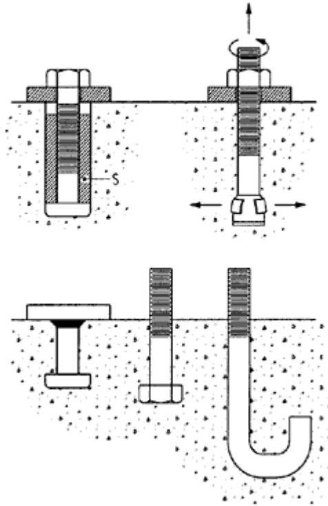
Figure 6-15 Types of Concrete Anchor Bolts
