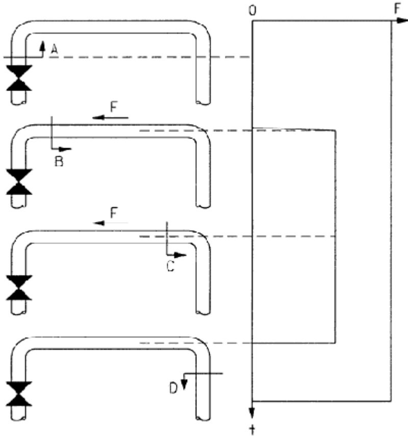
Figure 9-3 Waterhammer Force Imbalance F Between Elbows
