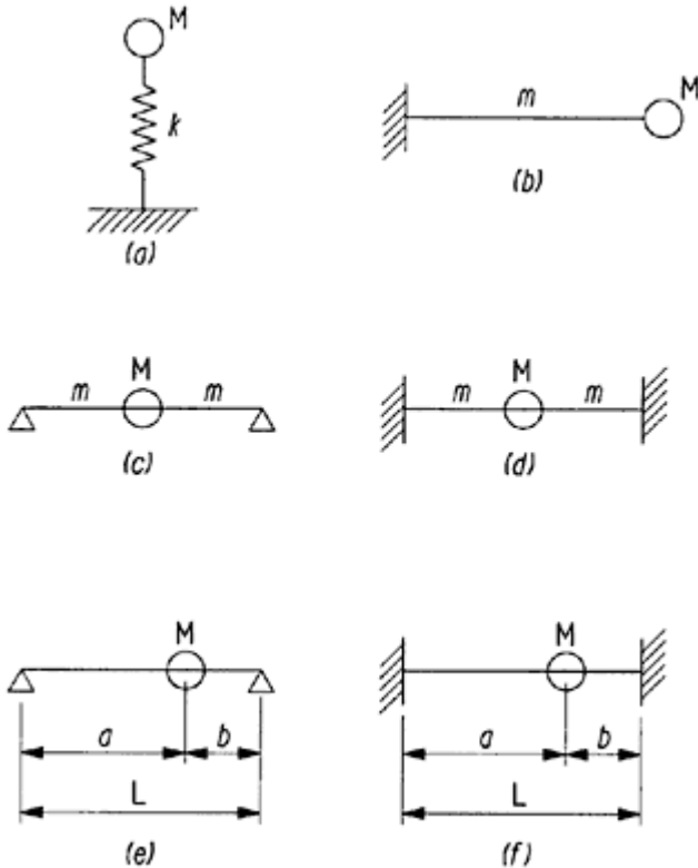
Figure 8-6 Natural Frequency Models
