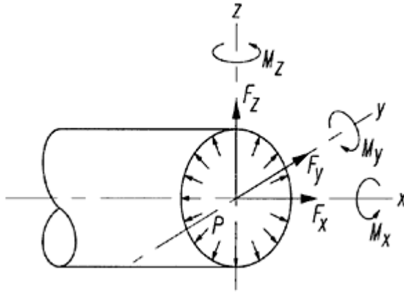
Figure 6-2 Force and Moment Directions
