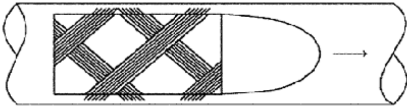
Figure 16-6 Foam Pig
