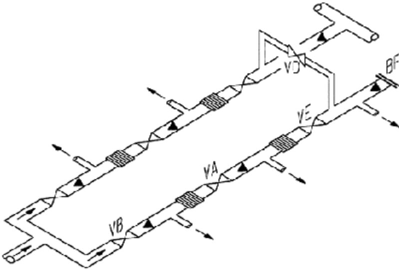
Figure 9-6 Steam System Layout, First Case Study
