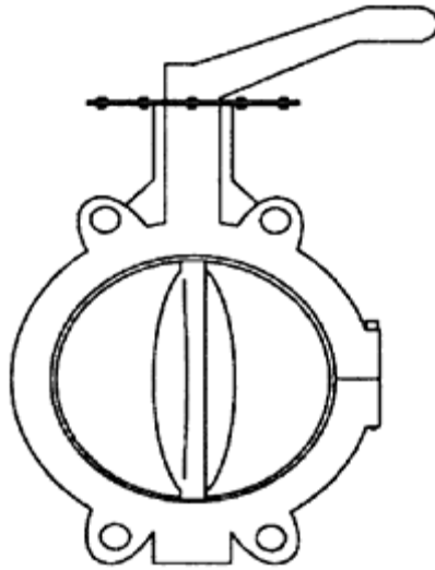
Figure 25-5 Butterfly Valve
