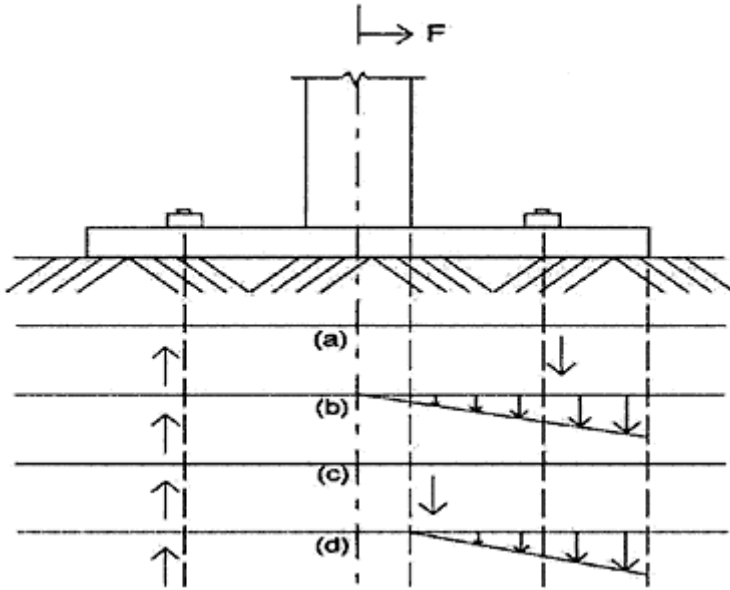
Figure 6-14 Distribution of Compressive Force on Concrete
