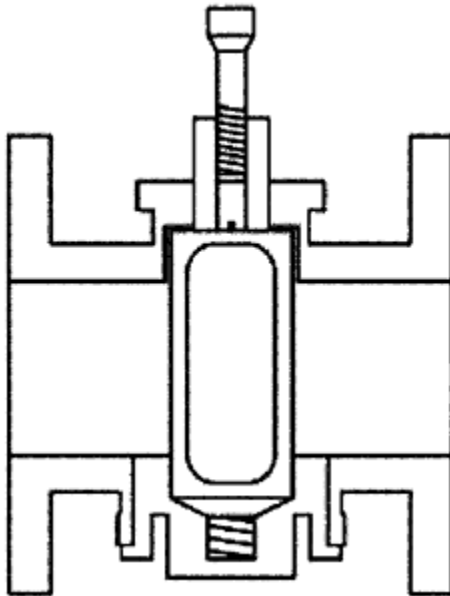
Figure 25-3 Plug Valve
