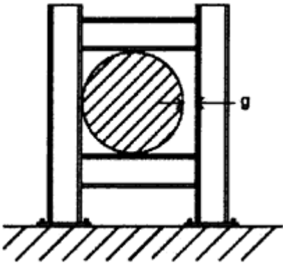
Figure 6-6 Steel Frame with a Lateral Gap
