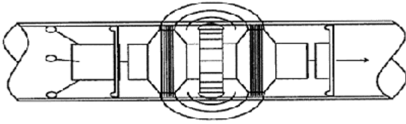
Figure 16-9 Magnetic Flux Leakage Pig
