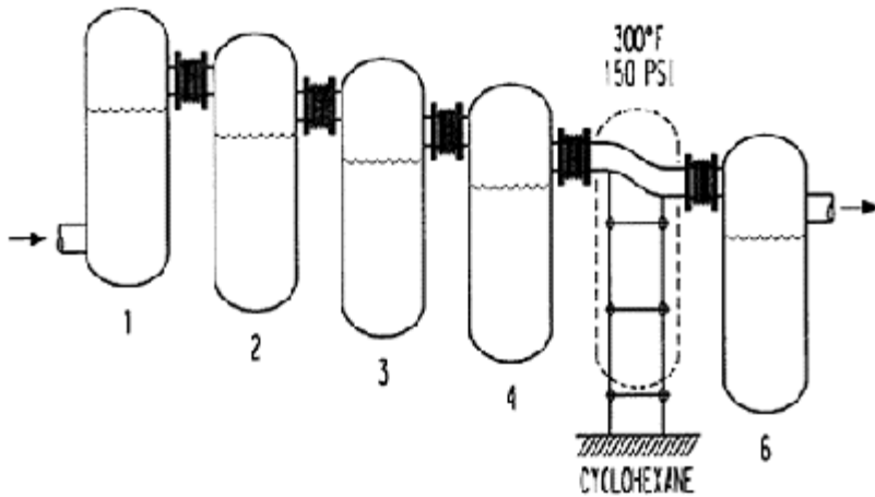
Figure 7-13 Simplified Vessel and Bellows Arrangement
