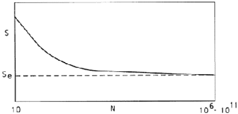
Figure 7-5 Form of the S (Stress Amplitude) -N (Cycles) Fatigue Curve
