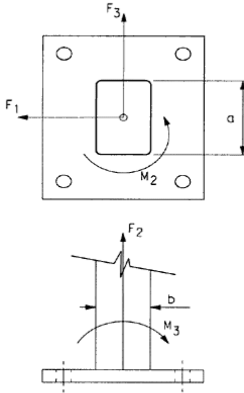
Figure 6-13 Base Plate Example
