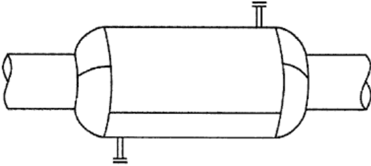
Figure 23-10 Welded Leak Box
