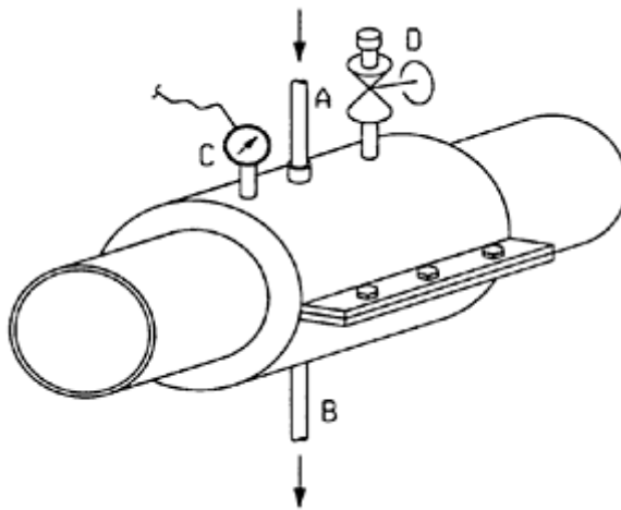
Figure 19-5 Freeze Plug Arrangement.
