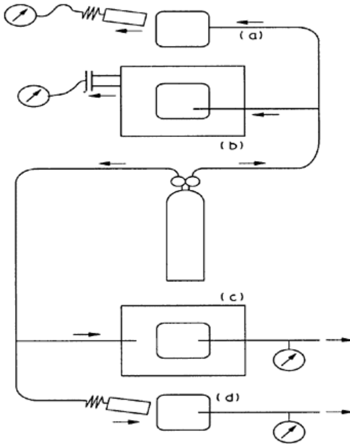
Figure 19-2 Sensitive Leak Test Arrangements
