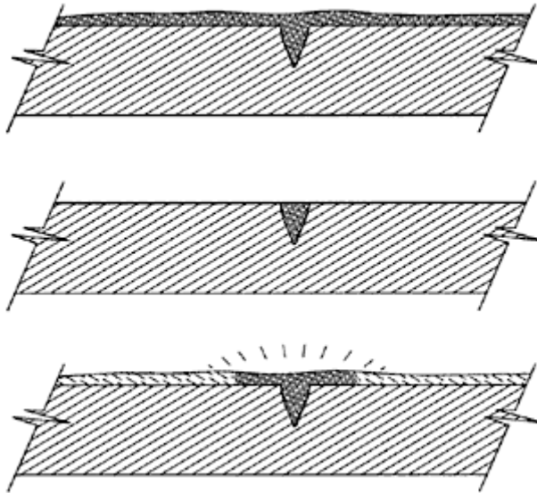
Figure 16-2 Liquid Penetrant Testing
