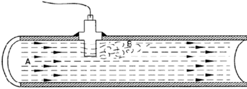
Figure 8-7 Vortex Shedding around Obstruction
