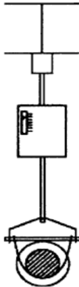
Figure 6-3 Variable Spring Hanger
