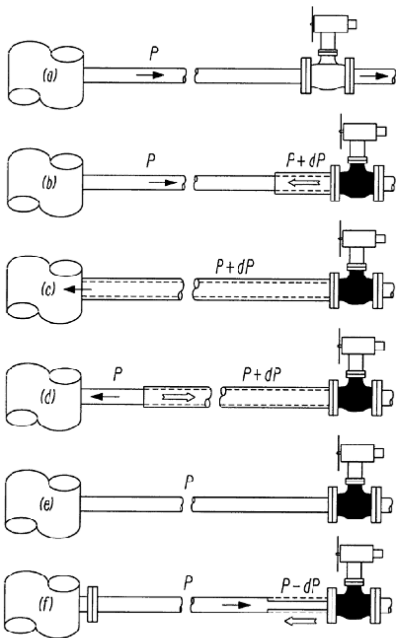
Figure 9-2 Travel of Pressure Wave
