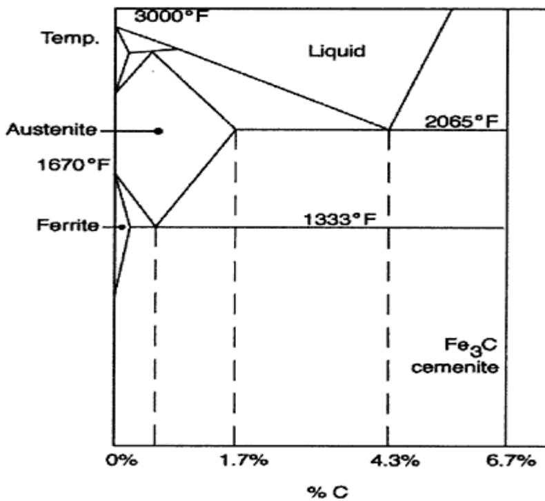
Figure 3-5 Simplified Phase Diagram of Carbon Steel
