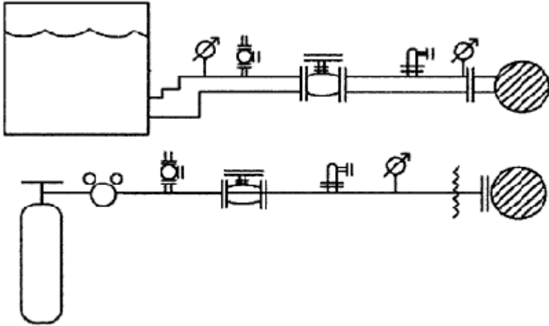
Figure 19-3 Hydrostatic (top) and Pneumatic (bottom) Test Arrangements.
