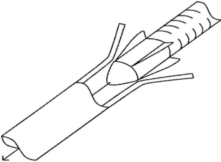
Figure 23-15 Pipe Splitting with Polyethylene Pipe Follower
