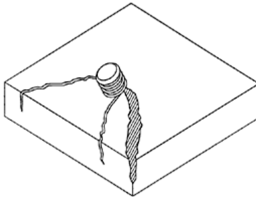
Figure 6-17 Concrete Failure, Insufficient Edge Distance
