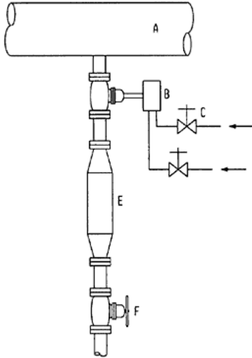
Figure 23-1 Settling Leg Arrangement
