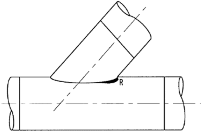
Figure 4-5 Burst of 30° Intersection at R [Sang]
