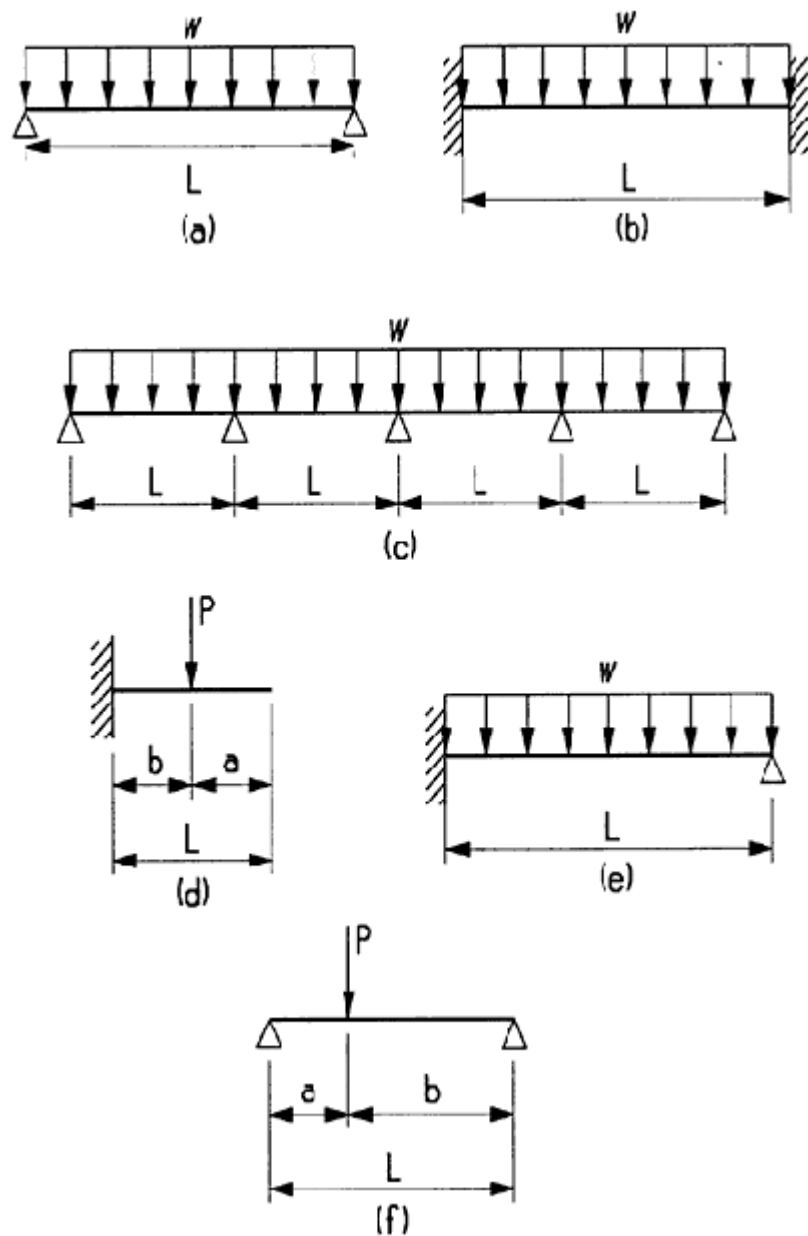
Figure 6-1 Simplified Pipe Spans
