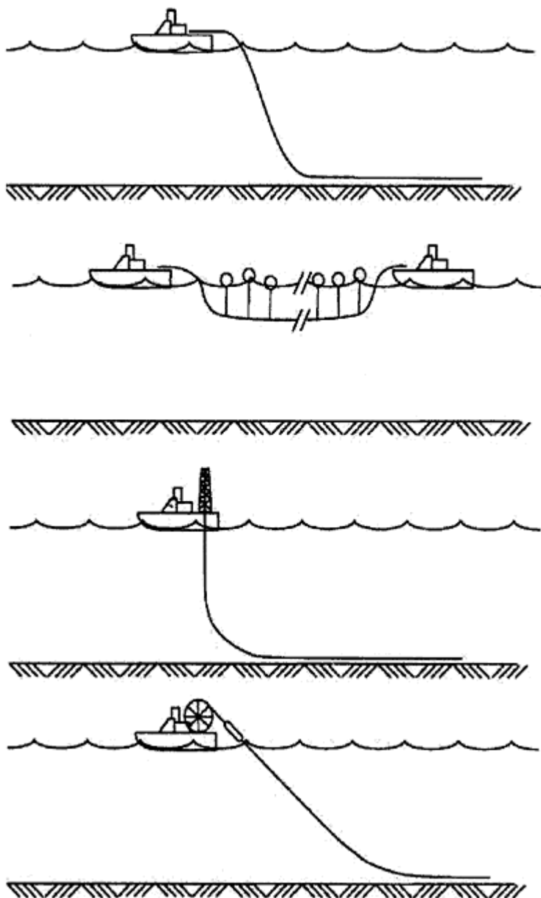
Figure 13-1 Methods for Lowering Pipelines to the Seabed
