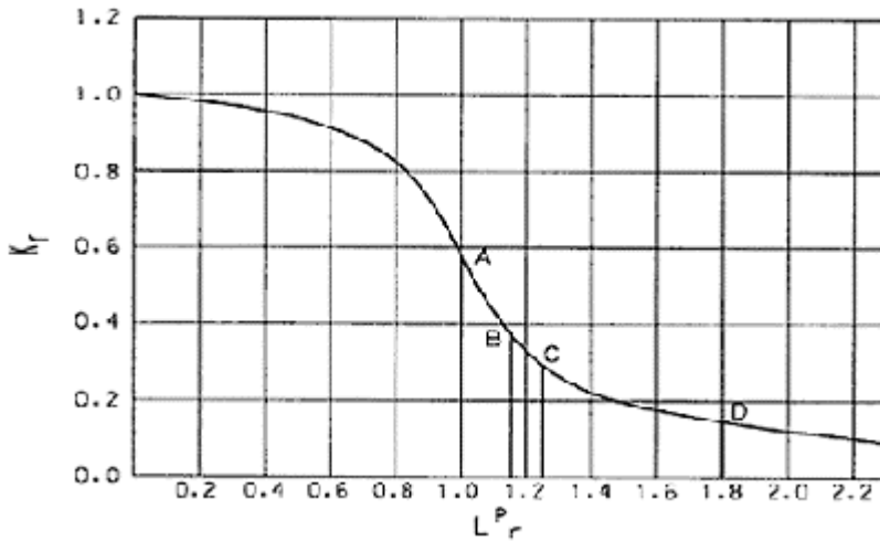
Figure 21-9 Failure Assessment Diagram (FAD)
