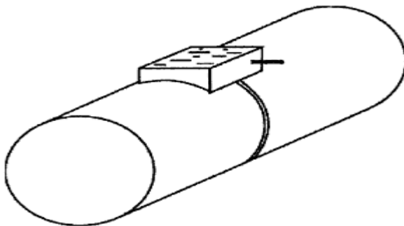
Figure 19-1 Leak Box Test Arrangement
