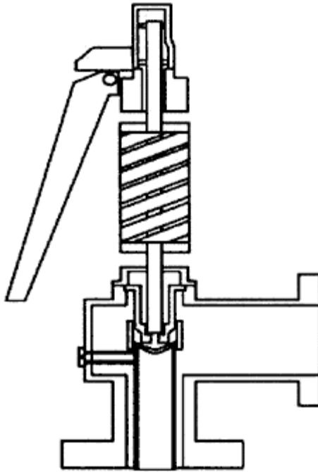
Figure 25-7 Spring Loaded Relief Valve
