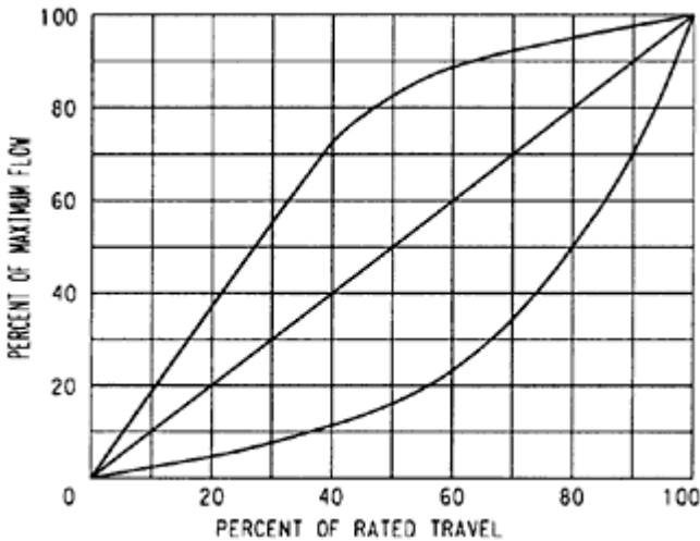
Figure 9-4 Typical valve Characteristics
