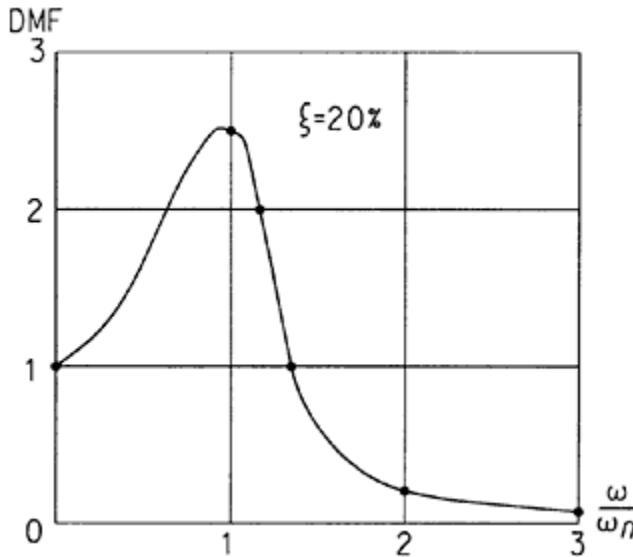
Figure 8-4 Resonant Response
