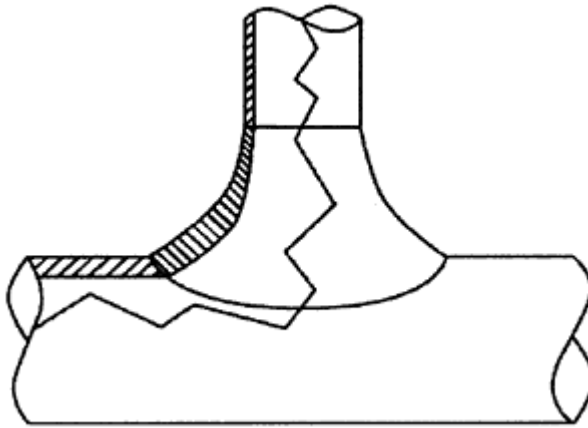
Figure 4-8 Integrally Reinforced Outlet Fitting
