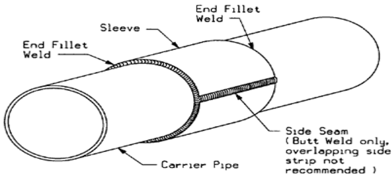
Figure 23-7 Full Encirclement Split Sleeve, with Circumferential Weld
