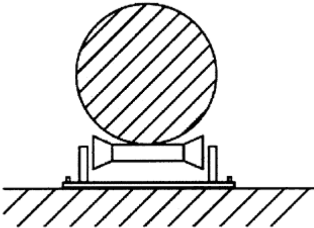
Figure 6-8 Pipe Roll
