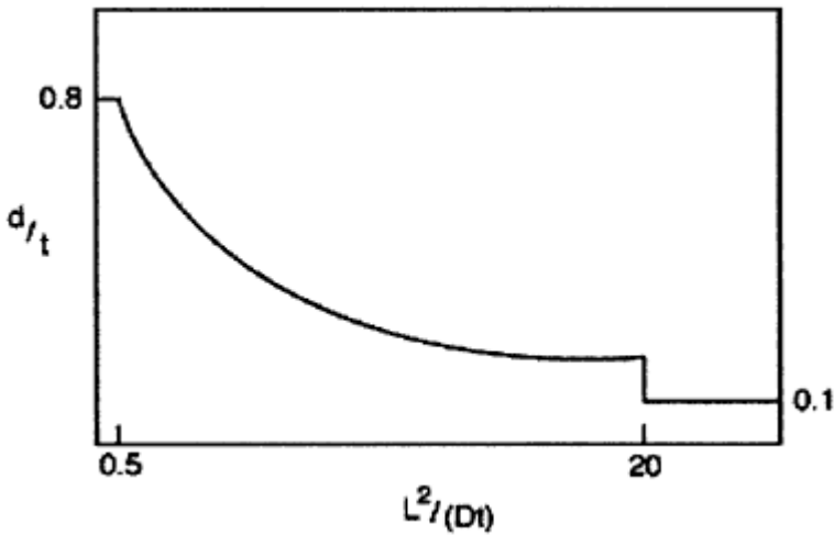
Figure 21-4 ASME B31G Acceptance Curve
