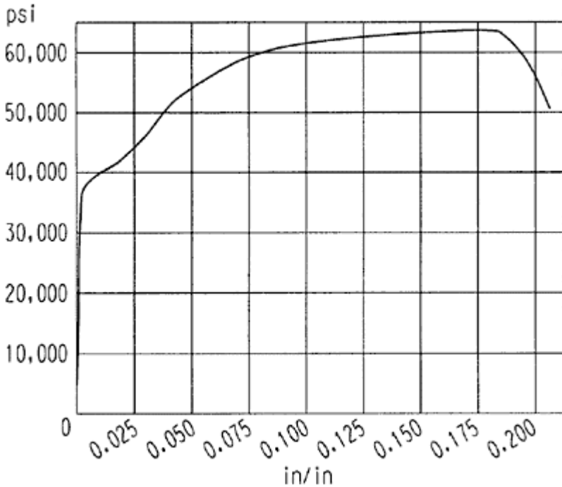
Figure 3-8 An Engineering Stress-Strain Curve for Carbon Steel
