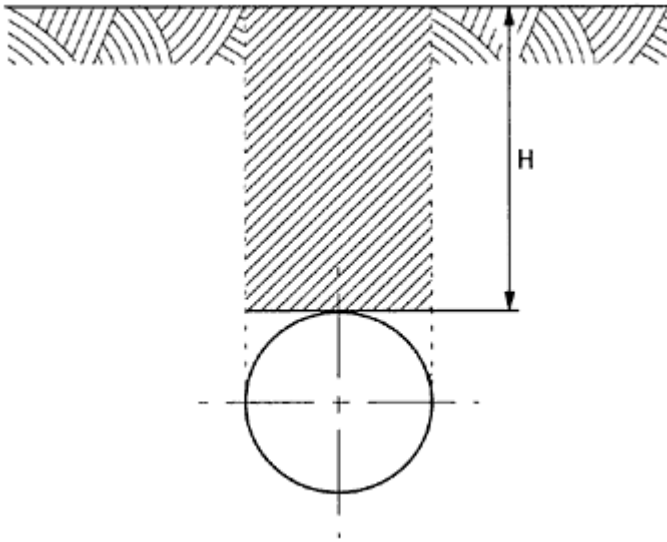
Figure 14-1 Soil Prism Above Pipe
