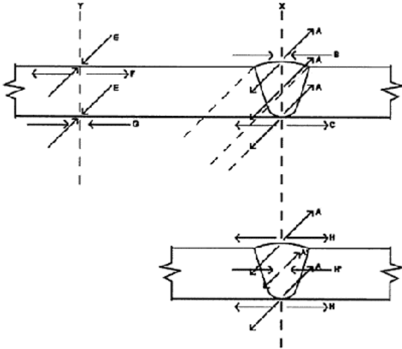
Figure 21-10 Residual Stresses in a Girth Weld
