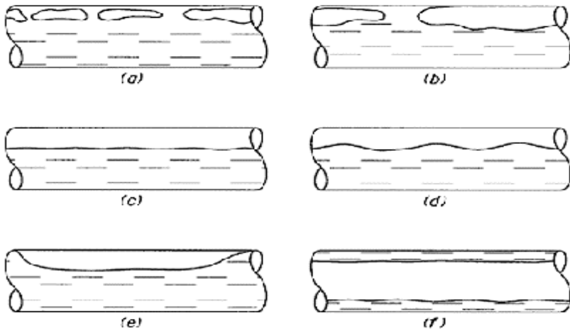
Figure 9-9 Liquid-Gas Flow Regime
