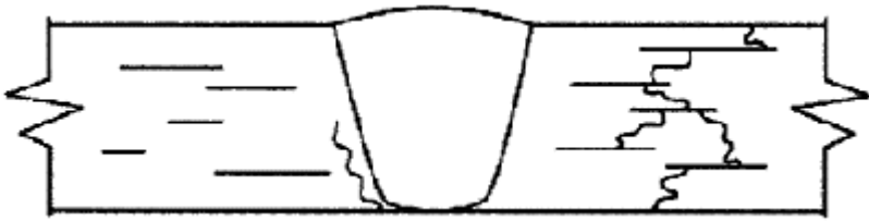
Figure 20-6 HIC (left), SSC (at left of weld root), SOHIC (right)
