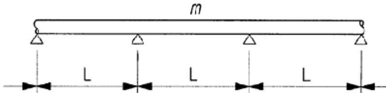
Figure 8-5 Multispan Beam
