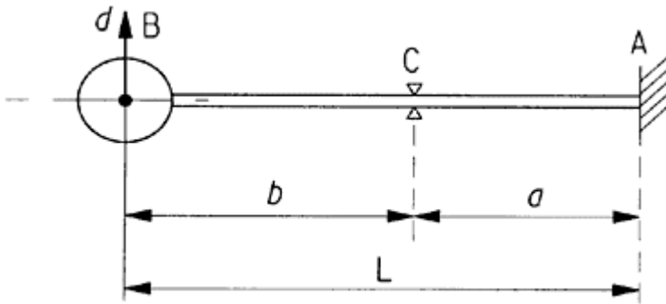
Figure 7-1 Evaluation of Header Movement
