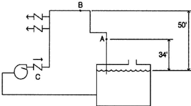
Figure 9-8 Siphon Column Separation
