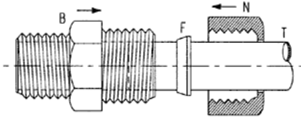
Figure 18-2 Example of a Swage Fitting
