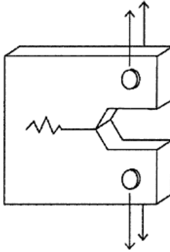
Figure 3-12 Illustration of a KIC Test Specimen
