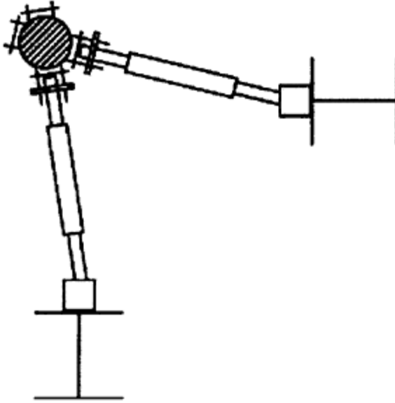
Figure 6-9 Rigid Strut Tandem
