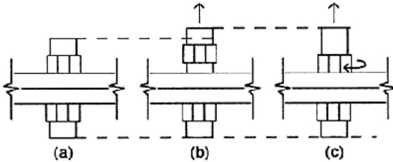
Figure 17-5 Hydraulic Tensioning
