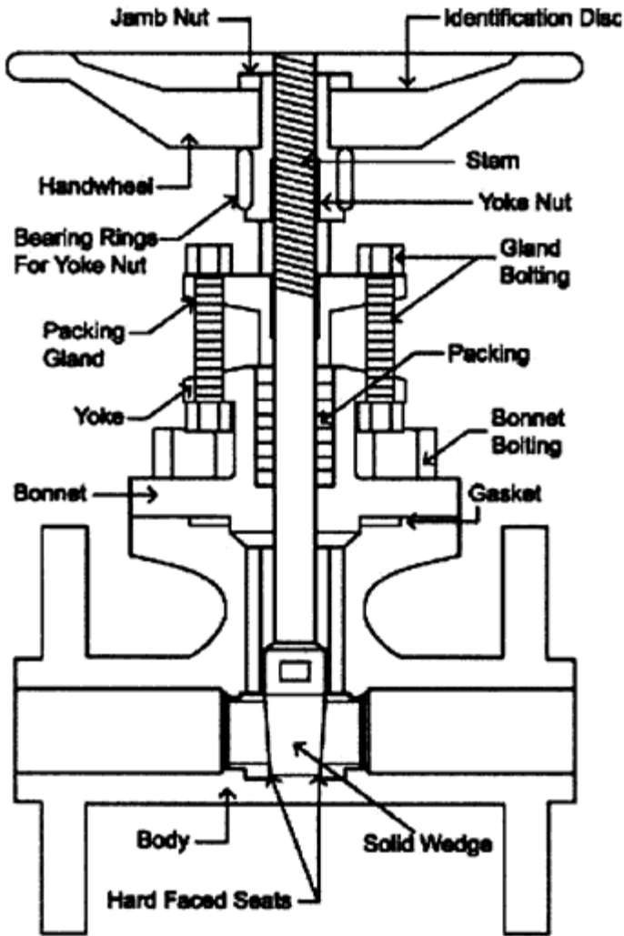
Figure 25-1 Gate Valve, Solid Wedge
