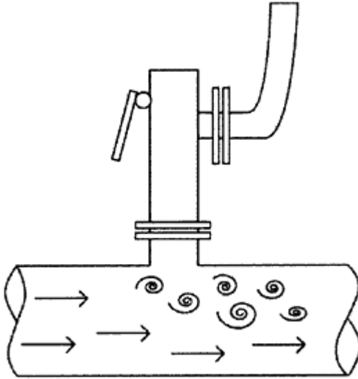
Figure 8-8 Vortex Shedding at Branch Inlet
