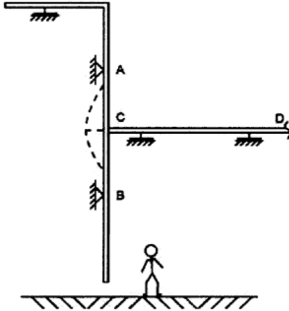
Figure 7-9 Bowing of Hot Line During Startup
