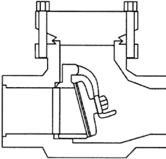
Figure 25-6 Swing Check Valve
