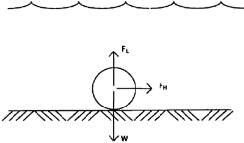
Figure 13-2 Forces Applied to Subsea Pipeline
