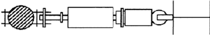
Figure 6-10 Snubber Installed Horizontally
