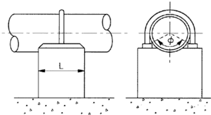
Figure 6-12 Pier Support with Strap
