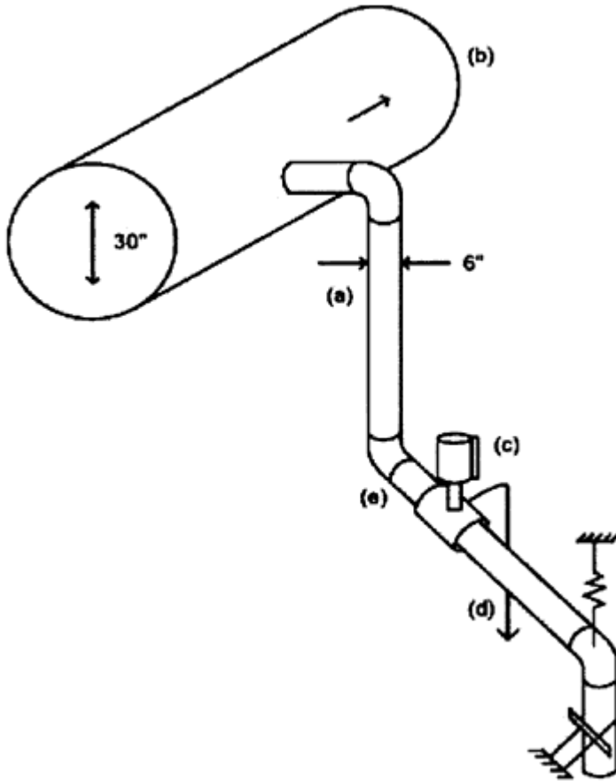
Figure 7-12 Layout of Header and Branch
