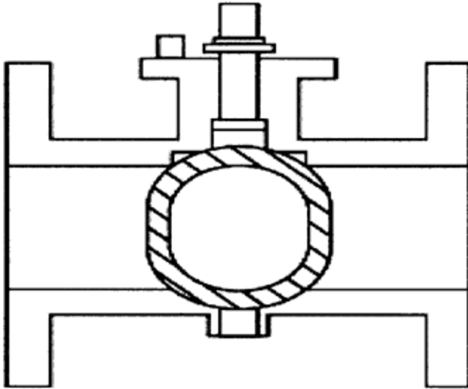
Figure 25-4 Ball Valve
