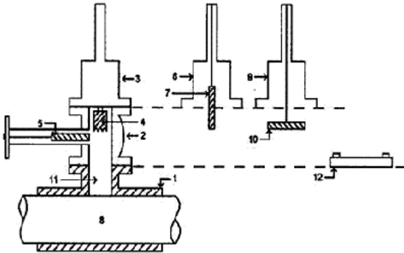
Figure 23-4 Hot Tap
