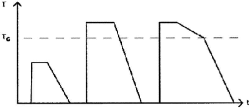
Figure 15-7 Post-Weld Heat Treatment
