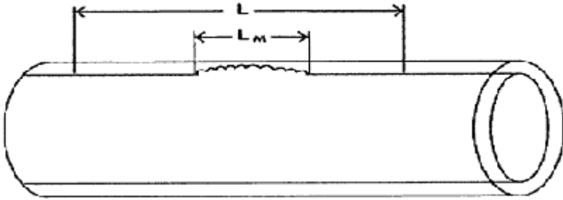
Figure 21-2 Measured Length of Wall Thinning
