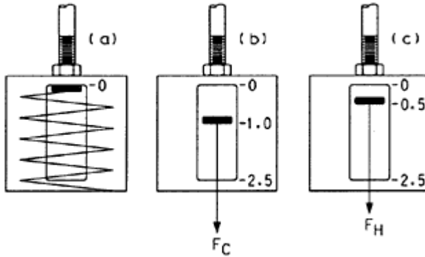
Figure 6-4 Variable Spring Selection Example
