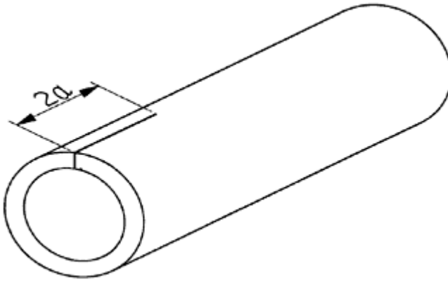
Figure 21-8 Through-Wall Crack of Length 2a
