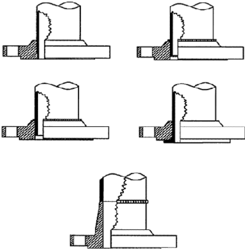
Figure 17-1 Common Flange Types
