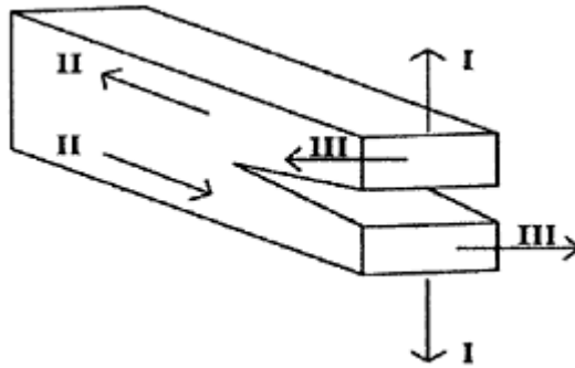
Figure 21-7 Three Modes of Fracture
