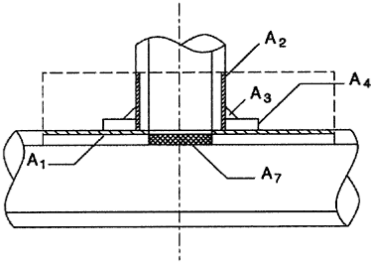
Figure 4-6 Branch Reinforcement Areas
