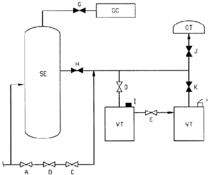
Figure 4-11 Simplified Diagram of Oil-Gas Separator
