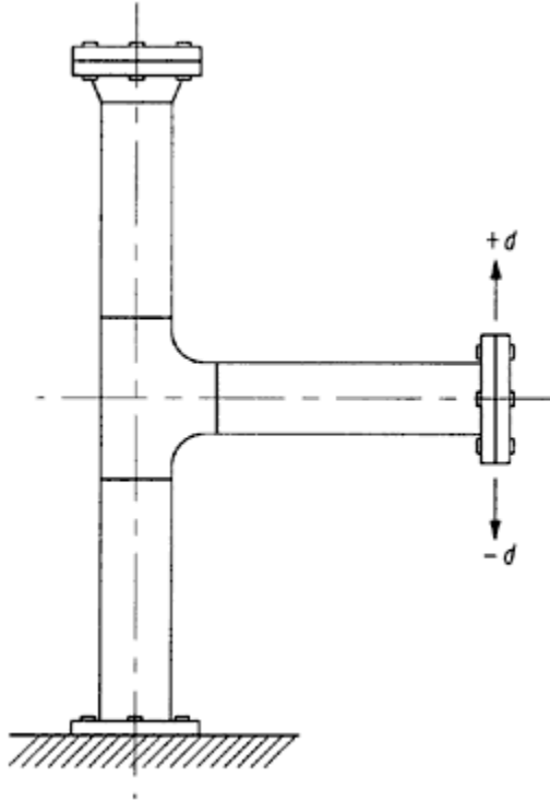
Figure 7-7 Stress Intensification Factor Test
