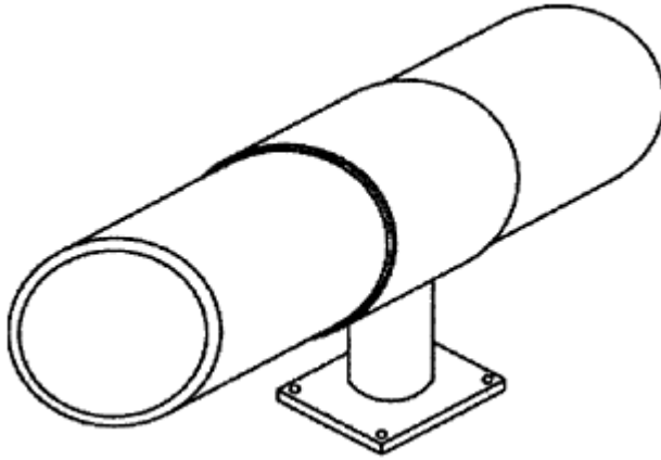
Figure 6-11 Pipe Anchor with Full Encirclement Sleeve
