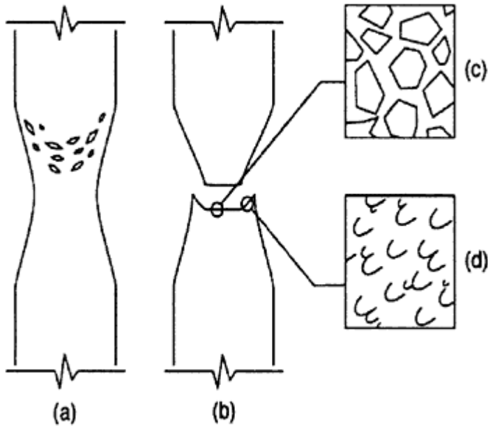
Figure 22-4 Shear and Tension Overload
