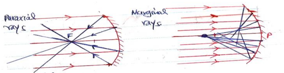
Paraxial rays
