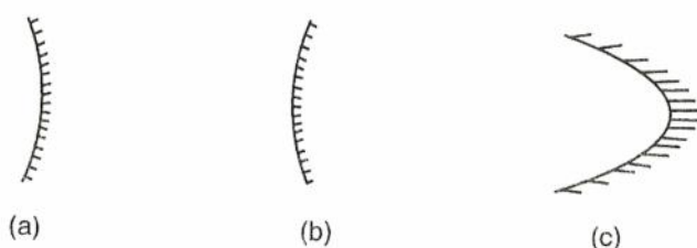
a)concave mirror
