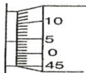
(b) Zero mark of thimble scale does not coincide with the centre line of the sleeve scale. —ve zero error add error to reading
