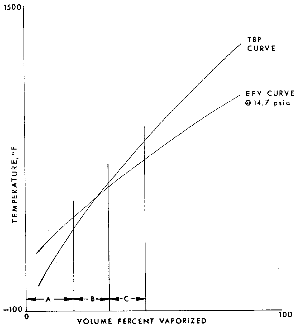
Figure 2.1. TBP and EFV Curves for a typical crude oil and product yield by volume.
