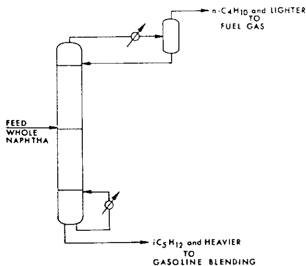
Figure 5.1. Whole naphtha stabilizer with vapor distillate.
