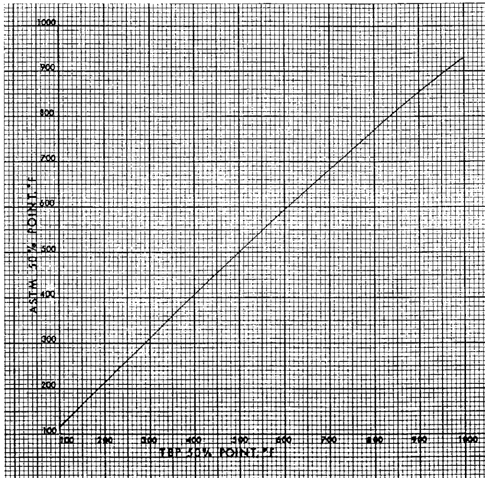
Figure 2.10. Relationship between ASTM and TBP 50 volume percent points.
