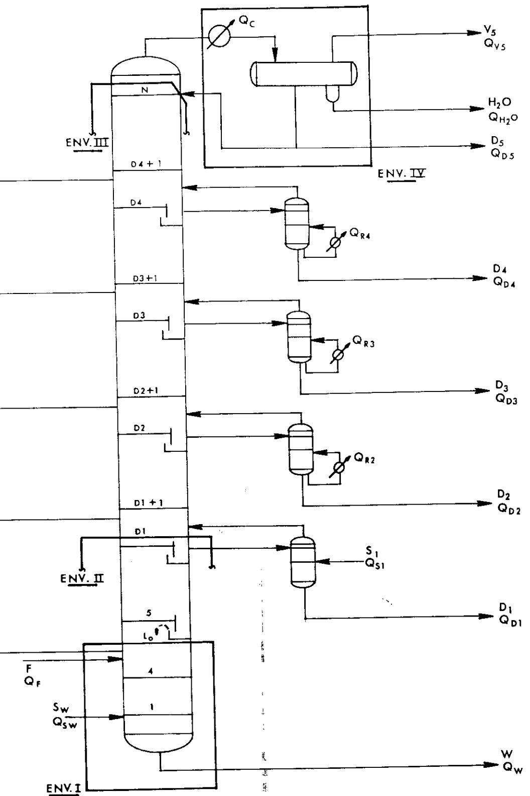
Figure 2.17. Heat and material balance summary—atmospheric tower, Type U.
