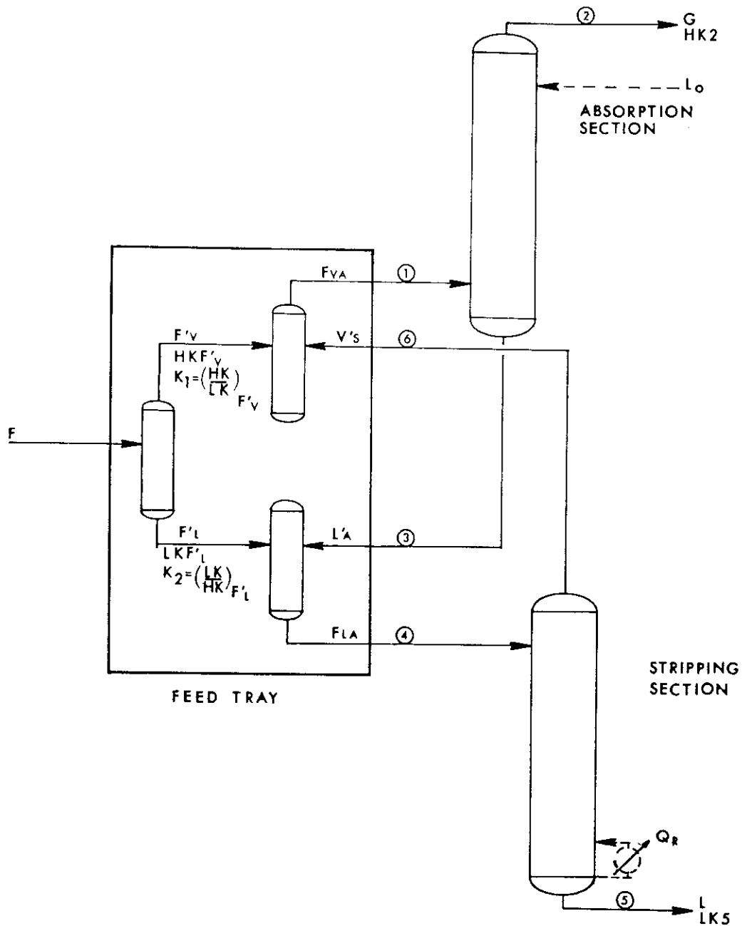
Figure 5.10. Vapor and liquid traffic in a reboiled absorber. Note: lean oil and reboiler not included in overall or feed tray balances.
