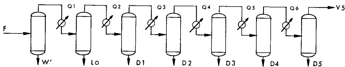
FIG. 2-3a - SERIES OF FLASH DRUMS
