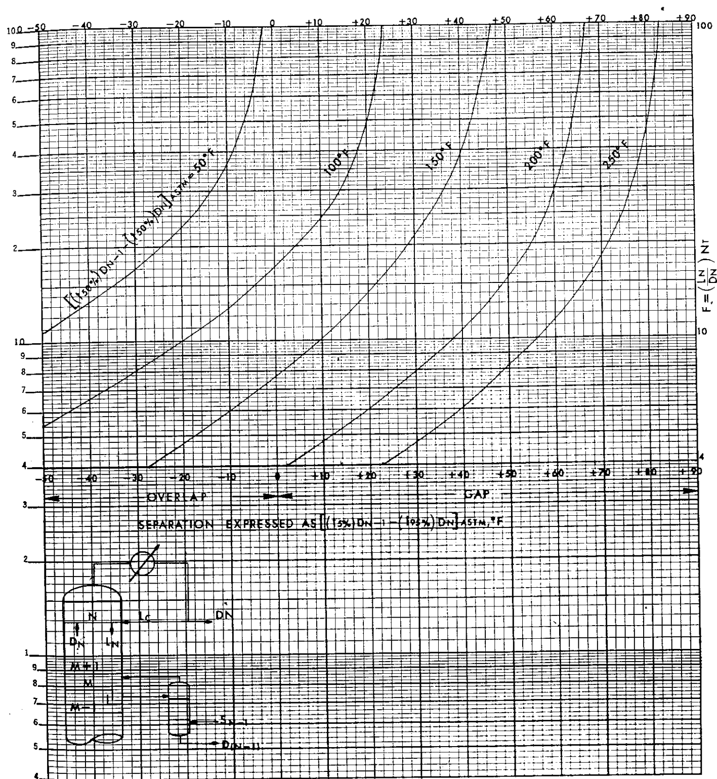
Figure 2.6. Fractionation between total overhead and highest sidestream product, atmospheric crude towers (used with permission of the American Institute of Chemical Engineers).
