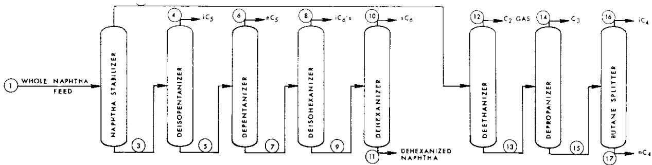
Figure 5.4. Typical flow scheme, refinery saturates gas plant.
