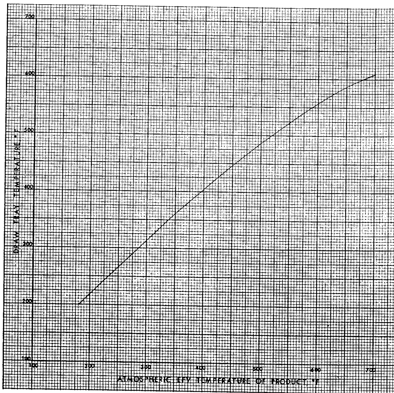
Figure 2.23. Draw/Tray temperatures—Type R tower.
