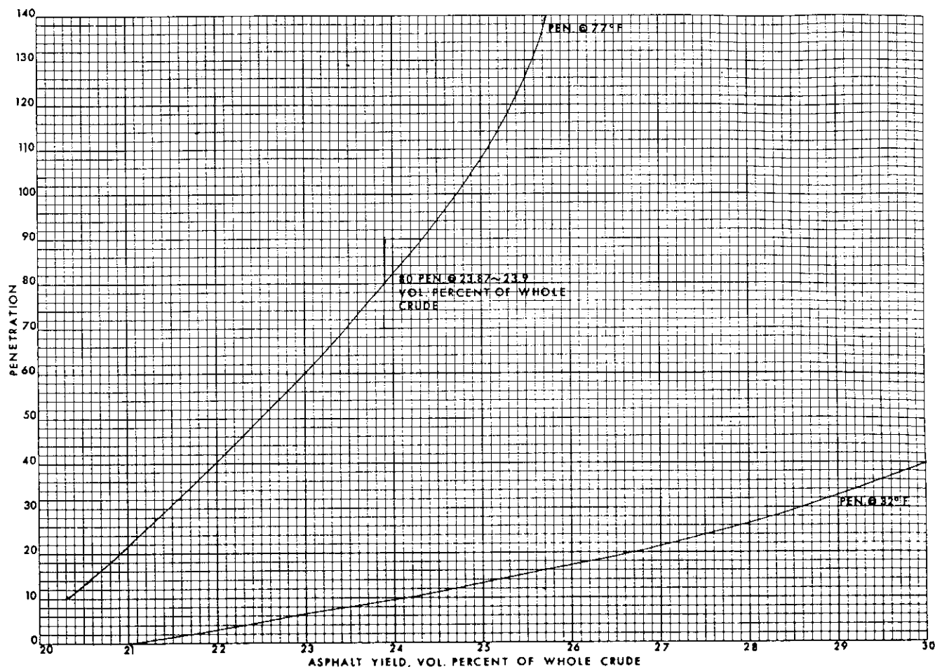
Figure 3.5. Crude assay data. Asphalt yield versus penetration.
