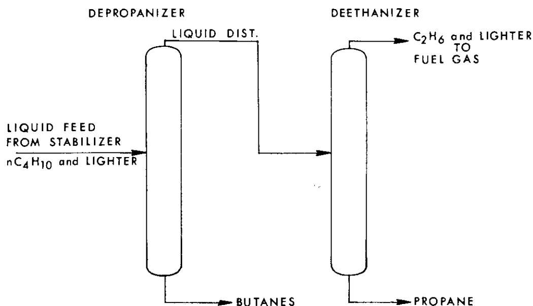
Figure 5.2. LPG recovery from refinery gas.
