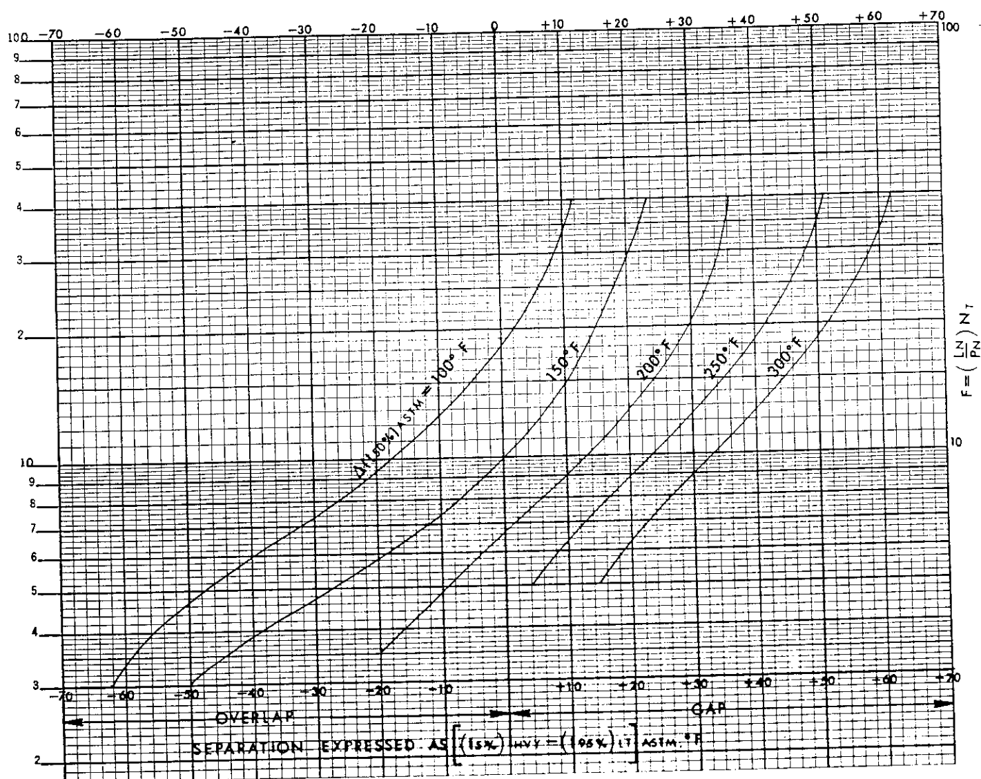
Figure 4.3. Fractionation between sidestream products, catalytic cracking fractionators. (Used by permission of the American Petroleum Institute.)
