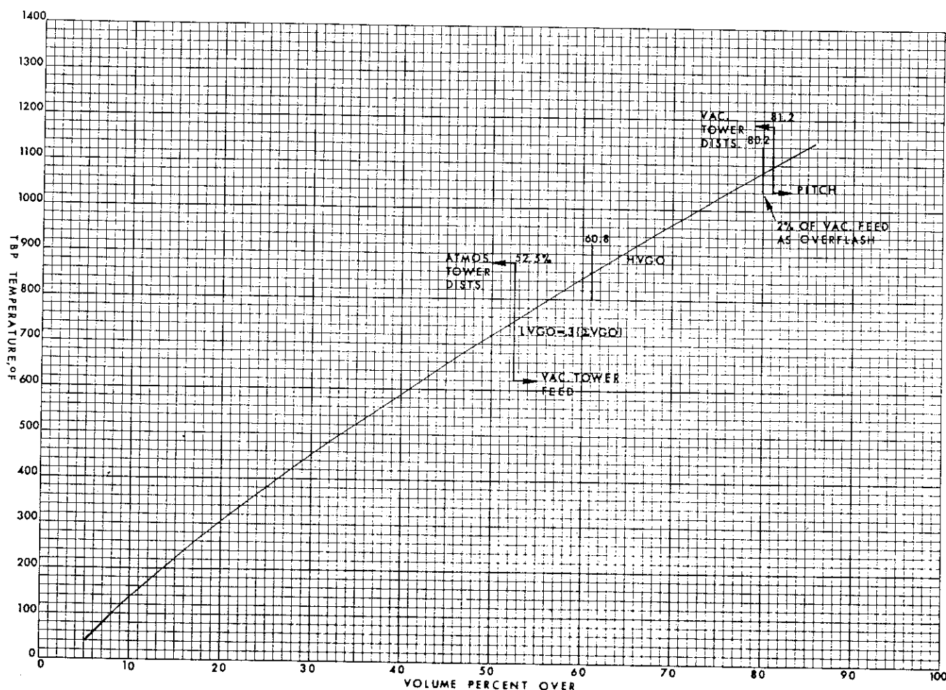
Figure 3.7. Whole crude TBP temperature-yield curve, fuels-pitch operation.
