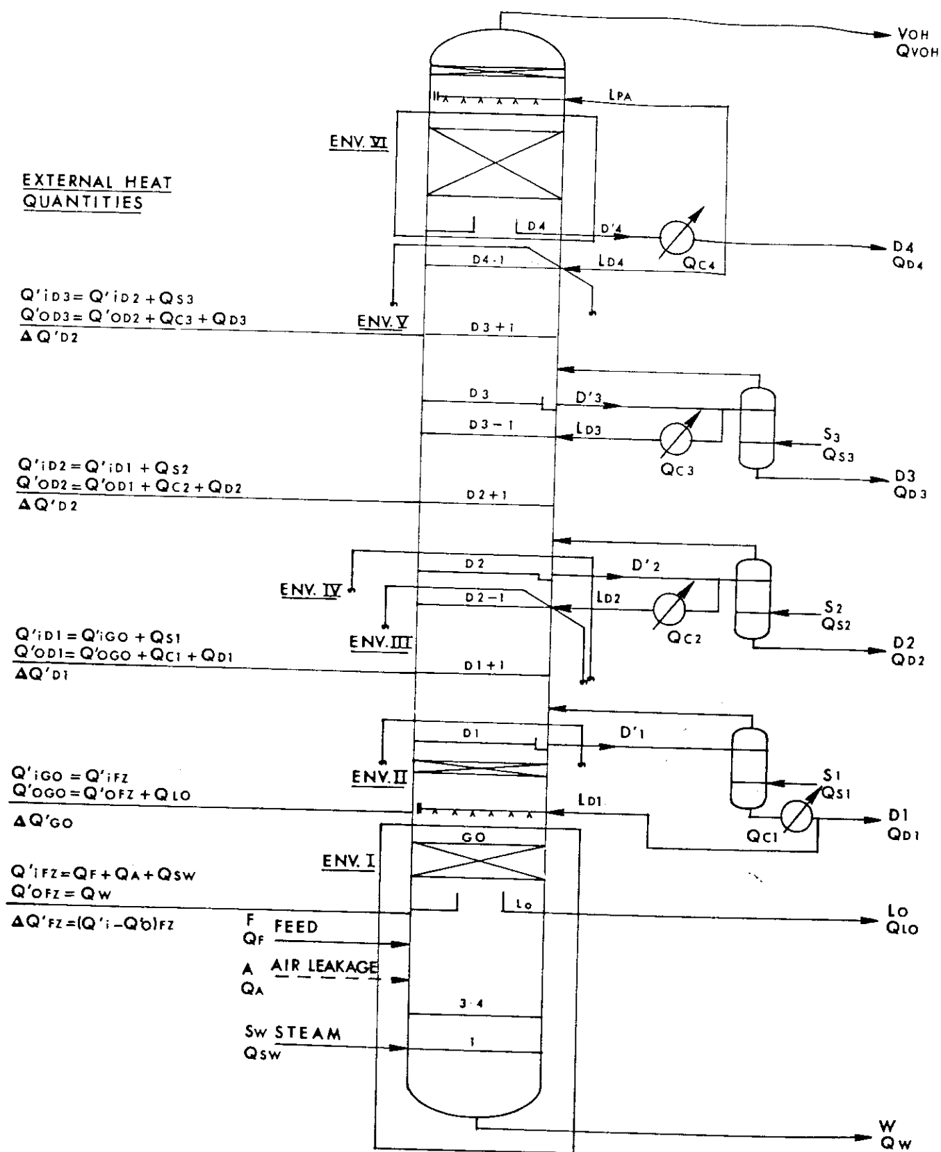
Figure 3.9. Heat and material balance summary, lube type vacuum tower with pumpback reflux heat removal.
