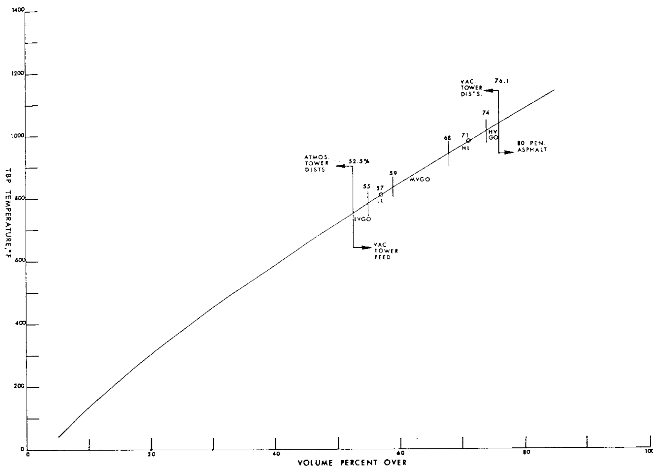
Figure 3.4. Whole crude TBP temperature—yield curve, lube—asphalt operation.
