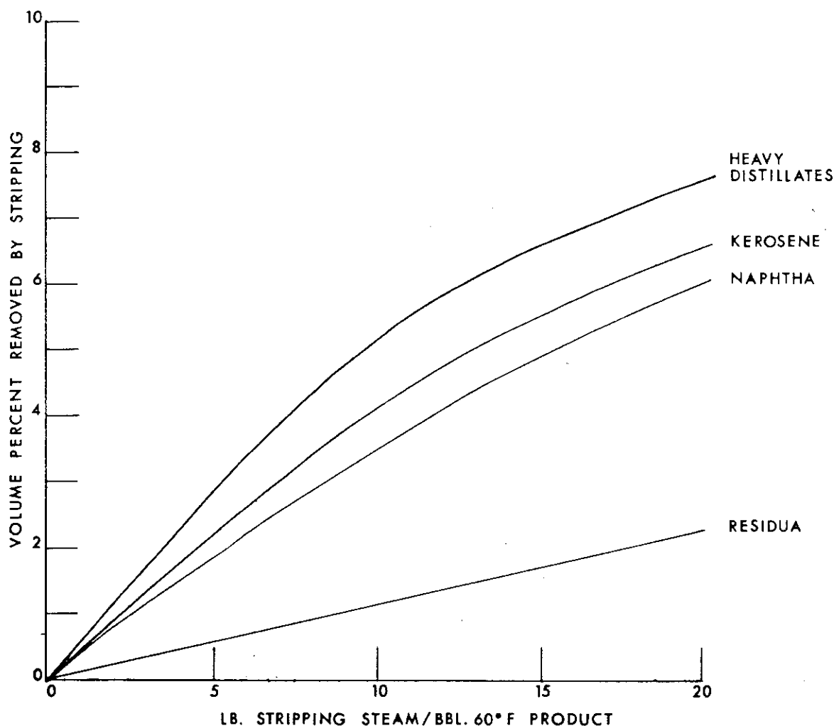
Figure 2.13. Steam stripping of petroleum fractions in four actual trays (with permission of Oil and Gas Journal ).
