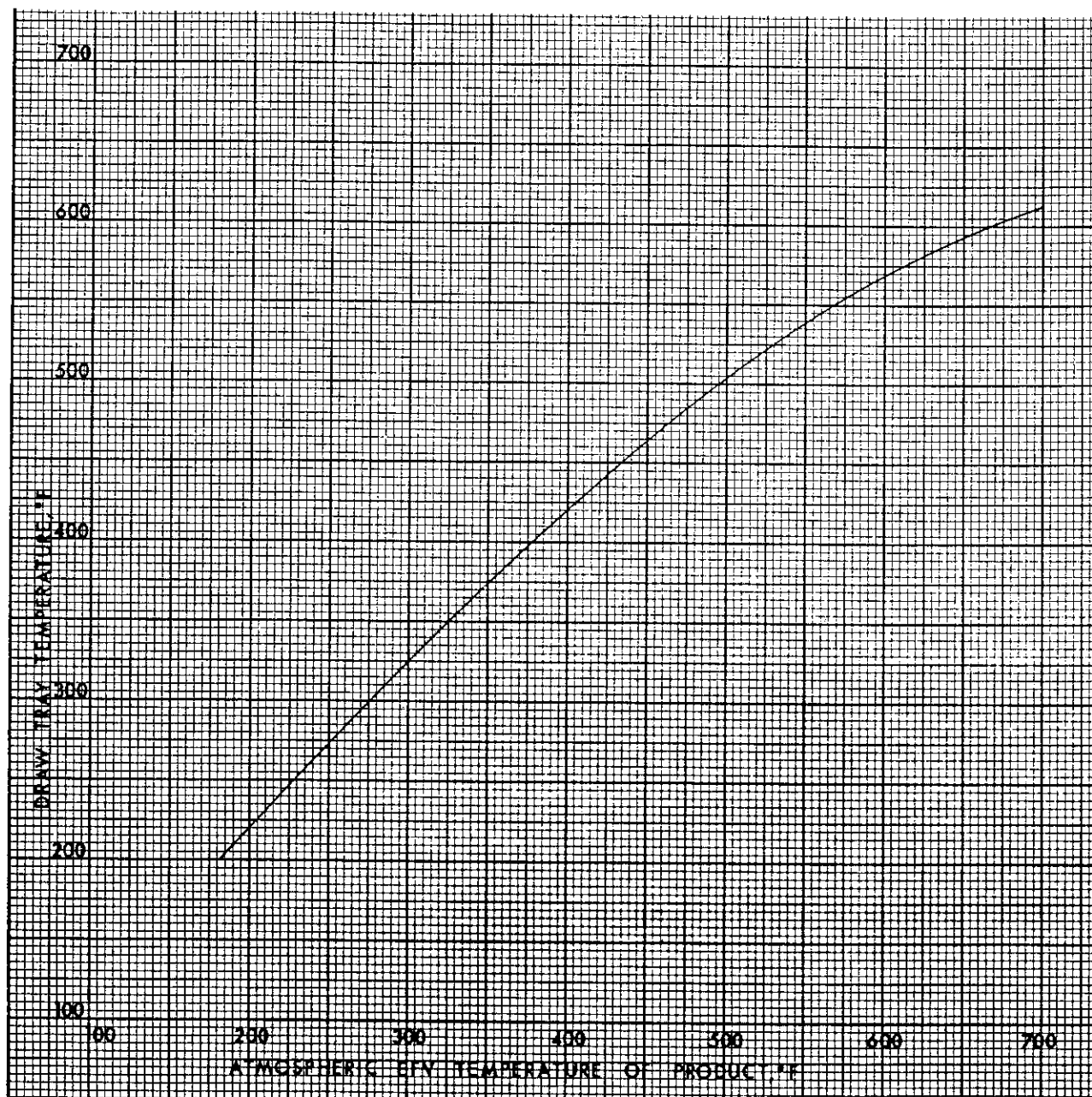
Figure 2.18. Draw tray temperatures—Type U tower.
