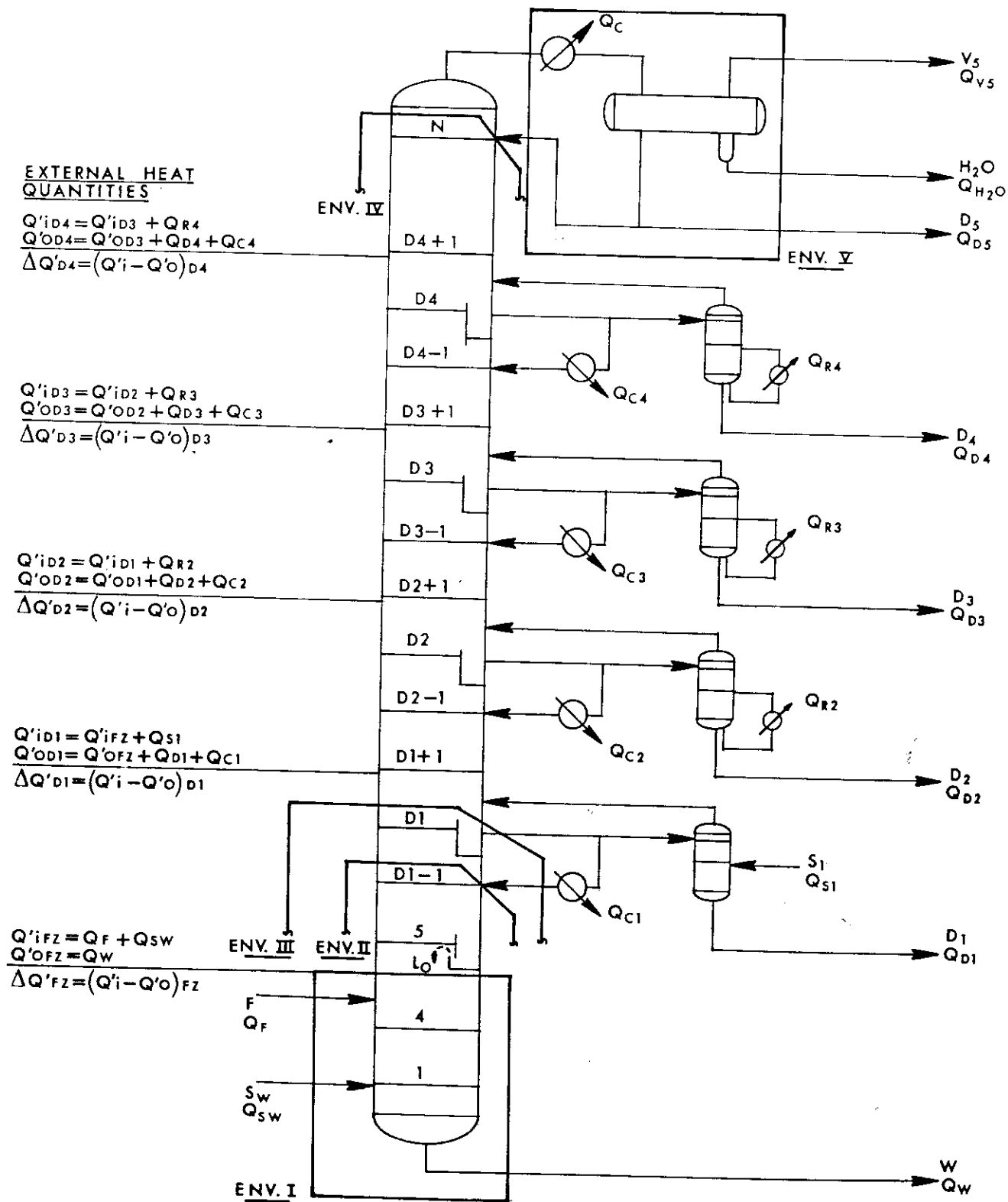
Figure 2.22. Heat and material balance summary—atmospheric tower, Type R.
