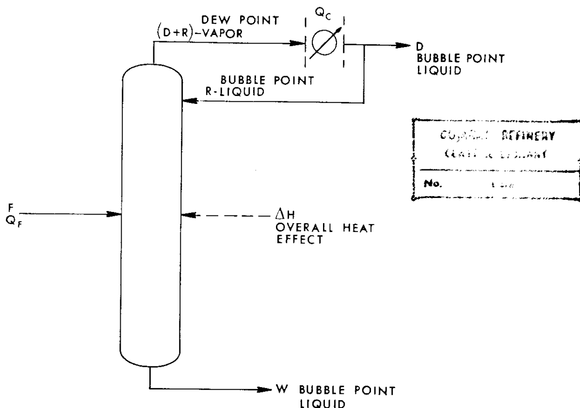
Figure 5.6. Heat requirements for a typical one feed-two product distillation.
