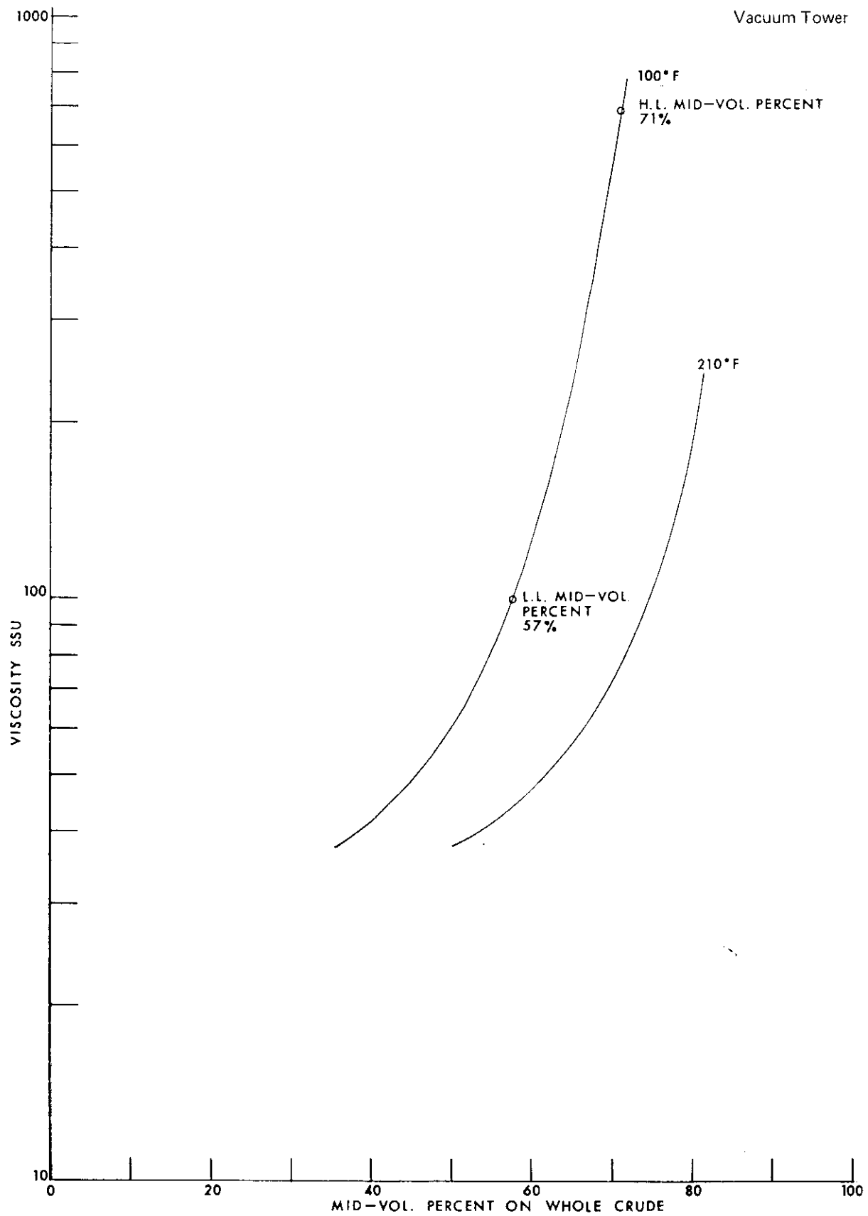
Figure 3.6. Crude assay data, viscosities of vacuum gas oils.
