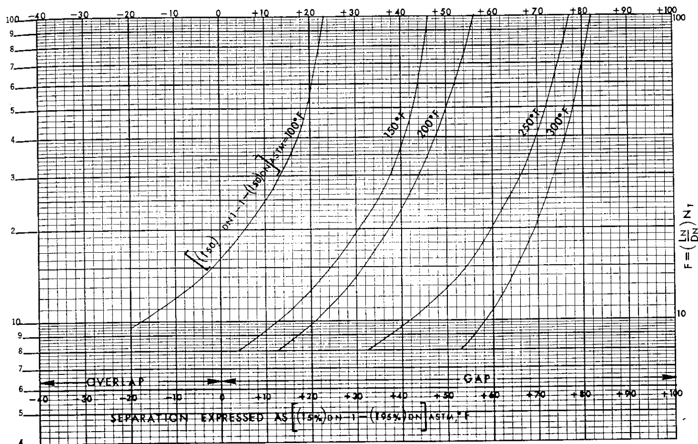
Figure 4.2. Fractionation between total overhead and highest sidestream product, catalytic cracking fractionators. (Used by permission of the American Petroleum Institute.)
