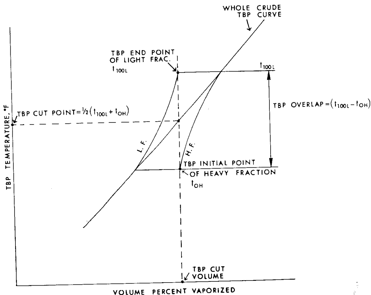
Figure 2.14. Temperature relationships around the cut point between fractions.
