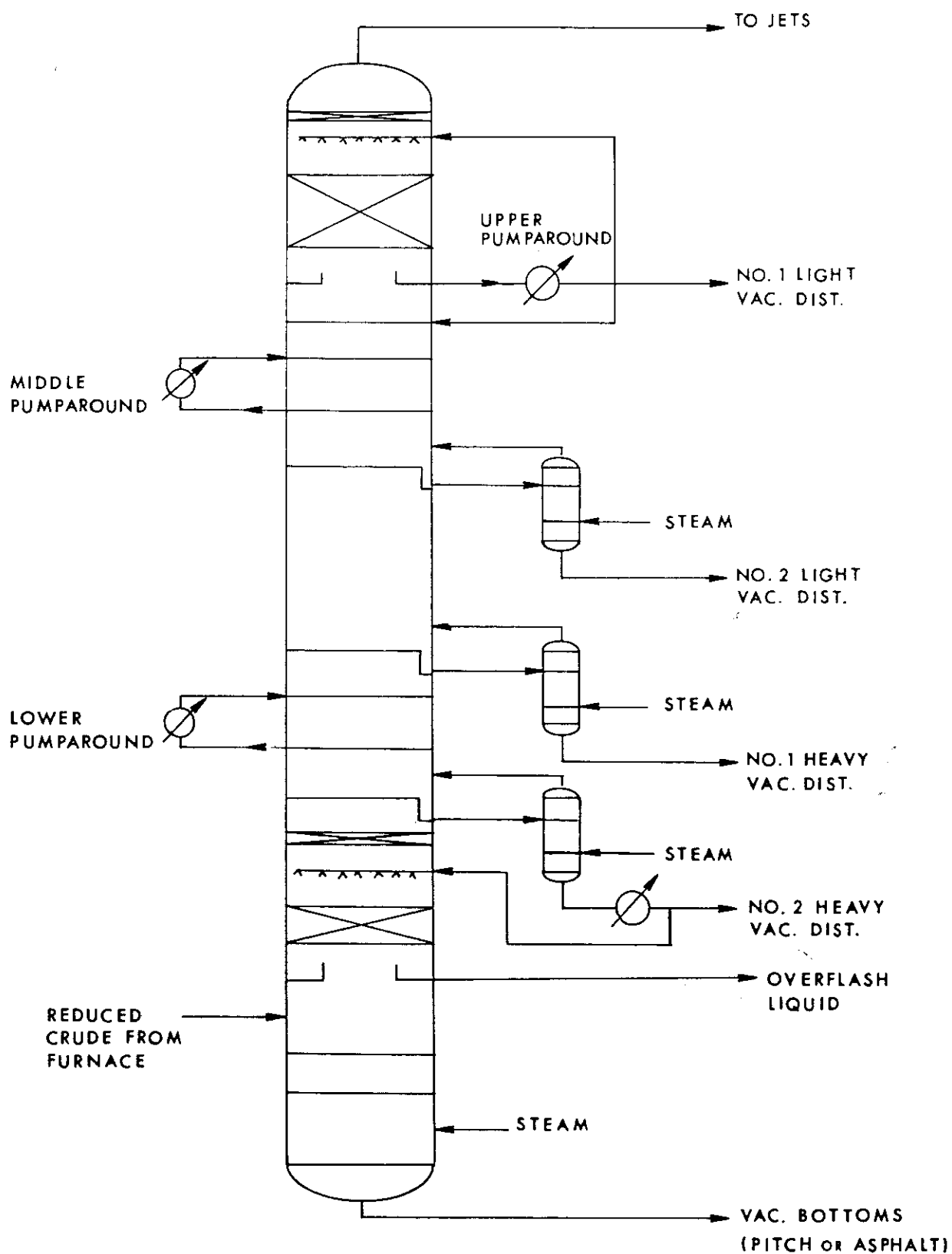
Figure 3.2. Lube type vacuum tower with pumparound reflux heat removal.
