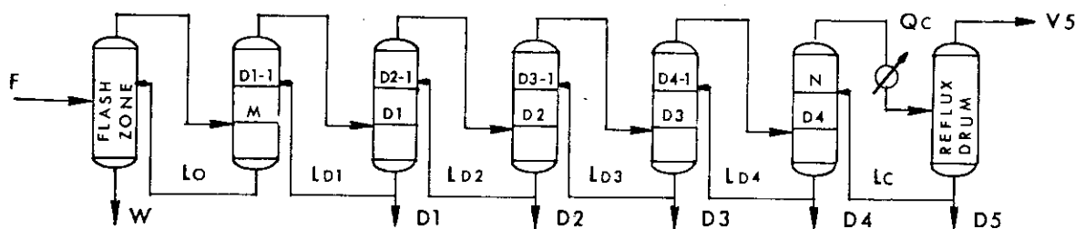
FIG. 2-3b - TYPE U (TOP TRAY REFLUX)
