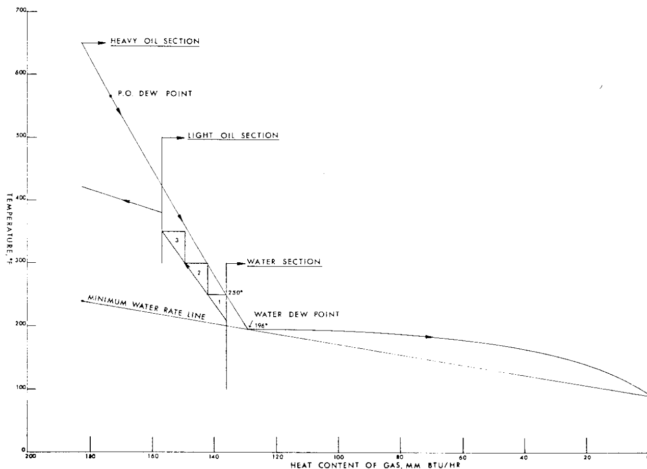
Figure 6.2. Typical cracked gas cooling curve and quench tower temperature profile.
