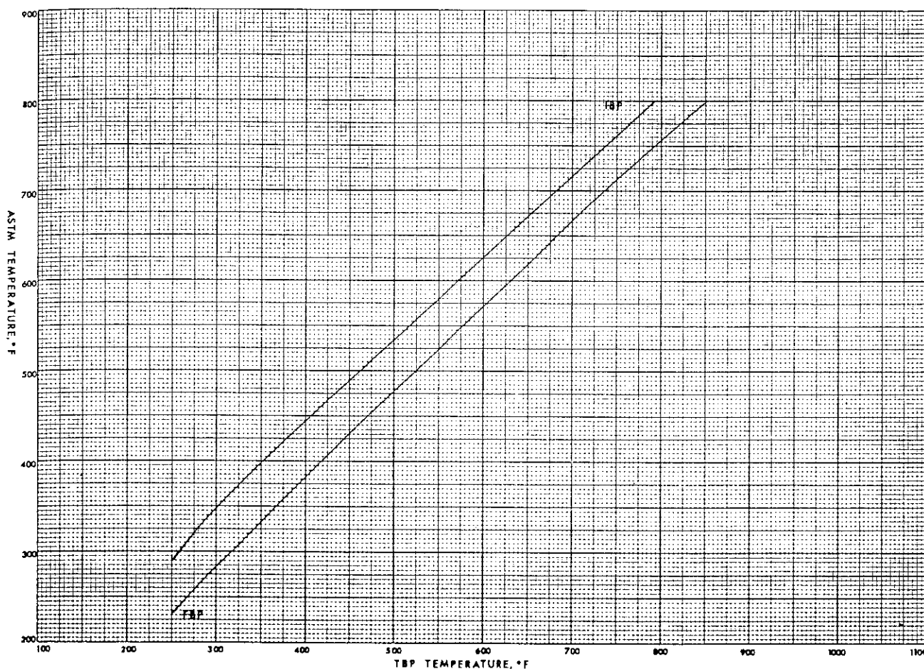
Figure 2.15. Relationships between ASTM and TBP initial (0 percent) and final (100 percent) boiling points.
