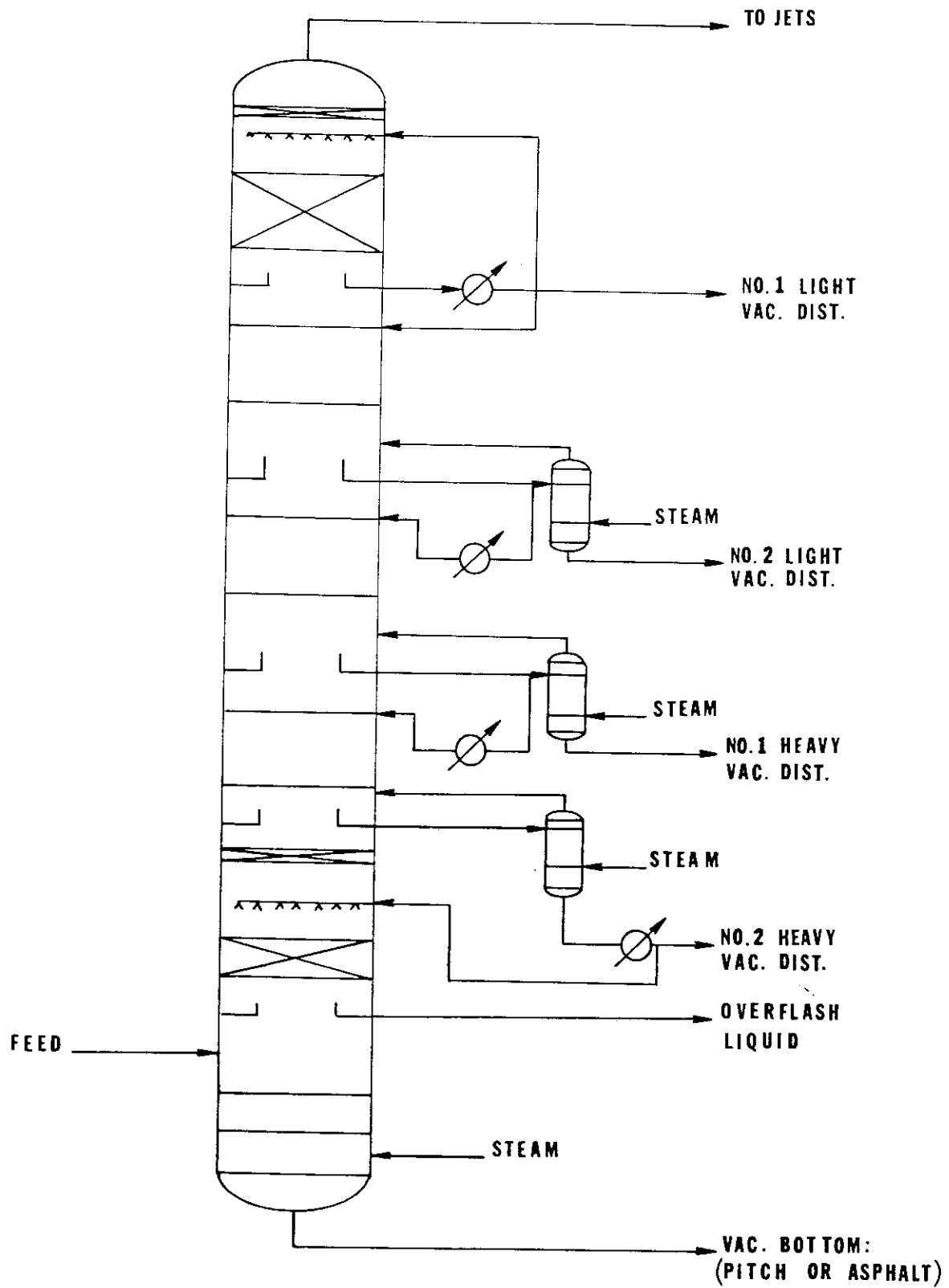
Figure 3.1. Lube type vacuum tower with pumpback reflux heat removal.
