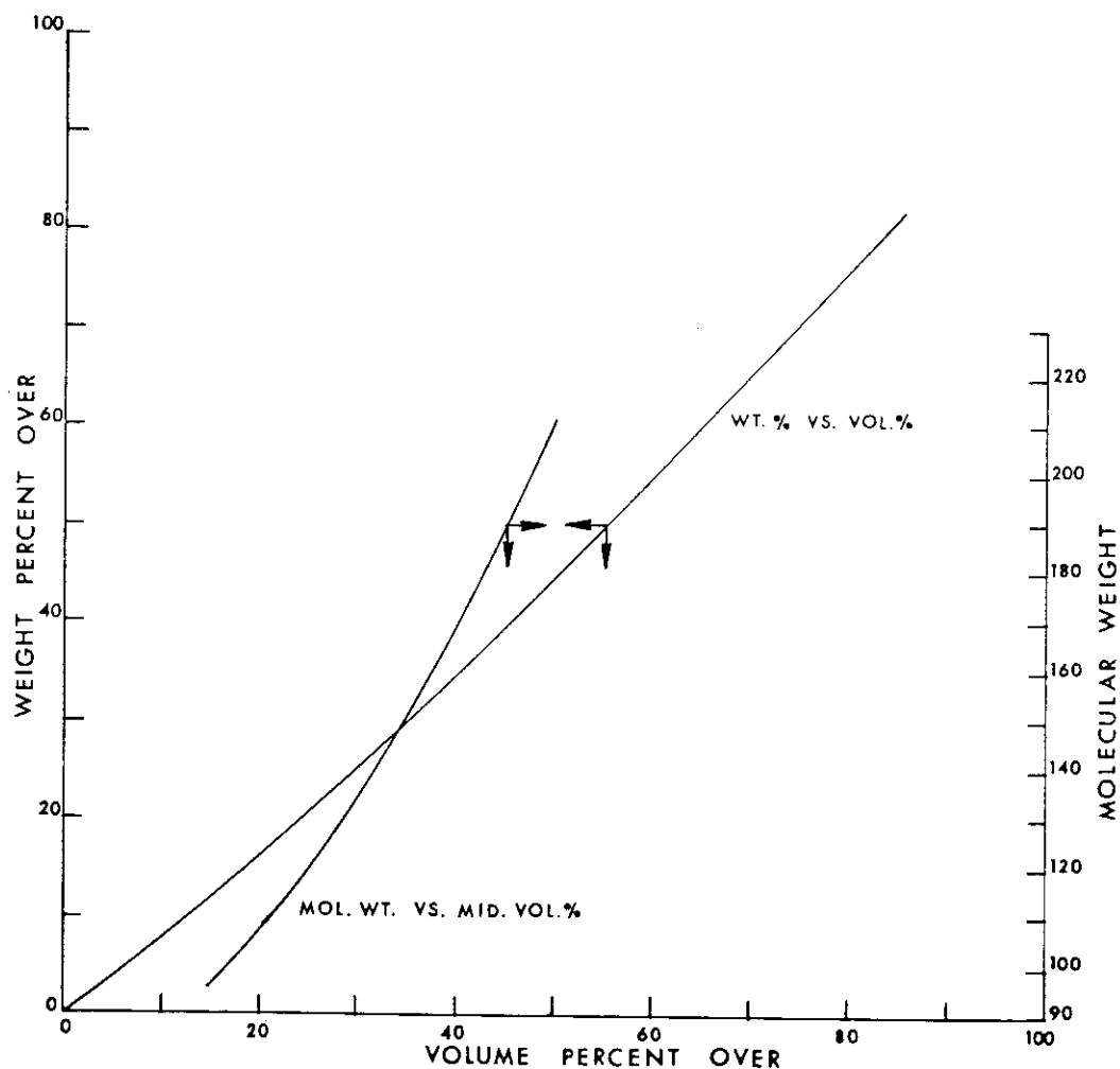
Figure 2.27. 36.3 degree API crude, volume-mole-weight relationships.
