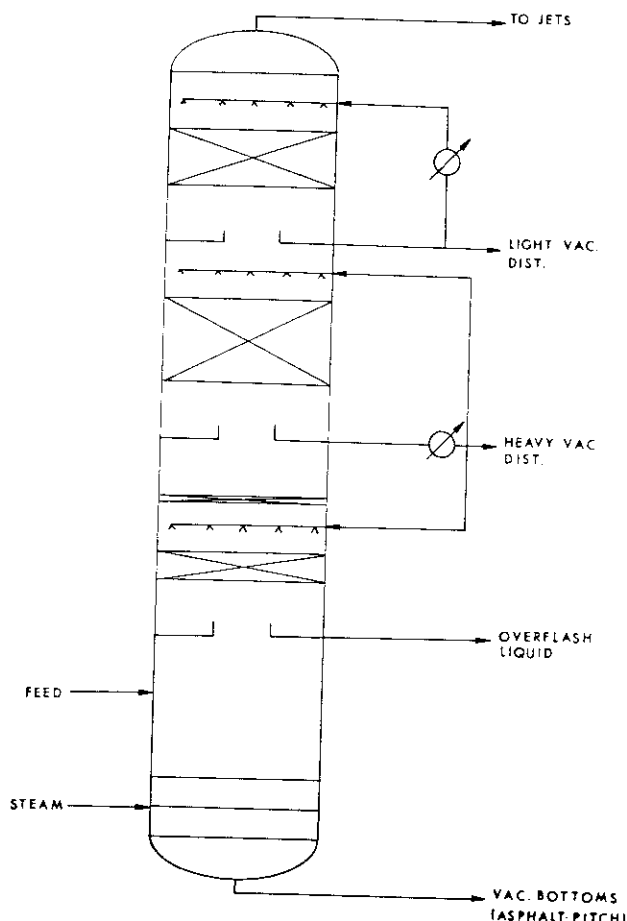
Figure 3.3. Fuels type vacuum tower.
