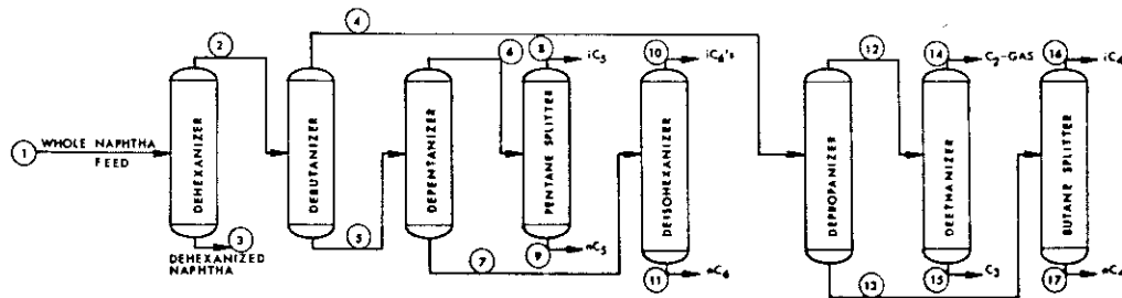
Figure 5.5. Alternate flow scheme, refinery saturates gas plant.
