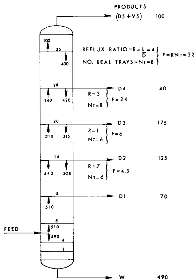
Figure 2.8. Product and reflux volumetric flow rates.
