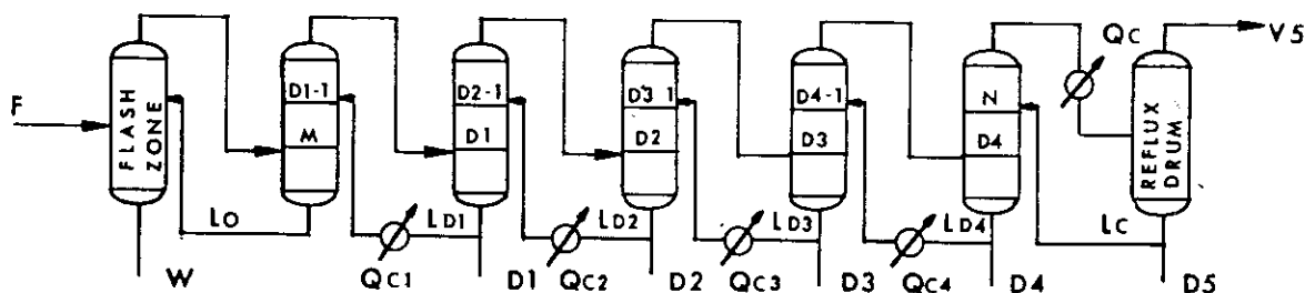
FIG. 2-3d - TYPE R (PUMPBACK REFLUX)
