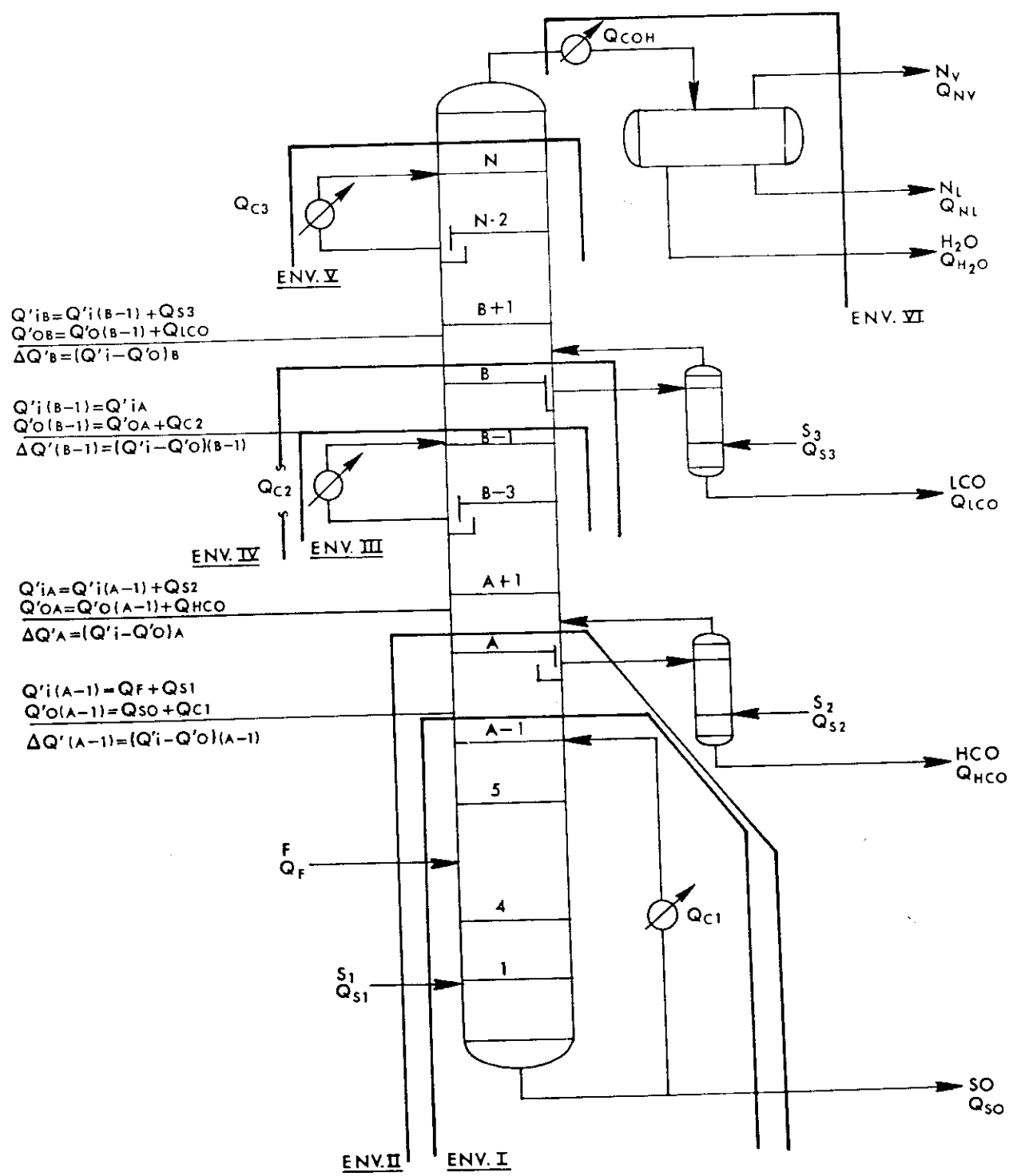
Figure 4.4. Heat and material balance summary, catalytic cracking unit-main fractionator.
