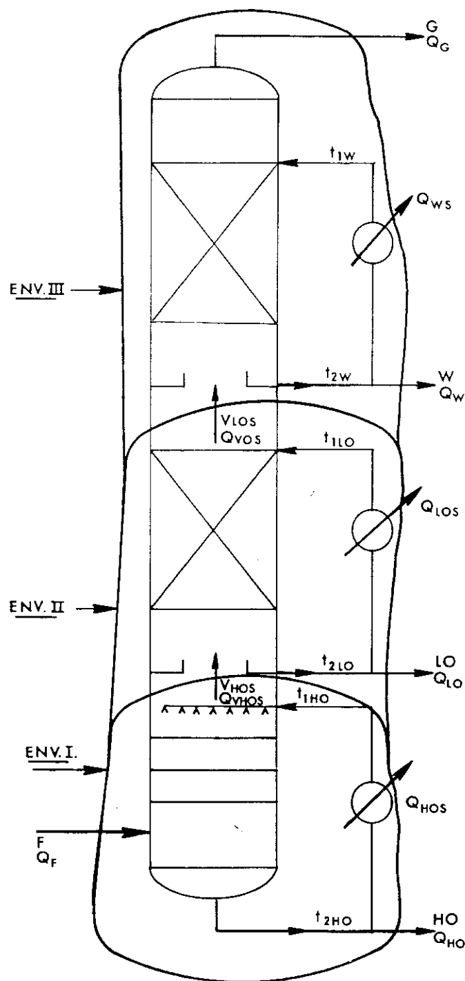
Figure 6.1. Pyrolysis gas combination—oil and water quench tower.
