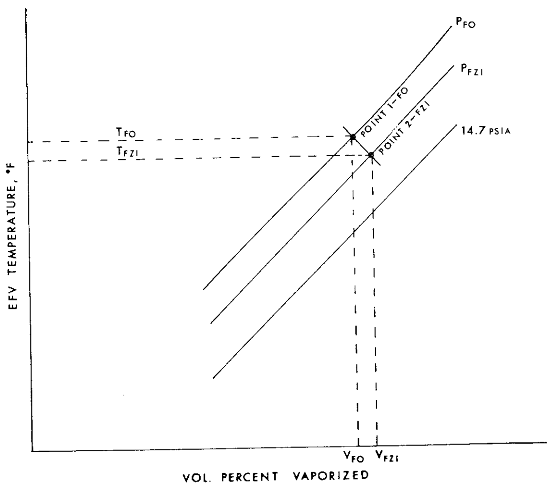
Figure 2.12. EFV curves for whole crude at 14.7 psia, flash zone inlet pressure ( P_{FZI} ) and furnace outlet pressure ( P_{FO} ).
