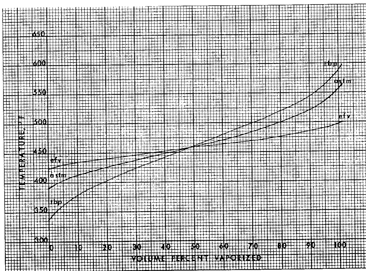
Figure 2.2. ASTM, TBP and EFV curves for 39.7 degree API light distillate.
