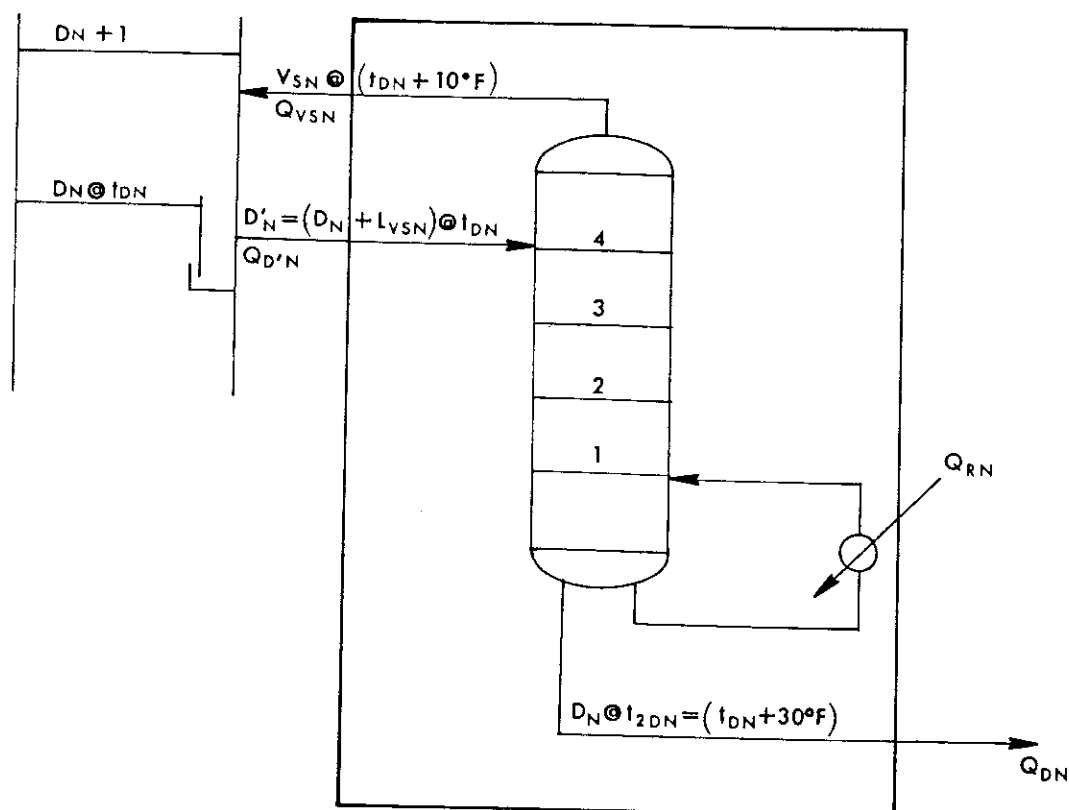
Figure 2.20. Heat and material balance quantities around a reboiled stripper.
