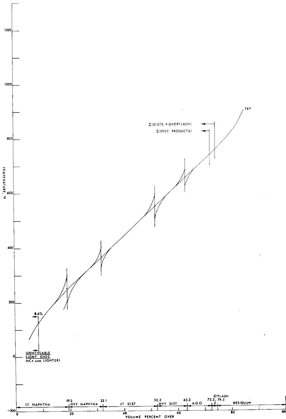
Figure 2.28. 36.3 degree API crude, TBP curves for atmospheric tower feed and products.
