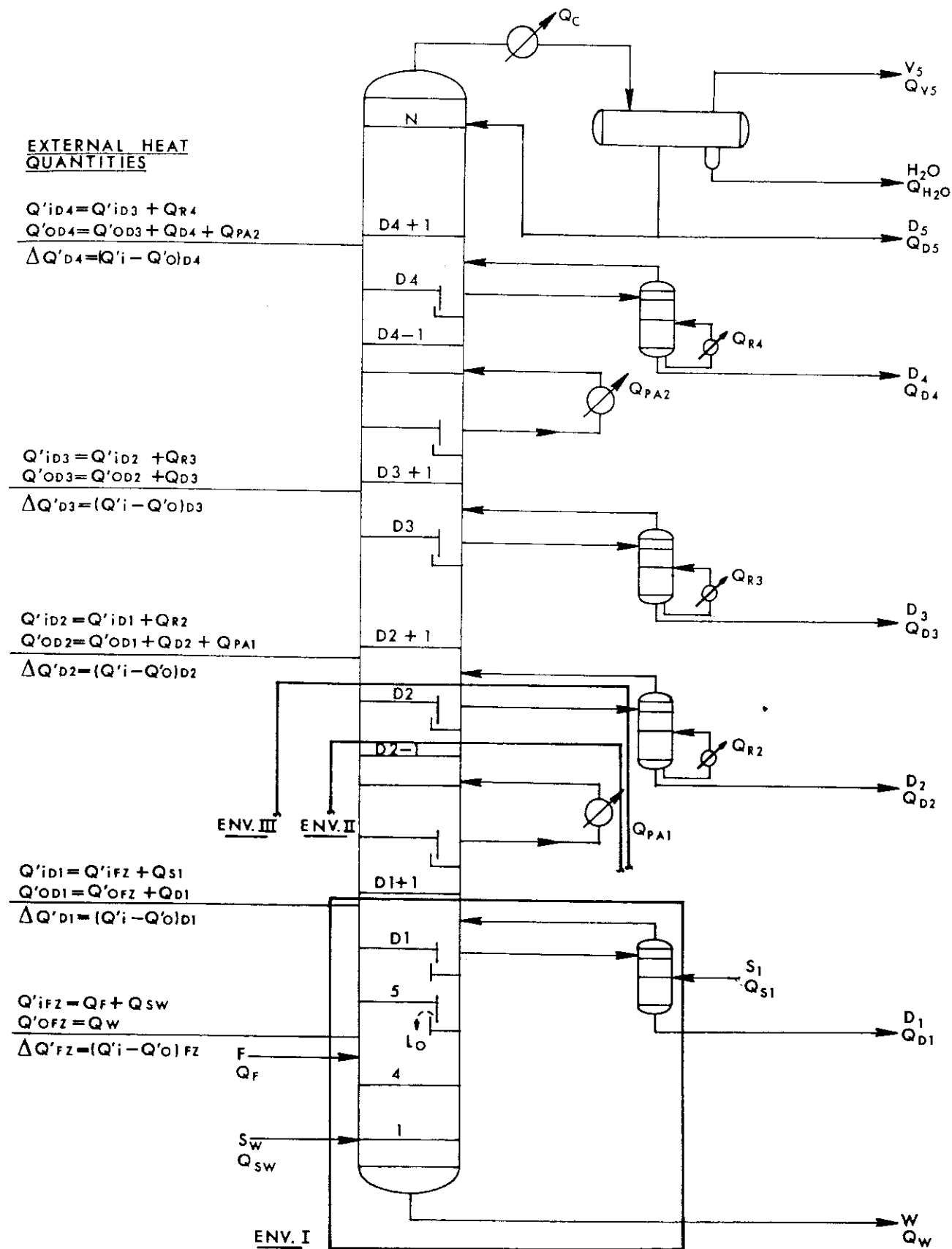
Figure 2.25. Heat and material balance summary—atmospheric tower, Type A with two pumparound circuits.
