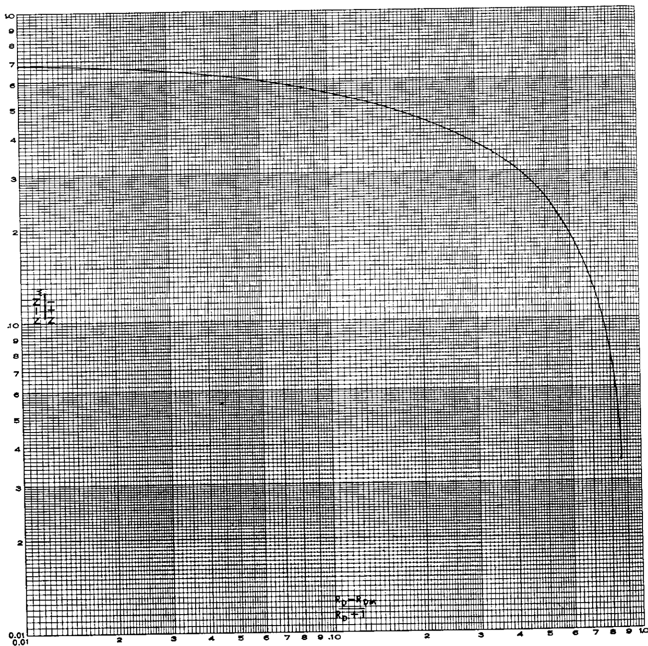
Figure 5.7. Gilliland's correlation, theoretical to real trays (used with permission of the American Chemical Society).
