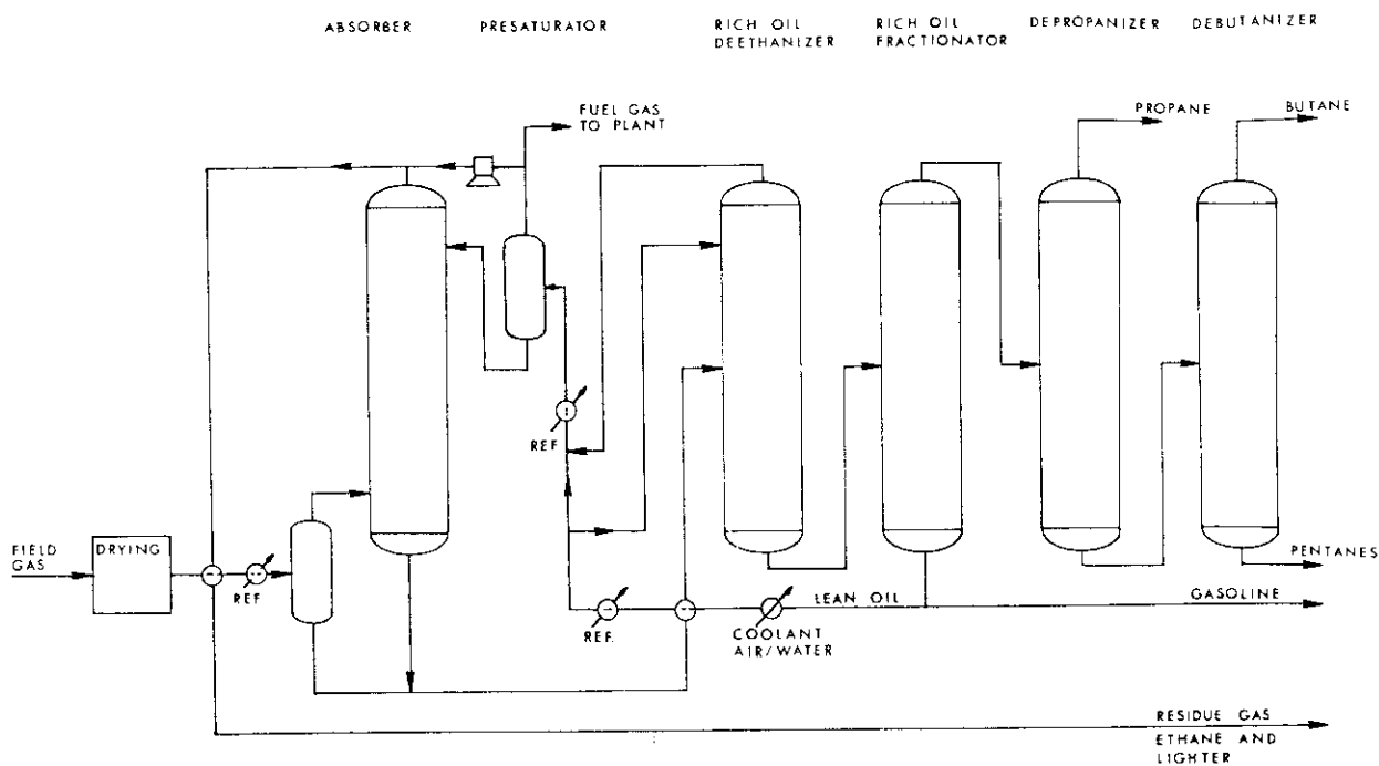
Figure 5.8. Natural gas processing plant for recovering propane and heavier. Note: condensers and reboilers not shown.
