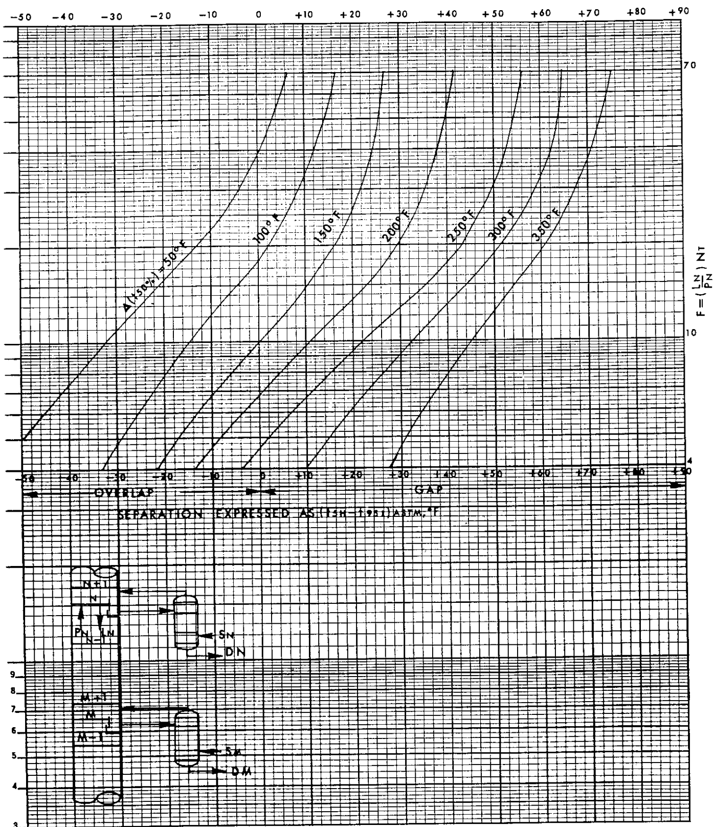
Figure 2.7. Fractionation between adjacent sidestream products, atmospheric crude towers (used with permission of the American Institute of Chemical Engineers).
