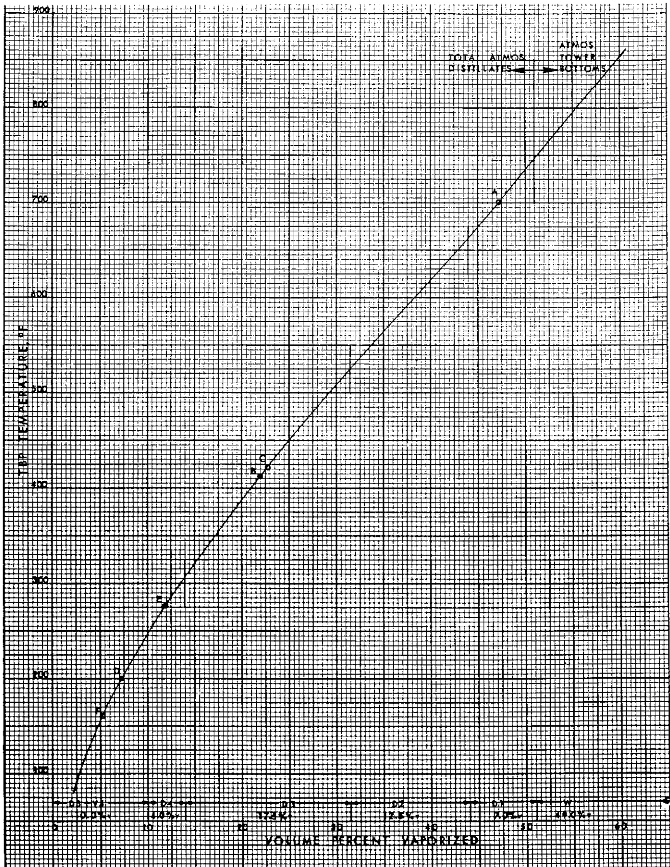
Figure 2.9. Product yield overlay on whole crude TBP curve.
