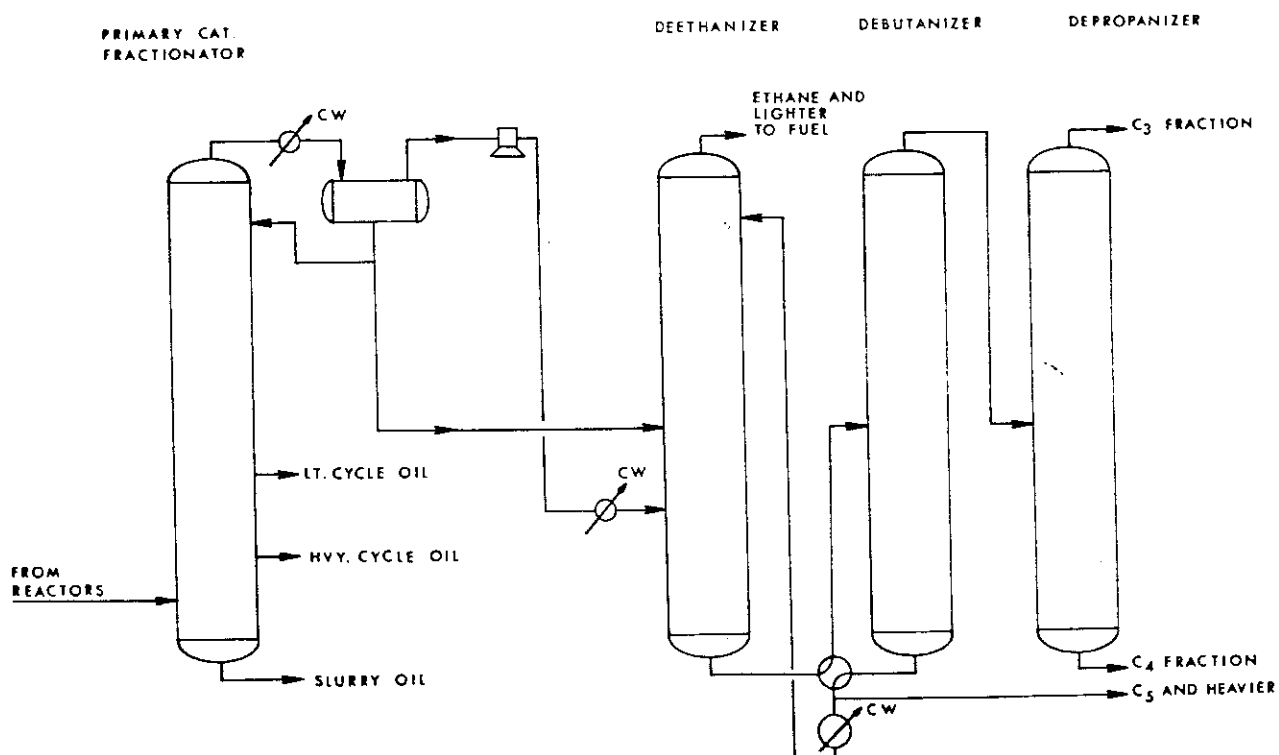
Figure 5.9. FCC unit gas plant for recovering propane and heavier.
