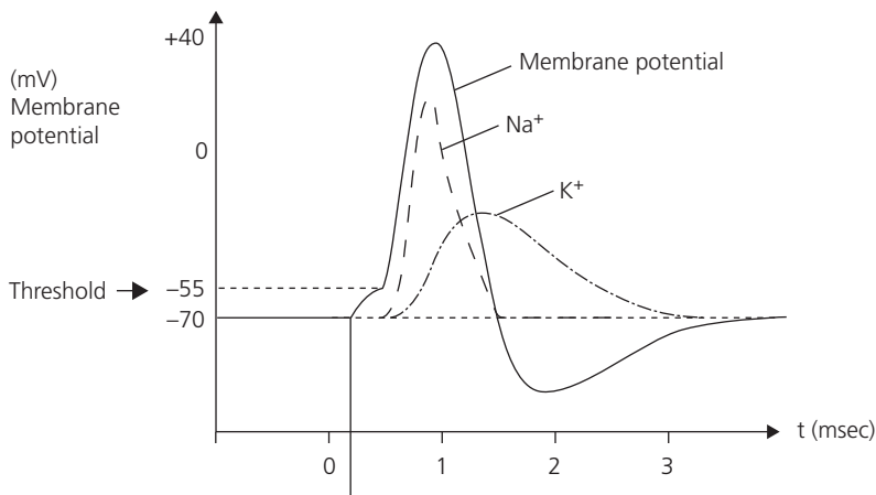
Figure 1.1 The change in Na + and K + conductance and time course of the nerve action potential.
