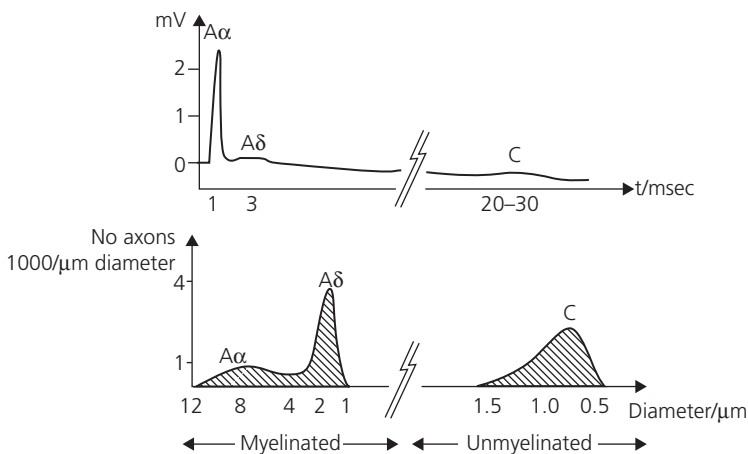
Figure 2.2 Sensory compound action potential waveform, measured in vitro (top panel). Late peaks reflect slow-conducting fibres that are narrow diameter or unmyelinated. They are not detected in routine clinical studies. In clinical practice the A\alpha peak is measured. This corresponds to a small number of large diameter axons.
