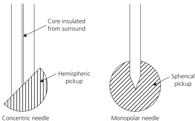
Figure 4.1 Recording volumes of concentric and monopolar EMG needles.
