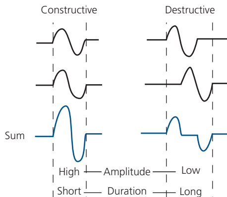
Figure 2.1 Constructive and destructive interference.
