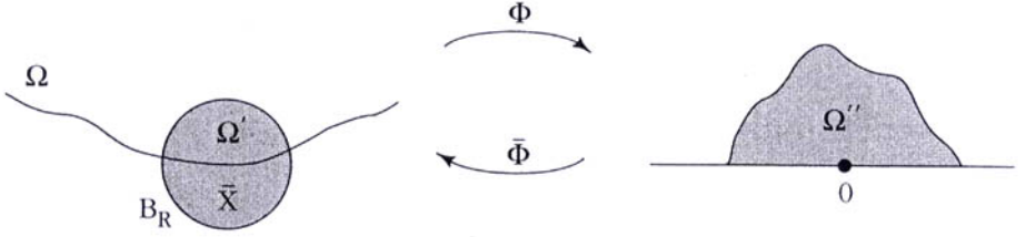
Figure 9.1. Straighting out the boundary.
