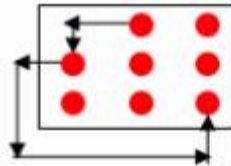
Figure 35: Jumper Setting For Microphone
