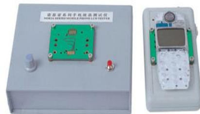
Figure 26: LCD tester
