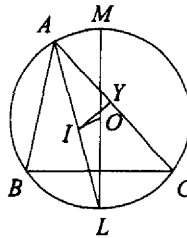
FIGURE 4.30. Euler's formula for [OI] .
