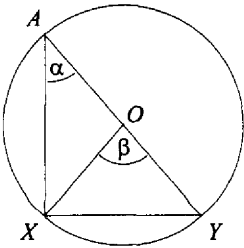
FIGURE 4.4. Central and peripheral angles 1.
