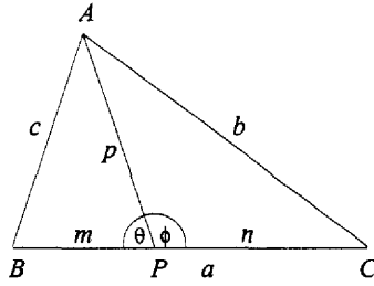
FIGURE 4.3. Proof of Stewart's theorem.
