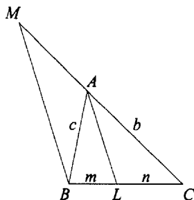
FIGURE 4.20. Angle bisectors.
