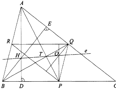
FIGURE 4.14. Euler's line.
