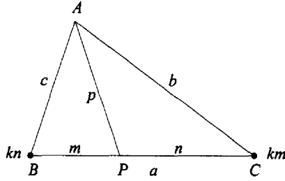
FIGURE 4.13. Another proof of Stewart's theorem.
