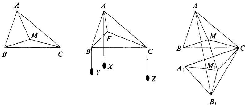
FIGURE 4.16. Fermat's point.
