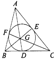
FIGURE 4.22. Gergonne's point.
