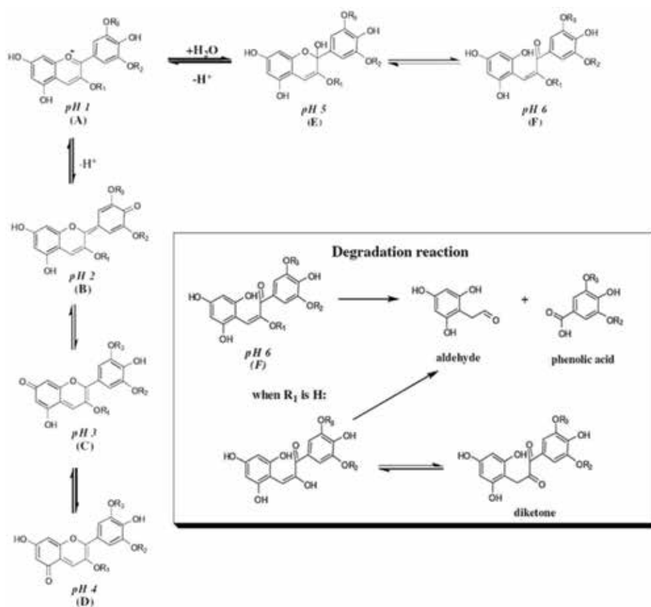
Figure 3. Anthocyanin chemical structure forms depending on pH. Source: Castaneda-Ovando et al. [67].
