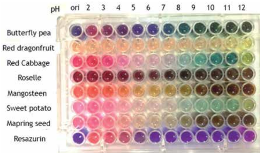
Figure 4. Color chart of anthocyanins extracted from different sources of plants at different pH levels, compared to chemical dye (resazurin). Source: Rawdkuen et al. [56].
