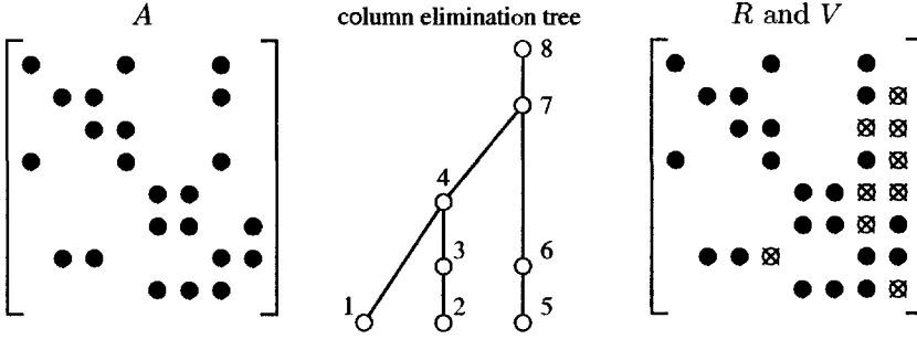
Figure 5.1. QR factorization
