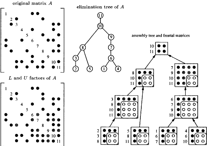
Figure 6.1. Multifrontal example
