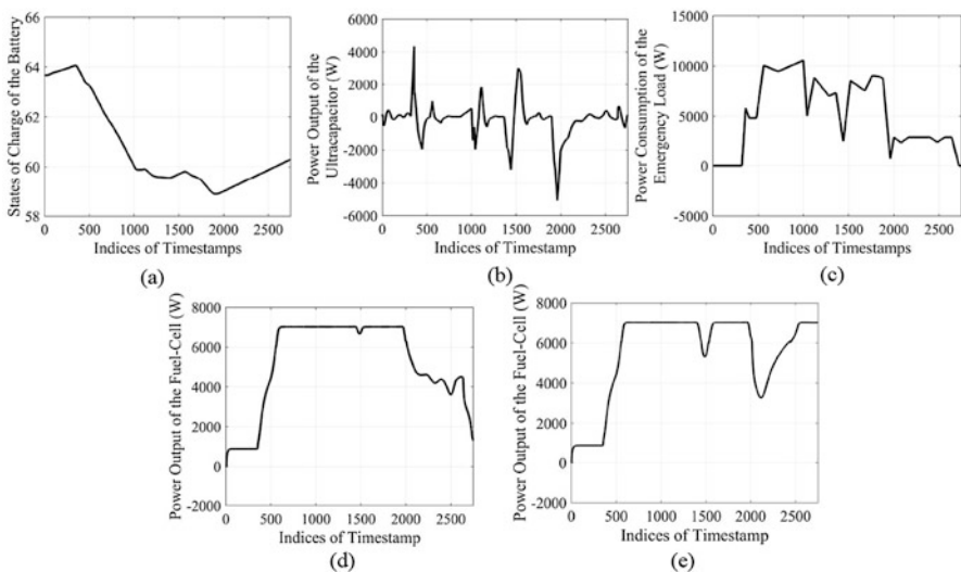
Fig. 4 Original measurement data obtained from APU for, (a) the SOC of the battery; (b) the power output of the ultracapacitor P_{UC} ; (c) the power consumption of the emergency load P_L ; (d) the power output of the fuel-cell P_{FC} ; and (e) power output of the fuel-cell P_{FC} with a simulated FDI attack
