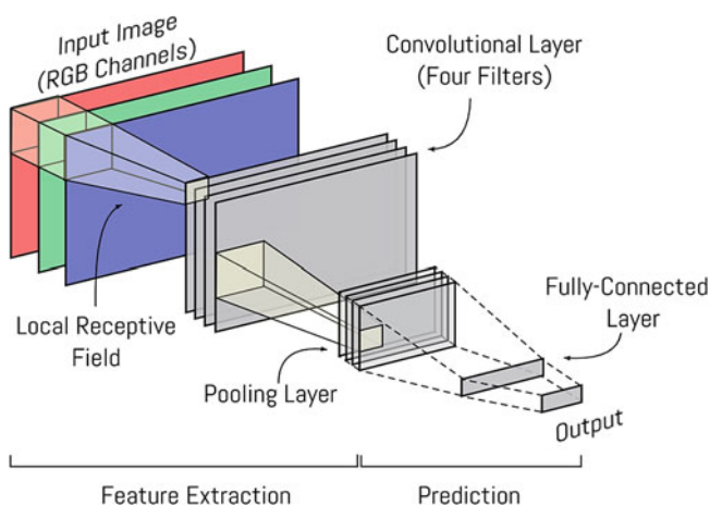
Fig. 1 The structure of a typical CNN used for image classification. The convolutional and pooling layers form the feature extraction stage while the fully-connected layers form the prediction stage
