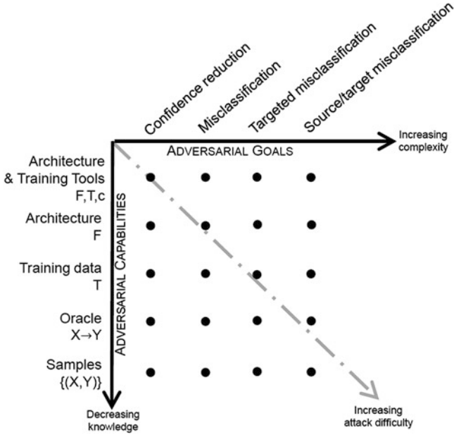
Fig. 1 Different types of attacks in adversarial learning [24]
