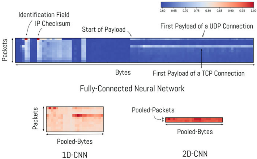
Fig. 11 Three heatmaps showing the important features in the input of the first fully-connected layer of the fully-connected neural network, 1D-CNN and 2D-CNN
