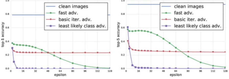
Fig. 5 Top-1 and top-5 accuracy of Inception v3 under attack by different adversarial methods and \epsilon values. The accuracy was computed on 50,000 validation images from the ImageNet dataset [13]
