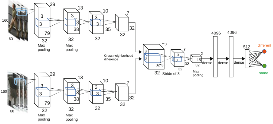
Fig. 3 The architecture of PersonNet. The network takes a pair of RGB images as input, which is put through a stack of convolution layers, matching layer, and higher layers computing relationships between them
