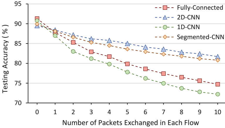
Fig. 12 Accuracy of each neural network on the test set with respect to the number of packets that were exchanged in each flow. Packets were exchanged with the next consecutive packet in the flow
