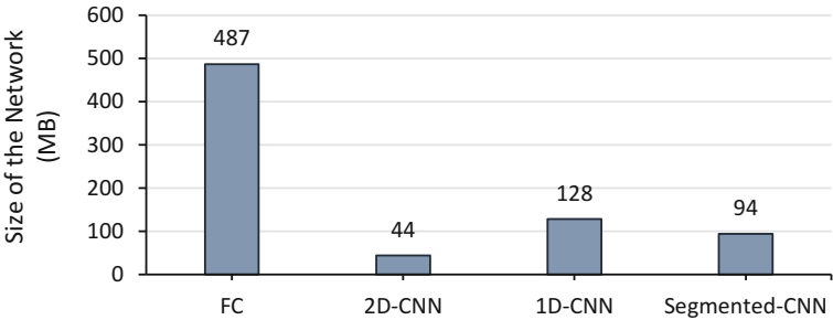
Fig. 7 Approximate size of the neural network in memory
