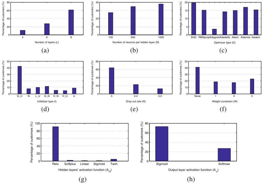
Fig. 7 Feed-forward grid search analysis results for all customers. (a) Optimal layers. (b) Optimal neurons. (c) Best optimizers. (d) Optimal initializer. (e) Optimal dropout rate. (f) Optimal weight constraint. (g) Optimal hidden layer activation. (h) Optimal output layer activation
