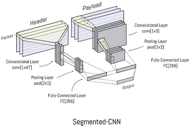
Fig. 5 Structure of a Segmented-CNN showing how the two CNN networks can be individually optimised for the two distinct regions of a packet, the header and payload. Only the first convolutional, pooling, and fully-connected layers of the Segmented-CNN have been shown
