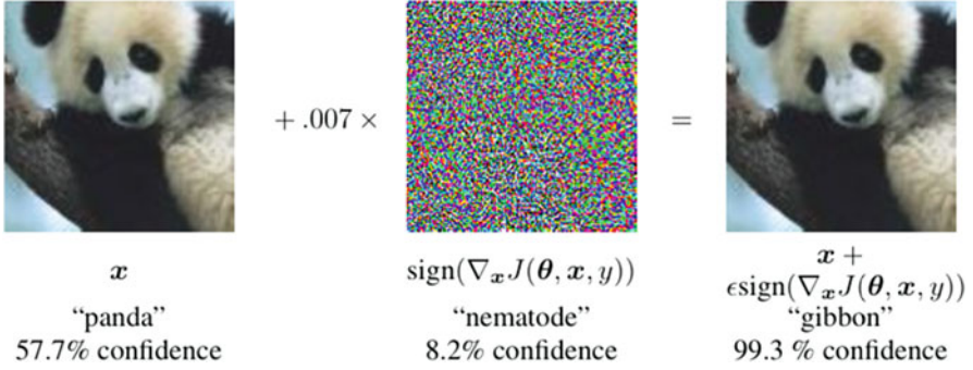
Fig. 4 A demonstration of fast adversarial example generation applied to GoogLeNet [28] on ImageNet [5]. By adding an imperceptibly small vector to the input, GoogLeNet’s classification of the image is changed [7]
