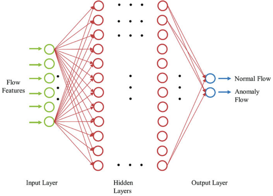
Fig. 1 The deep neural network structure
