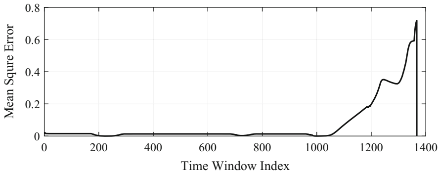
Fig. 6 MSE between compromised data obtained from simulation and predictions obtained from deep learning-based method
