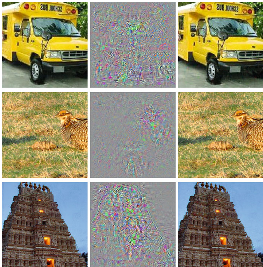
Fig. 2 Adversarial samples generated on AlexNet dataset. Left column is the original image, middle column is the computed perturbations, and right column is the adversarial sample. The images in the right column are predicted incorrectly to be an ostrich, Struthio, and camelus separately [30]
