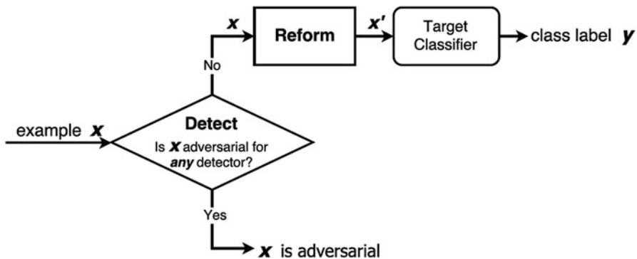
Fig. 11 The illustration of the MagNet work flow [20]
