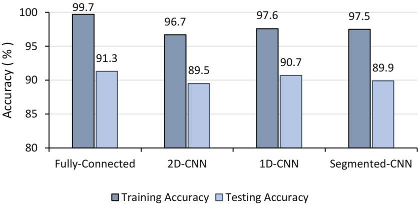
Fig. 9 Training and testing accuracy of different CNN architectures on the UNSW-NB15 data set. A fully-connected neural network was also analysed to provide a baseline comparison to the CNN techniques
