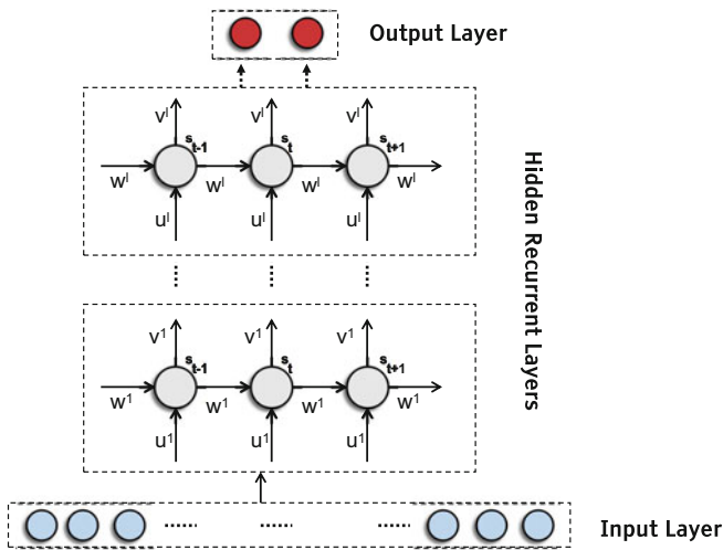
Fig. 5 Architecture of general RNN-based electricity theft detector
