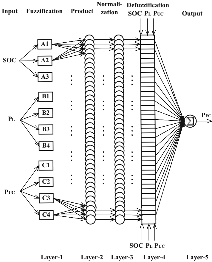
Fig. 3 Illustration of the proposed ANFIS implementation
