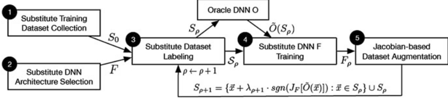
Fig. 8 Process of training substitute DNN and dataset augmentation [23]
