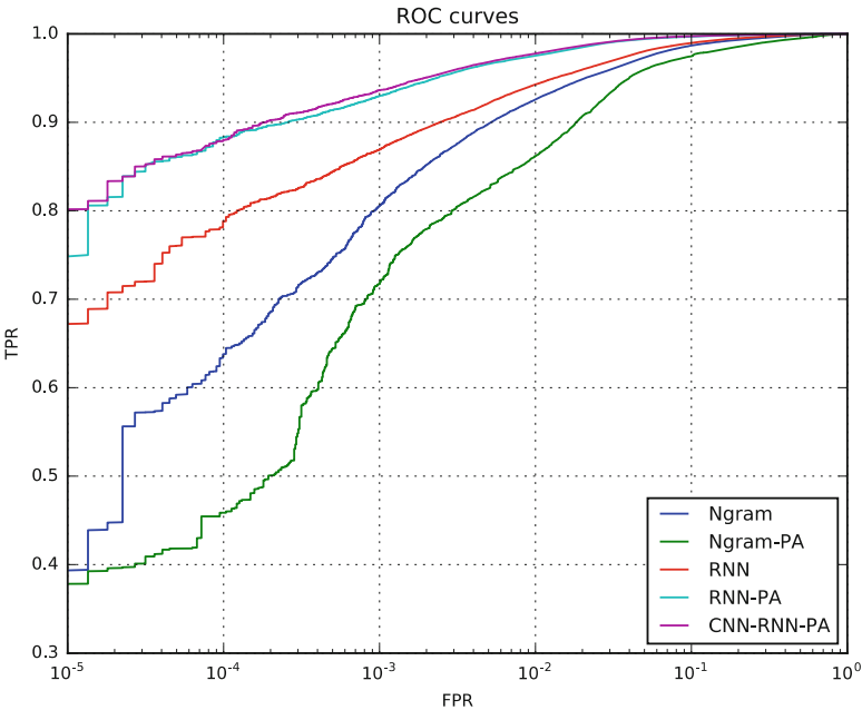
Fig. 4 ROC curves
