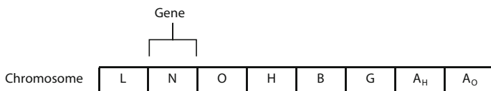
Fig. 6 Hyper-parameter chromosome
