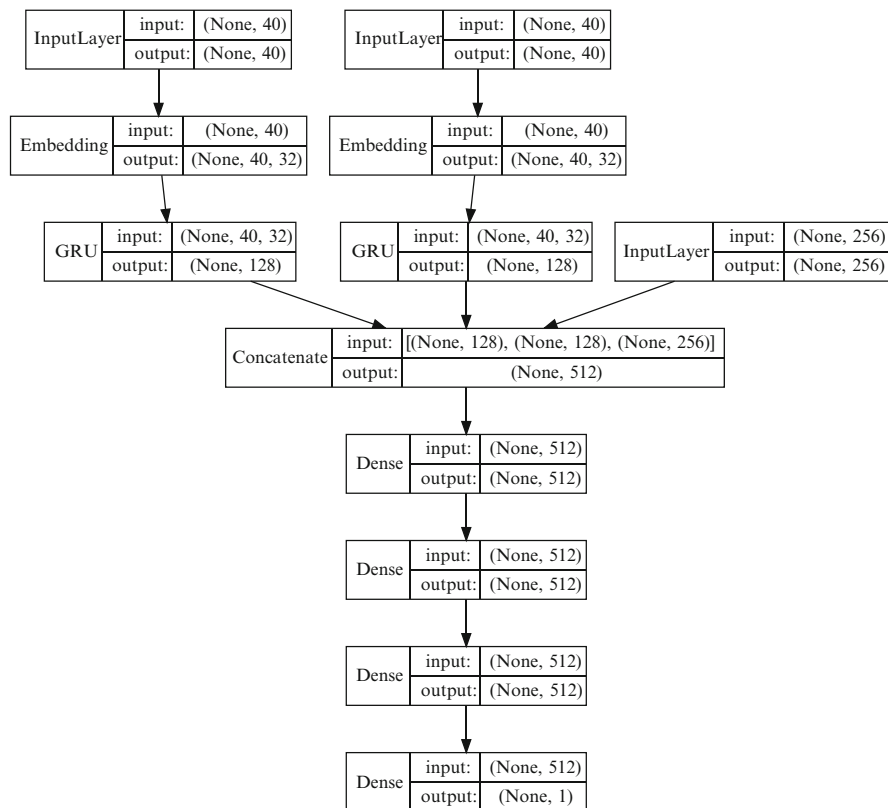
Fig. 3 The architecture of CNN-RNN model
