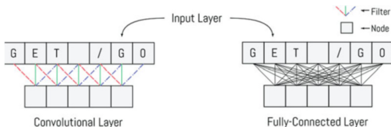
Fig. 2 A comparison of the connections in a convolutional layer versus a fully-connected layer. Each node in the convolutional layer makes the same three connections to the nodes in the input layer, albeit at different locations. This is known as a convolutional layer with a filter size of three. Each node in the fully-connected layer is connected to every node in the previous layer
