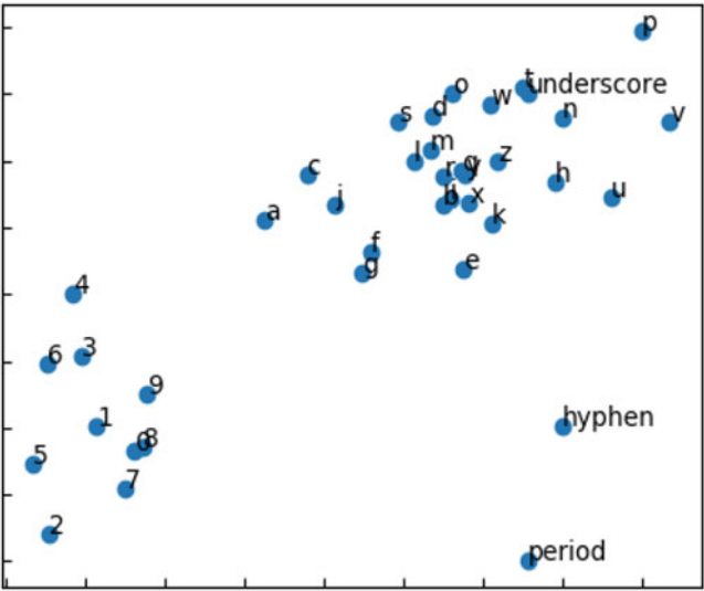
Fig. 4 Keras embedding character vector visualization of DBD model
