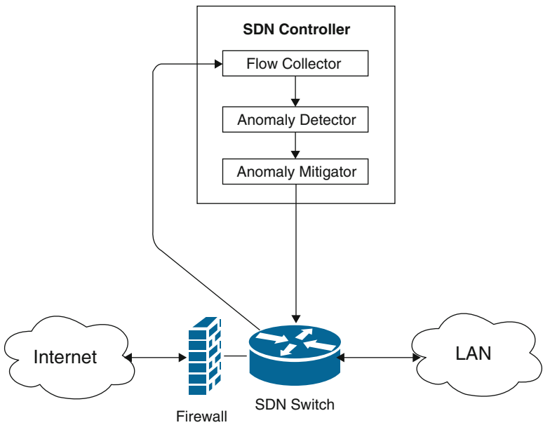
Fig. 2 SDN-based IDS architecture
