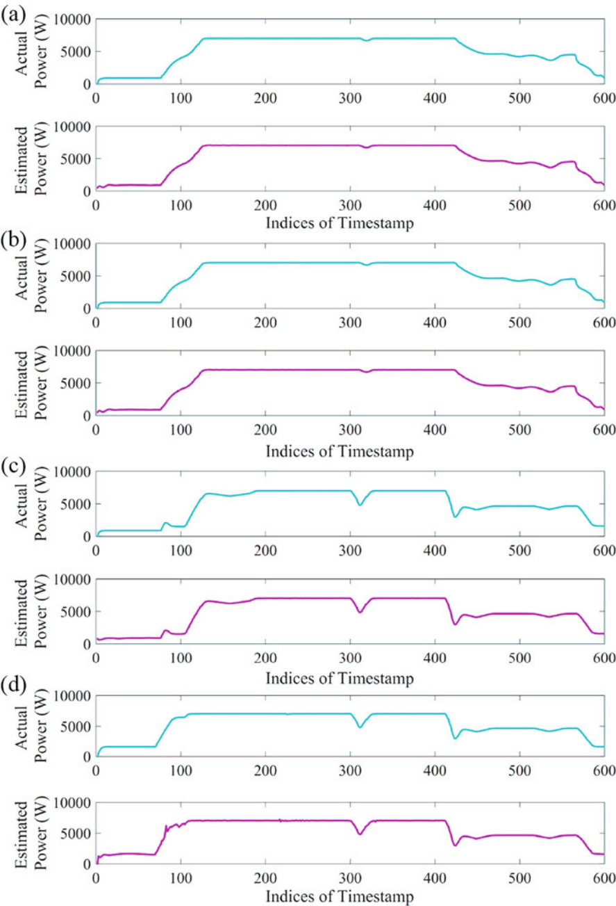
Fig. 8 Comparison results by considering, (a) state machine control; (b) frequency decoupling fuzzy logic control; (c) classical PI control; and (d) ECMS control strategies
