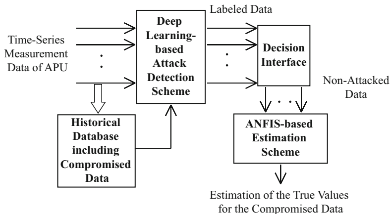
Fig. 1 Overview structure of our proposed security control architecture for hybrid emergency power system
