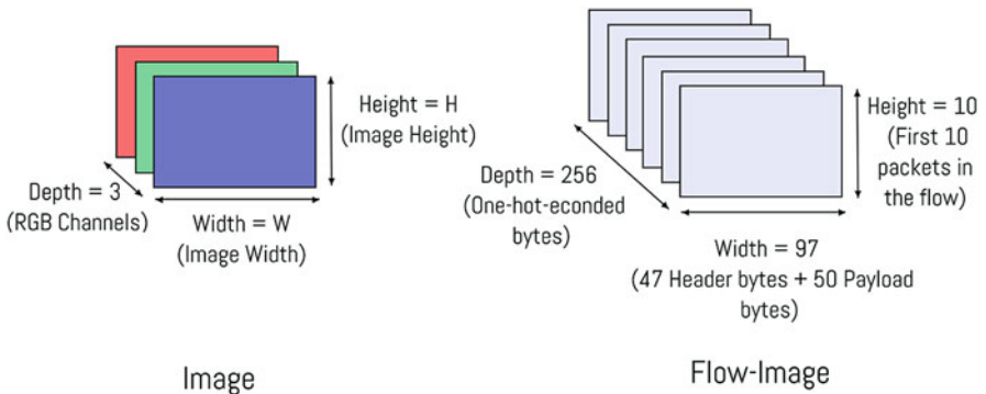
Fig. 3 Representation of an input used for image classification compared to Flow-Image
