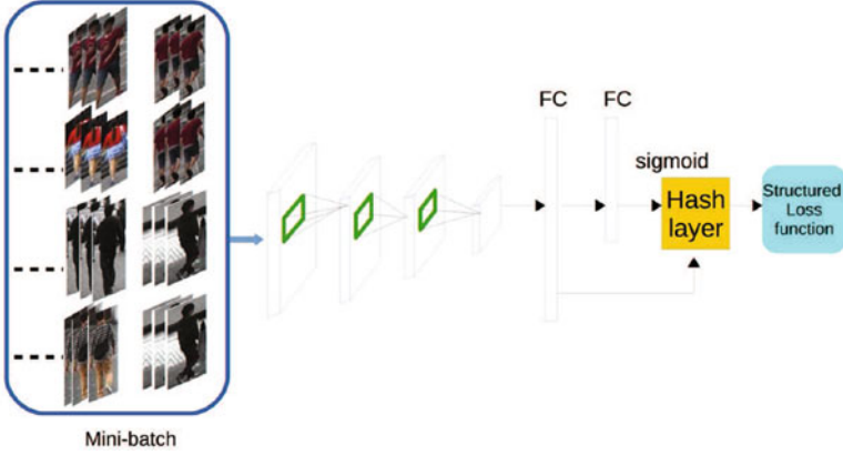
Fig. 5 Overview of the deep hashing framework for person re-identification. The deep neural network takes a feed-forward, back-propagation strategy to learn features and hash codes simultaneously. During the feed-forward stage, the network performs inference from a mini-batch. The mini-batch is put through a stack of convolutional layers to generate nonlinear yet discriminative features, which are subsequently mapped to output feature vectors by fully-connected layers (FC). Meanwhile, a hash function layer is introduced atop of FC layer to learn hash codes that are optimized by a structured loss function to preserve their similarities/dissimilarities. In back-propagation, parameters are updated by computing their Stochastic Gradient Decent (SGD) w.r.t. the mini-batch
