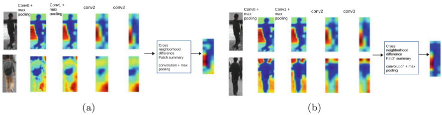
Fig. 4 Feature responses of each layer learned by the PersonNet network. (a) A pair of negative images. (b) A pair of positive images
