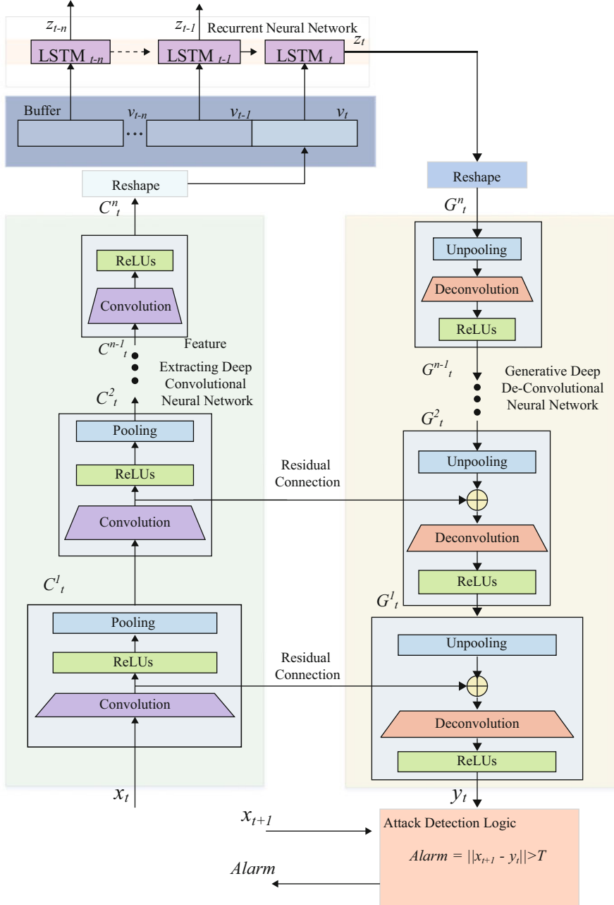
Fig. 2 Proposed architectures for our proposed deep learning-based cyber-attack detection scheme, where C_t^n is the output of the n th CNN at time t , G_t^n is the input for the n th generative DCNN, and ReLU block represent a layer of units with rectifier activation function
