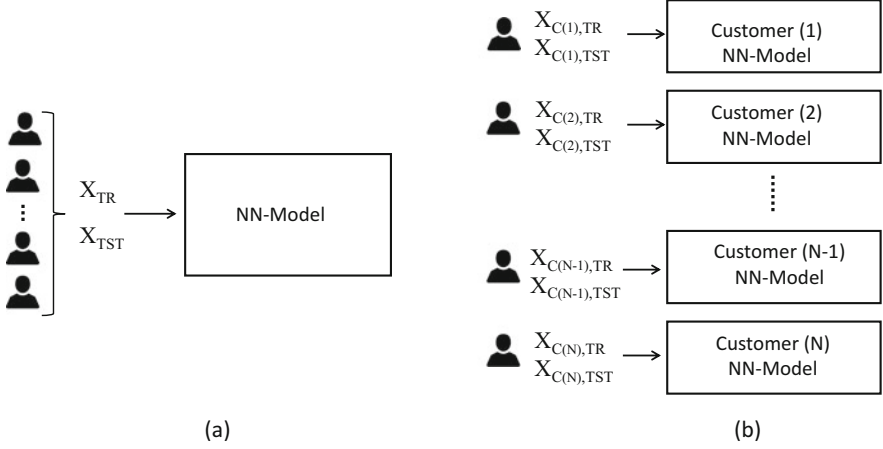
Fig. 1 Generalized versus customer-specific model. (a) Generalized NN-model. (b) Customer-Specific NN-model
