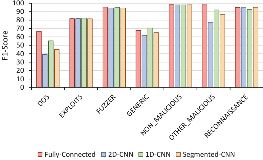
Fig. 10 F1-Score of the individual classes for each classifier on the testing set
