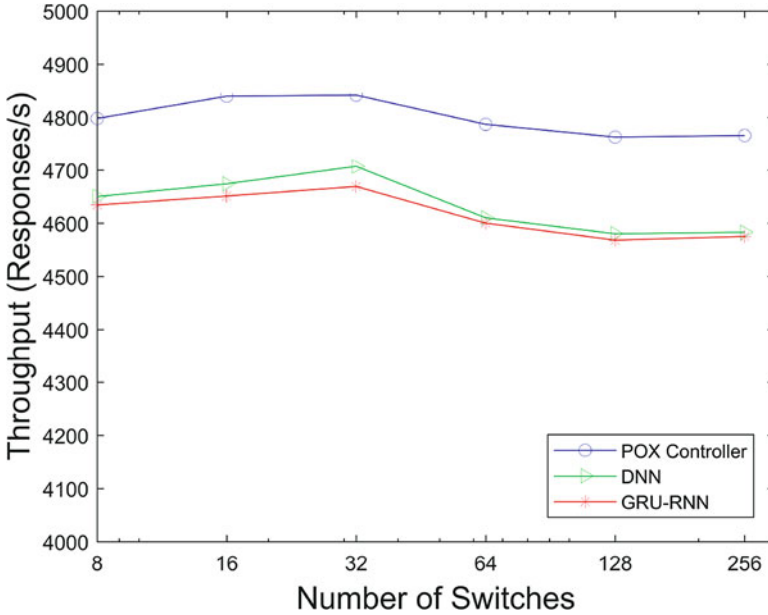
Fig. 6 Throughput evaluation
