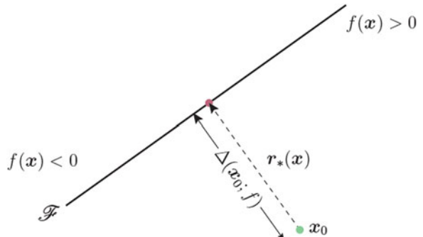
Fig. 7 Computation of the minimal perturbation for linearized binary classifier [21]
