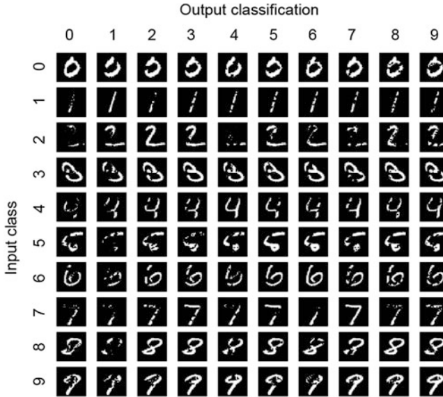
Fig. 6 Original samples and generated Adversarial samples on the MNIST dataset. The rows indicate original input classes and columns indicate target classes [24]
