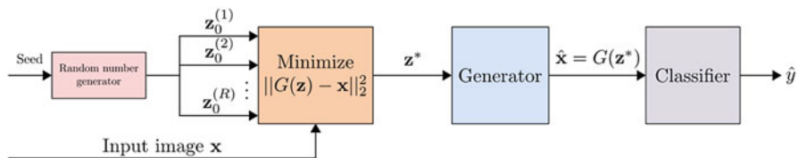
Fig. 12 Overview of the Defense-GAN algorithm [27]
