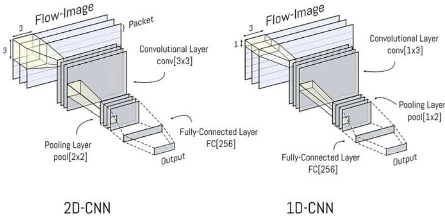
Fig. 4 Structure of a 2D-CNN and 1D-CNN. The filters of a 2D-CNN span multiple packets, while a 1D-CNN’s filters only consider the bytes of a single packet. Only the first convolutional, pooling, and fully-connected layers in the 2D-CNN and 1D-CNN are shown
