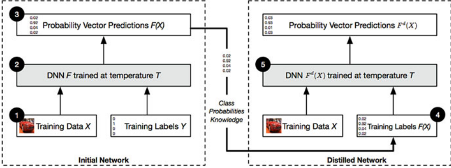
Fig. 10 The process of training a distilled neural network [25]
