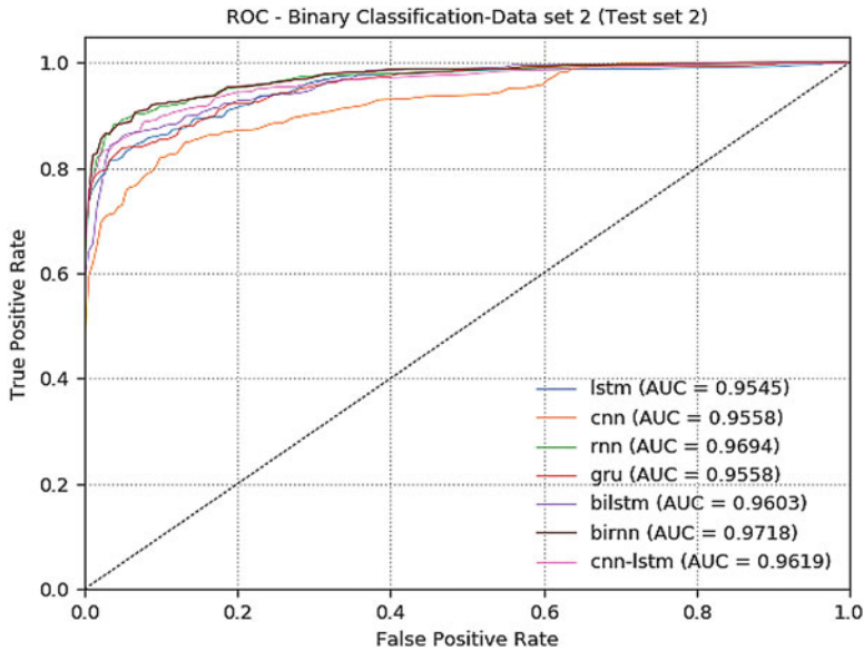
Fig. 5 ROC curve of binary class testing for dataset 2
