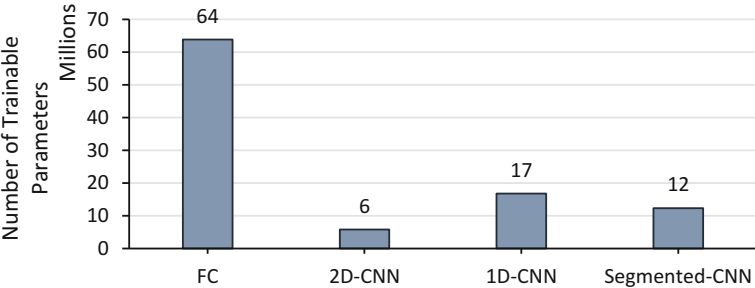
Fig. 6 Number of trainable parameters in each neural network to the nearest million
