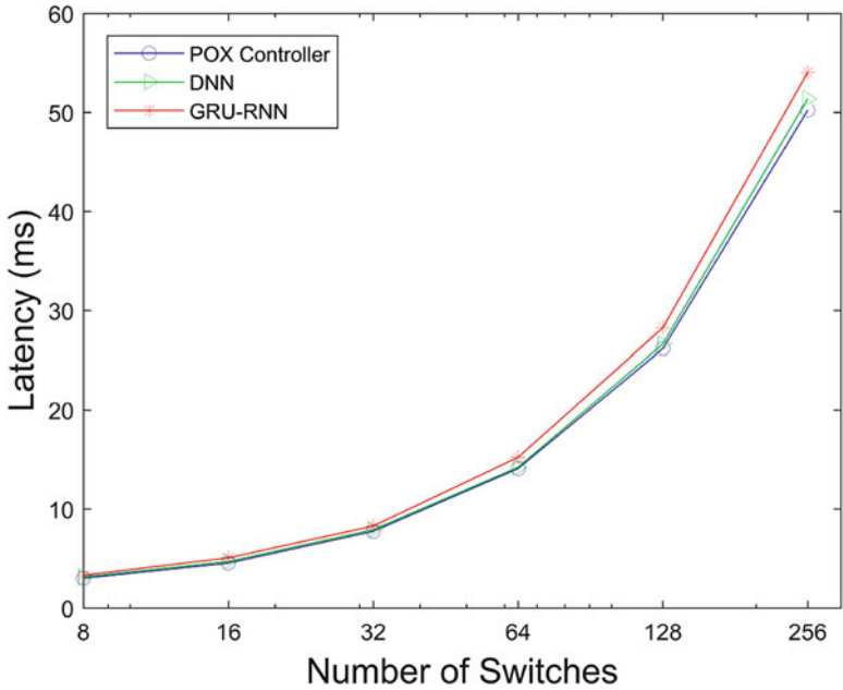
Fig. 7 Latency evaluation
