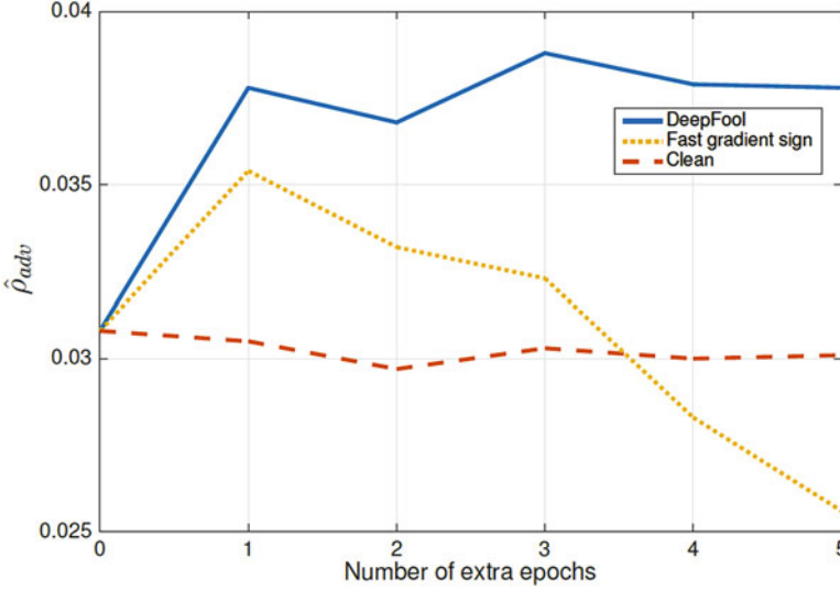
Fig. 9 Evolution of the model robustness for LeNet on CIFAR-10 dataset through the epochs [21]
