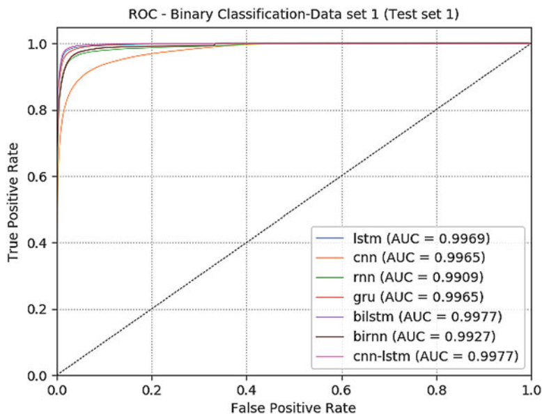
Fig. 4 ROC curve of binary class testing for dataset 1
