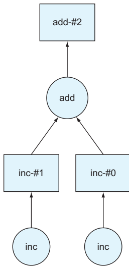
Figure 2.4 A visual representation of the DAG produced in listing 2.6
