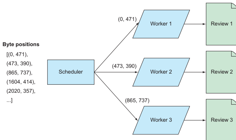
Figure 9.6 Mapping the parsing code to the review data
