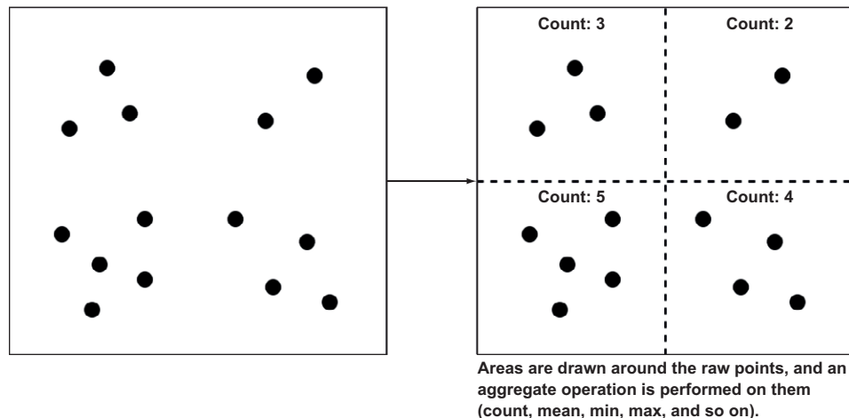
Figure 8.3 Aggregation draws areas around the raw points and performs an aggregate operation on the areas; each of these areas resembles a single pixel in the final visualization.
