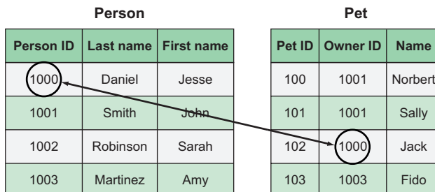
Figure 5.10 We can tell that Jack is my cat because his Owner ID is a key that points to my Person ID.
