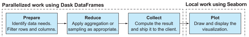
Figure 7.5 The prepare-reduce-collect-plot pattern for visualizing large datasets with Dask
