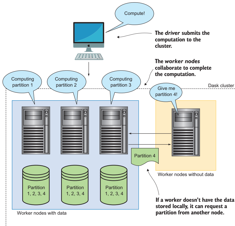
Figure 4.9 Shipping computations to the data
