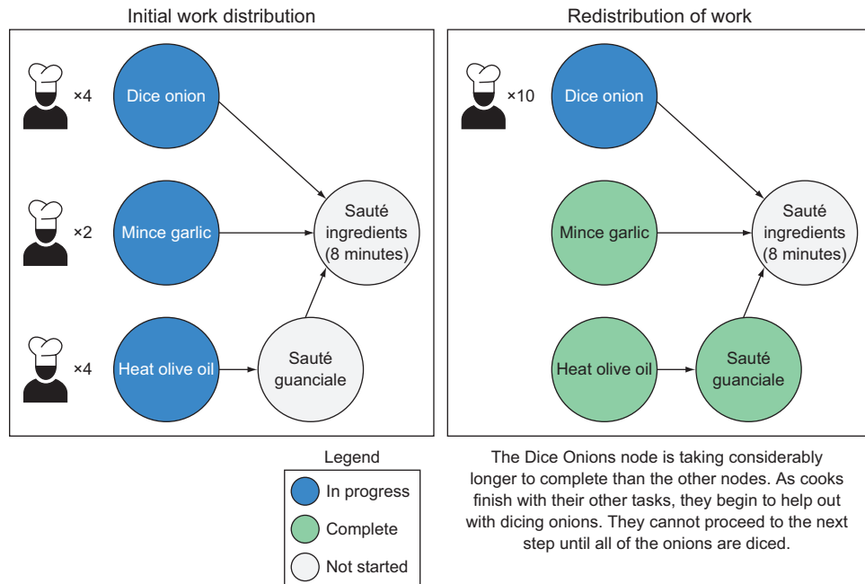
Figure 1.8 A graph with nodes distributed to many workers depicting dynamic redistribution of work as tasks complete at different times
