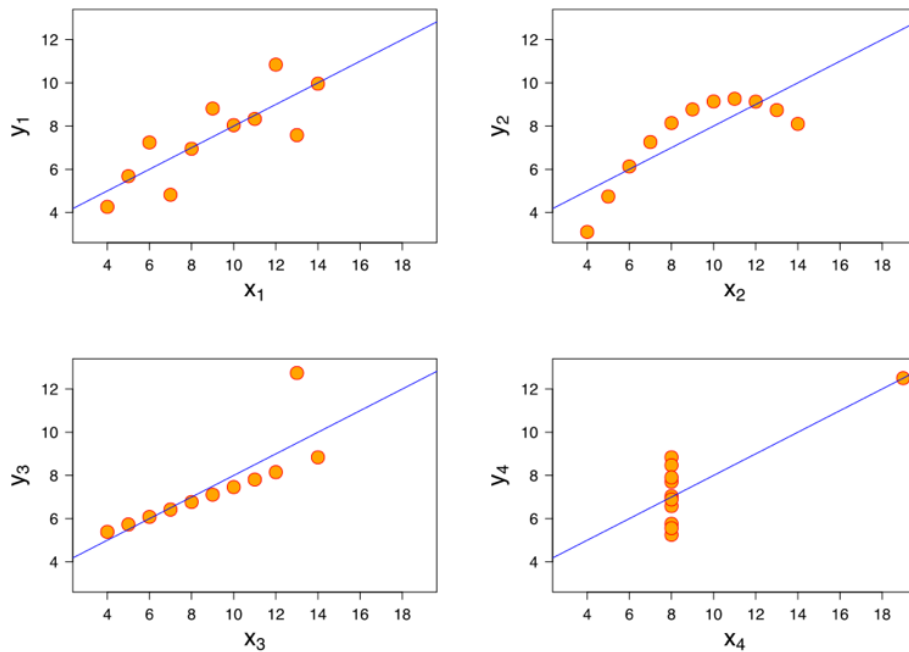
Figure 7.1 Anscombe's quartet highlights the importance of using visualization for effective data analysis.
