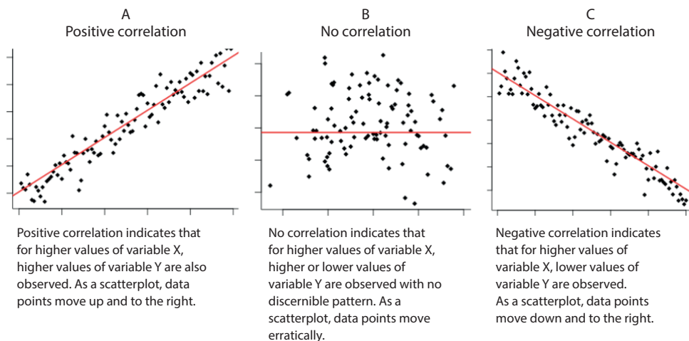
Figure 6.6 A visual guide to correlation
