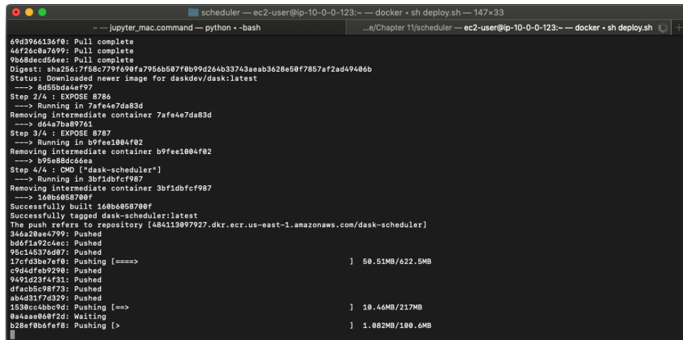
Figure 11.35 Building the dask-scheduler image
