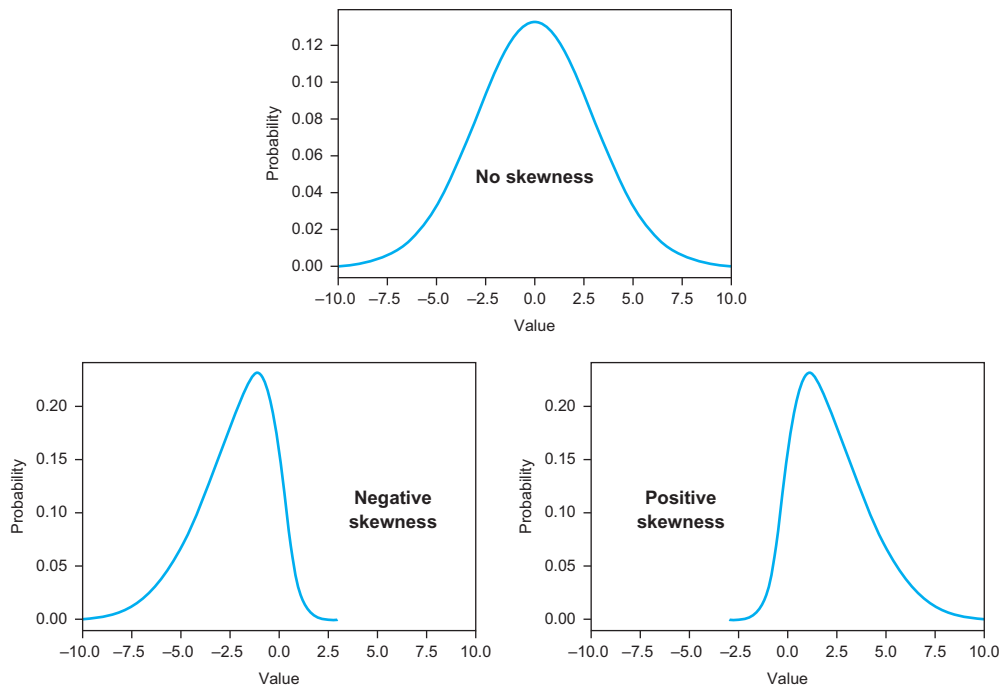
Figure 6.4 A visual comparison of skewness
