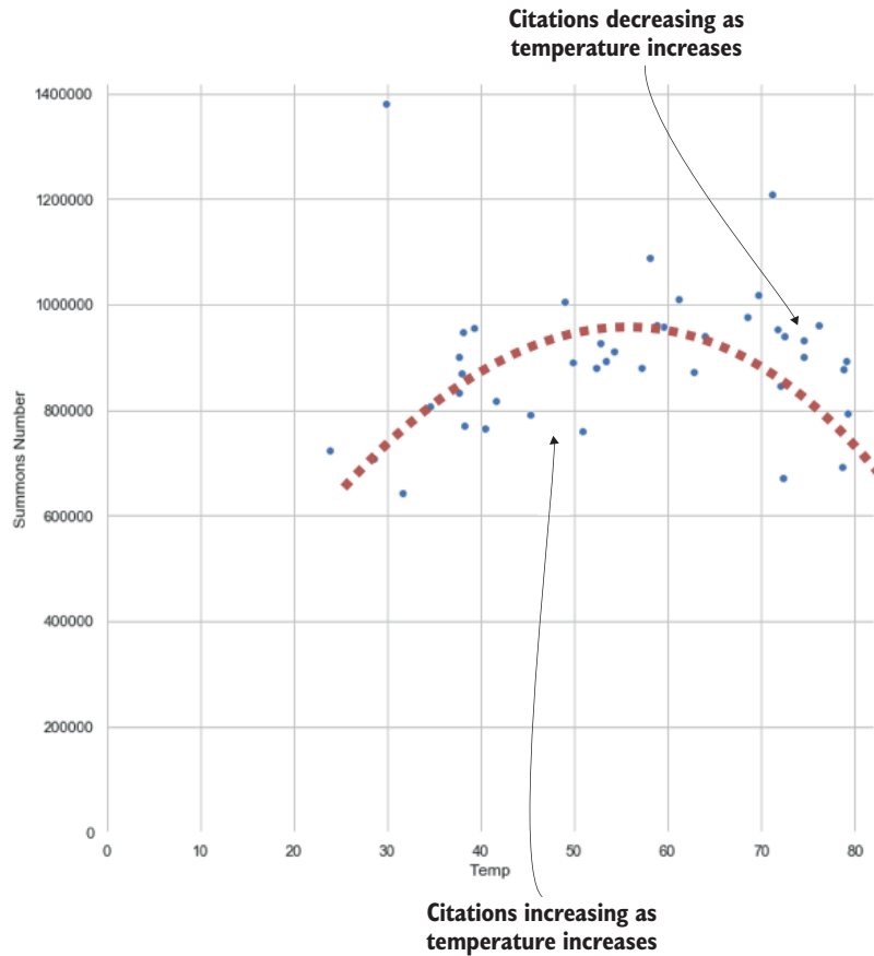
Figure 7.8 The relationship appears to be non-linear; the relationship changes direction around 60 degrees.
