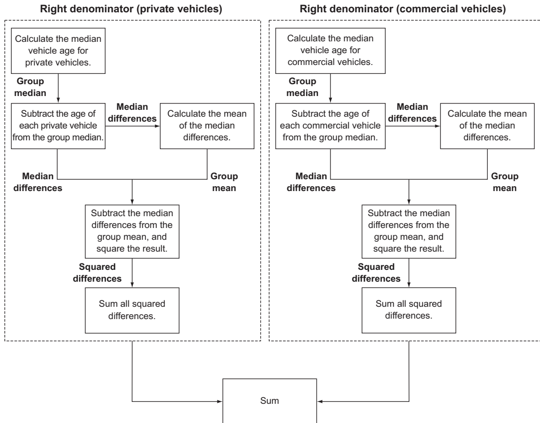
Figure 6.14 The process for calculating the right denominator
