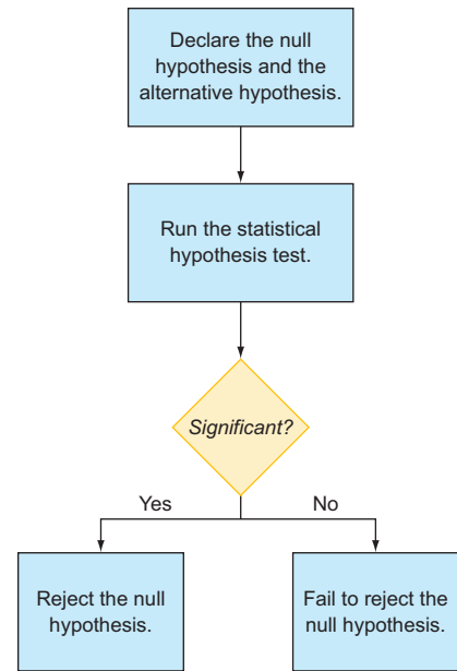
Figure 6.10 The process of statistical hypothesis tests
