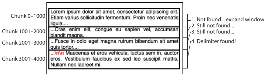
Figure 9.5 A visual representation of the recursive delimiter search function
