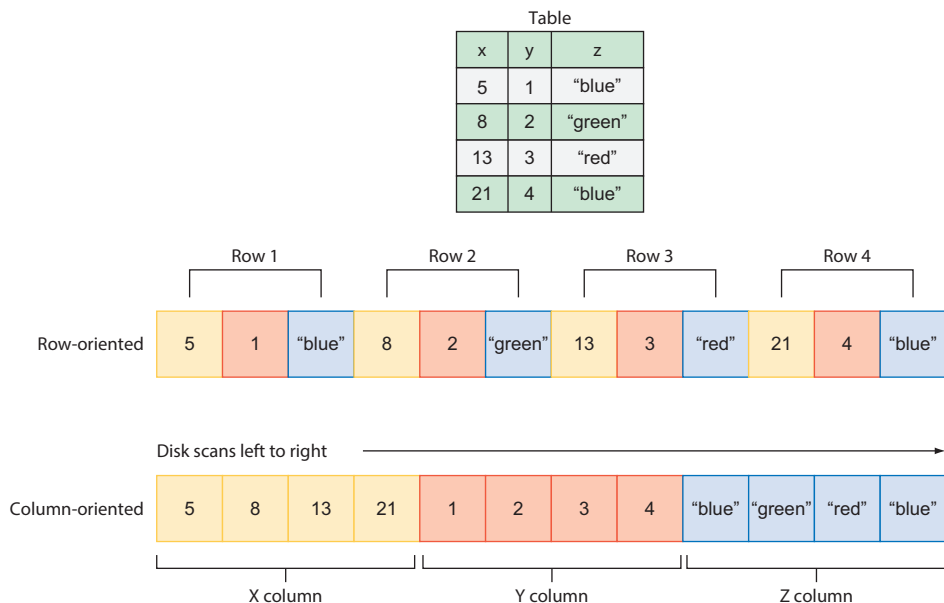
Figure 4.10 The structure of Parquet compared with delimited text files
