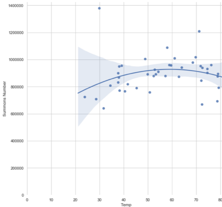
Figure 7.9 The scatterplot of average temperature vs. count of citations fit with a nonlinear curve
