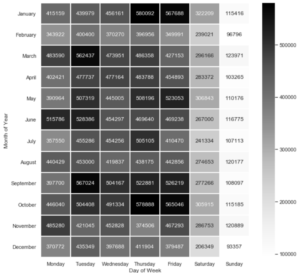
Figure 7.13 A heatmap of citations issued by day of week and month of year
