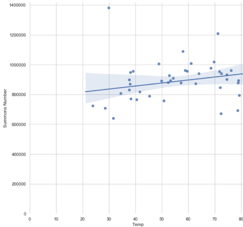
Figure 7.7 The scatterplot of average temperature vs. count of citations with an added regression line
