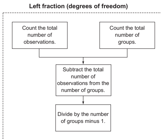
Figure 6.13 The first part of the Brown-Forsythe test
