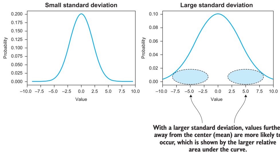
Figure 6.3 A comparison of standard deviation
