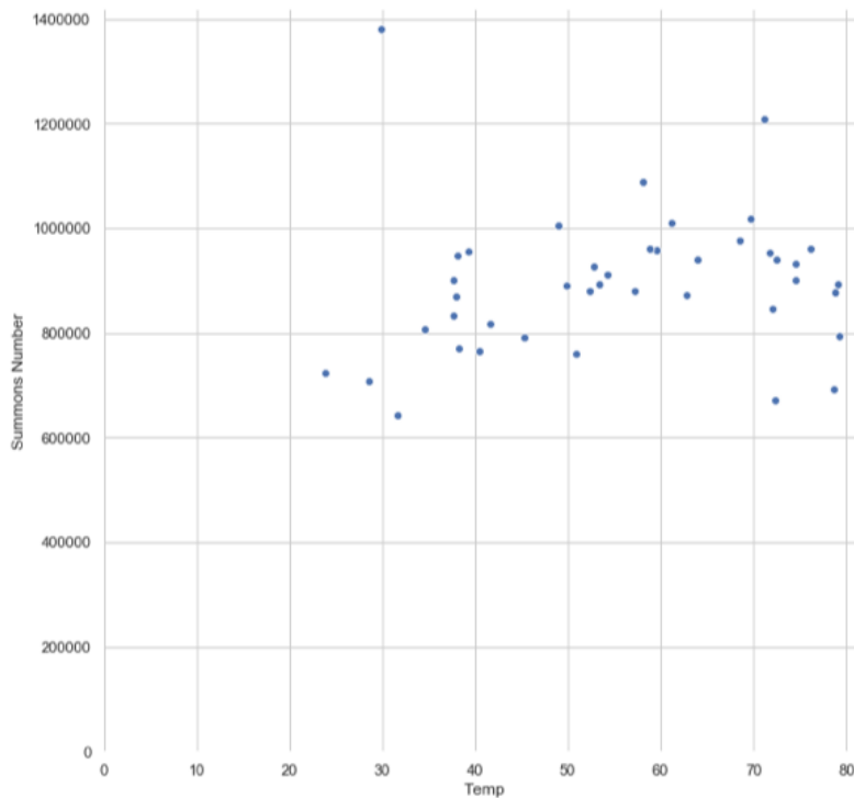
Figure 7.6 A scatterplot of average temperature vs. number of citations
