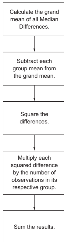
Figure 6.16 The process to calculate the right numerator of the Brown-Forsythe equation
