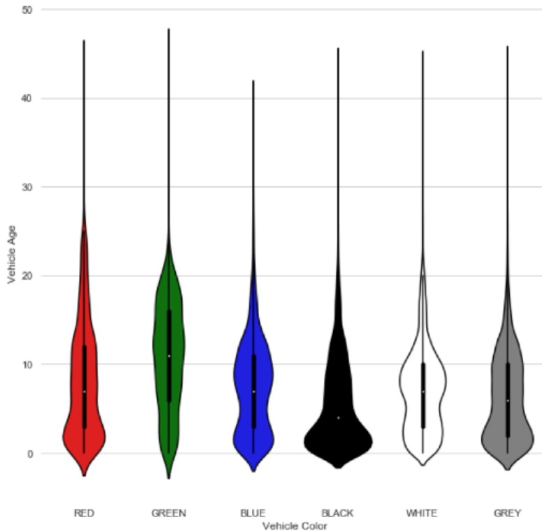
Figure 7.12 A violinplot of the random sample
