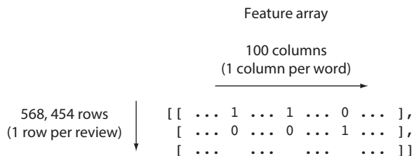
Figure 10.5 The shape of the feature array
