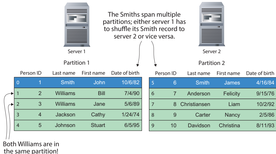
Figure 3.6 A GroupBy operation that requires a shuffle
