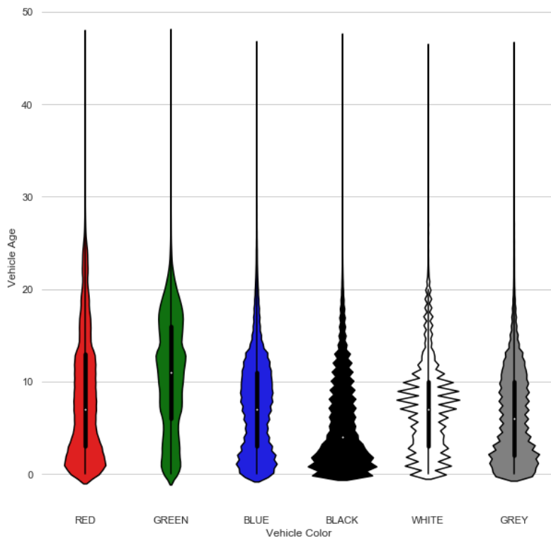
Figure 7.11 A violinplot of vehicle color vs. vehicle age
