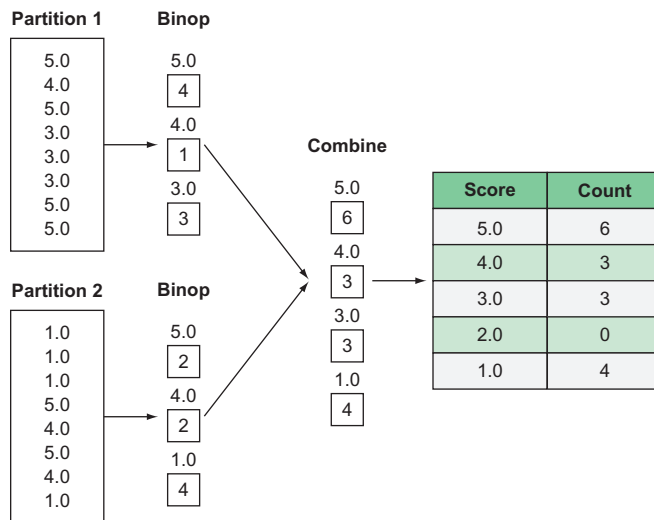
Figure 9.7 An example of a fold operation
