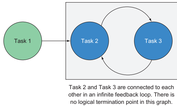
Figure 1.4 An example of a cyclic graph demonstrating an infinite feedback loop
