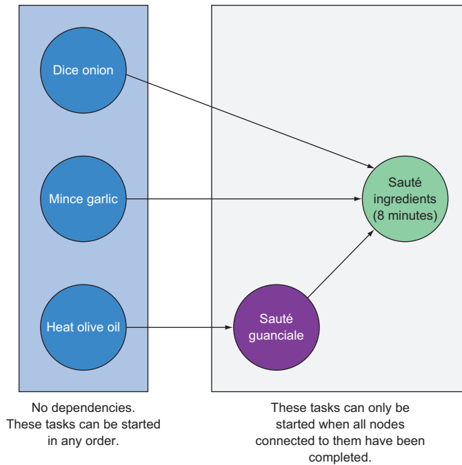
Figure 1.3 A graph displaying nodes with dependencies
