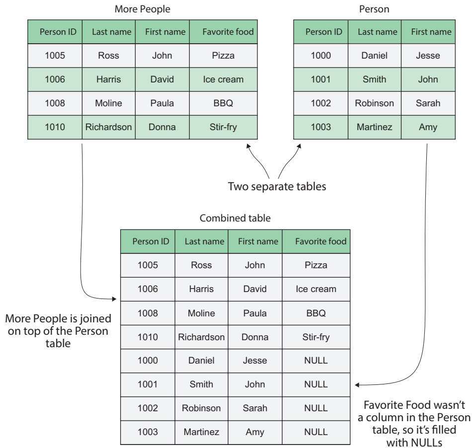
Figure 5.15 The result of concatenating the Person and More People tables
