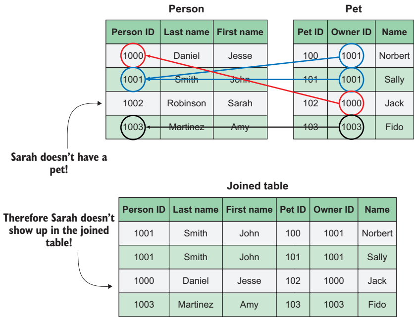
Figure 5.11 Showing all the key relationships between the Person and Pet tables
