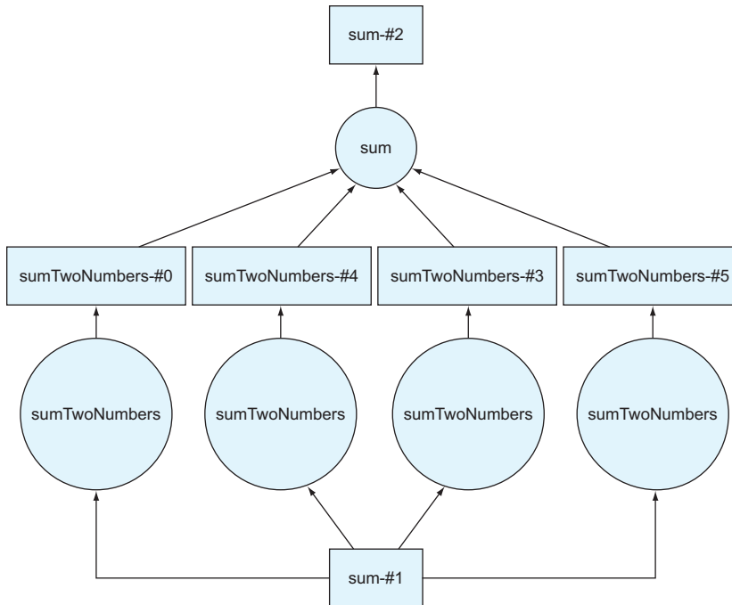
Figure 2.10 The DAG generated by listing 2.11
