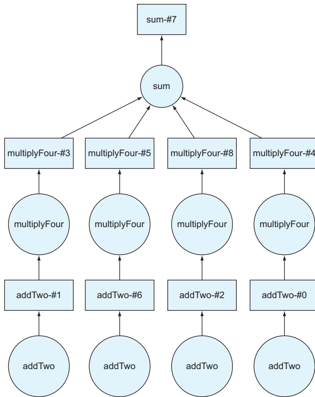
Figure 2.7 The DAG including the multiplyFour step
