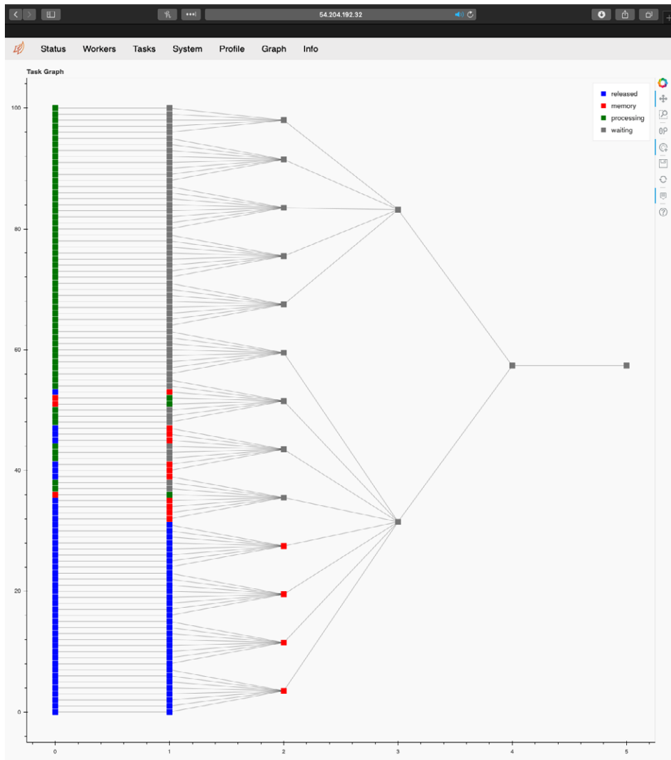
Figure 11.55 Real-time DAG view
