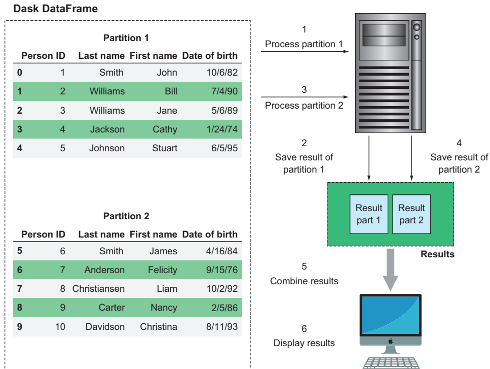
Figure 2.3 Dask splits large data files into multiple partitions and works on one partition at a time.
