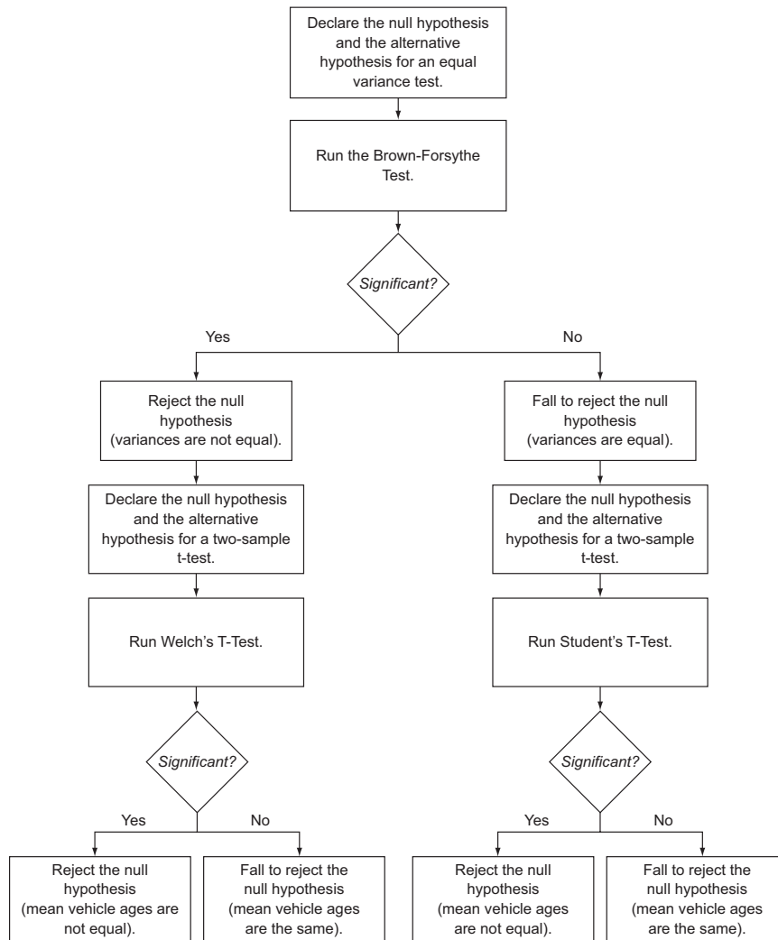
Figure 6.11 The process we will use to determine if mean vehicle age has any relationship with vehicle type
