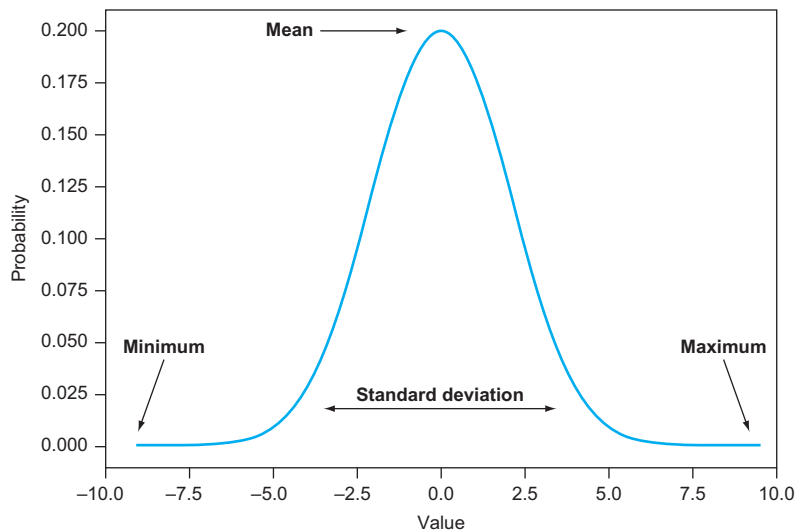
Figure 6.2 A visual guide to descriptive statistics
