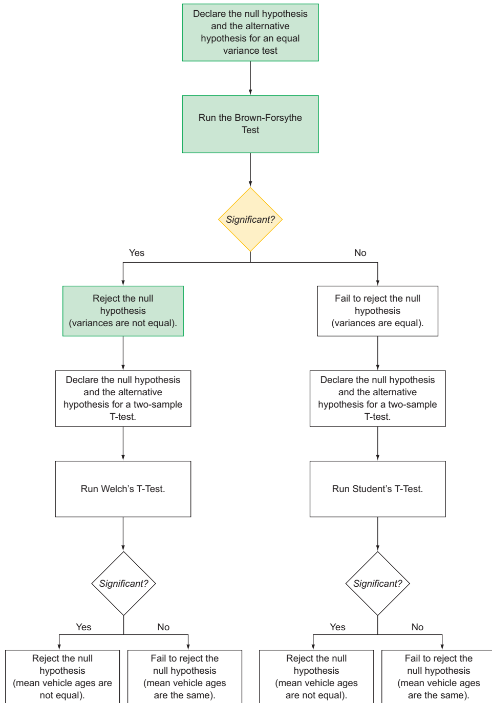
Figure 6.17 We've rejected the null hypothesis of the Brown-Forsythe test, so we will next run Welch's T-Test.
