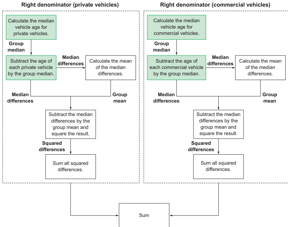
Figure 6.15 Our progress so far calculating the right denominator of the Brown-Forsythe equation
