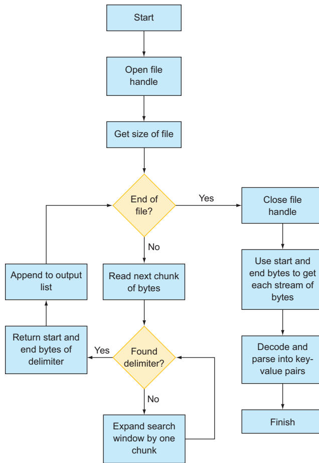
Figure 9.4 Our custom text-parsing algorithm to implement using Dask Delayed
