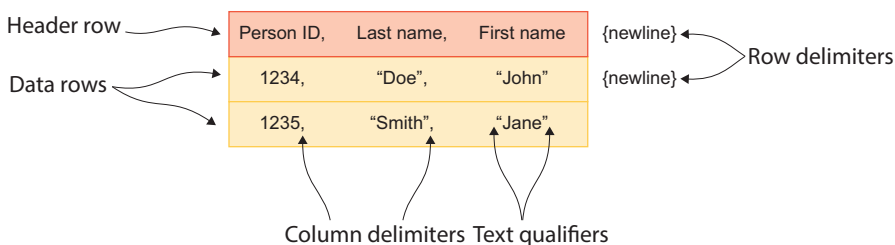
Figure 4.2 The structure of a delimited text file
