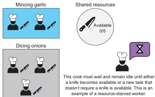
Figure 1.9 An example of resource starvation
