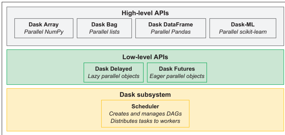
Figure 10.2 A review of the API components of Dask
