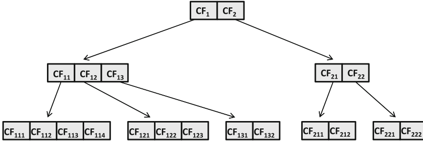
Figure 7.1: The CF-Tree
