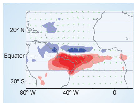
Figure 1 Determinants of present-day drought years in northeastern Brazil. An anomalous north–south gradient in ocean surface temperatures near the Equator (not shown), with warmer conditions in the north, drives a low-level atmospheric circulation, shown by arrows, that strengthens the trade winds in the southern Atlantic and weakens them in the north. The result is to impede the southward migration of the Atlantic Intertropical Convergence Zone, which increases rainfall in the northern tropical Atlantic (blue) and reduces it in the southern tropical Atlantic and northeastern Brazil (red). The opposite set of conditions, persisting over several centuries, is thought to characterize the wet episodes identified by Wang et al. 2 .
