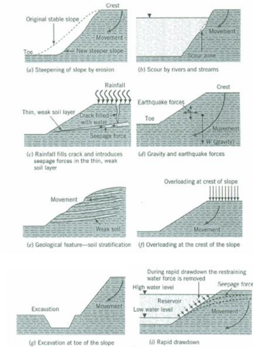
Figure 5.2: Some causes of slope failure (Budhu, pp. 526)
