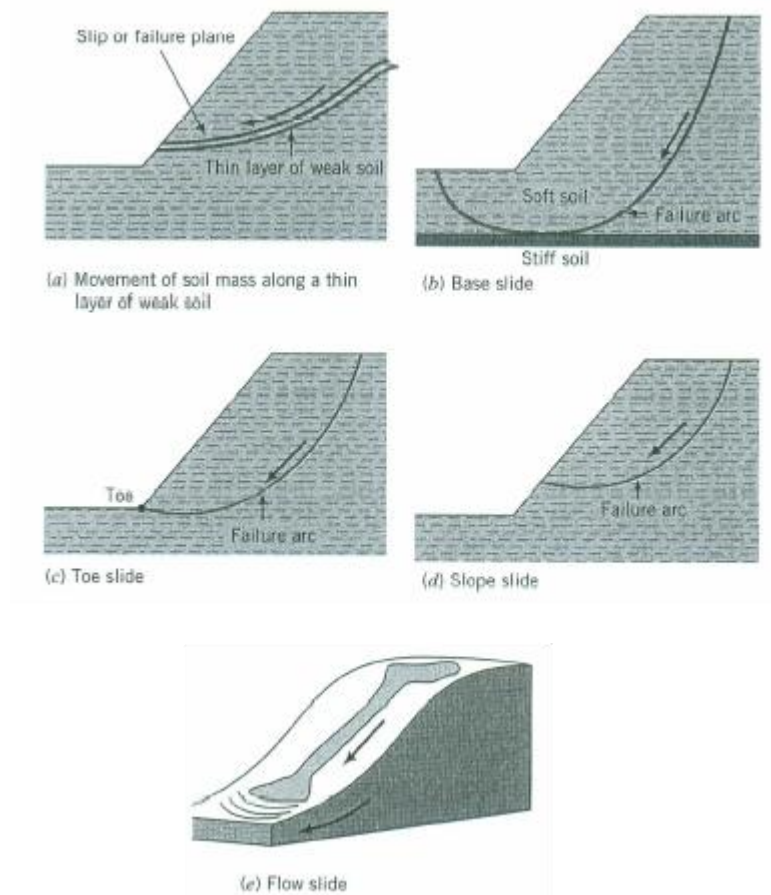
Figure 4.1: Some types of slope failure (Budhu, pp. 524)
