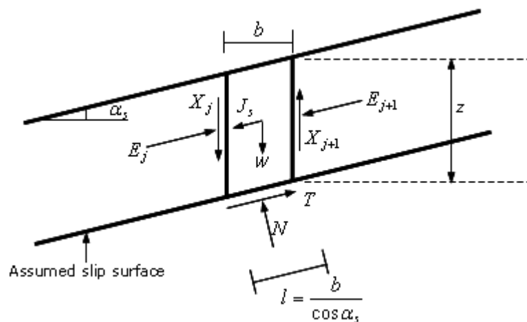
Figure 4.3: Forces on a slice of soil in an infinite slope.
