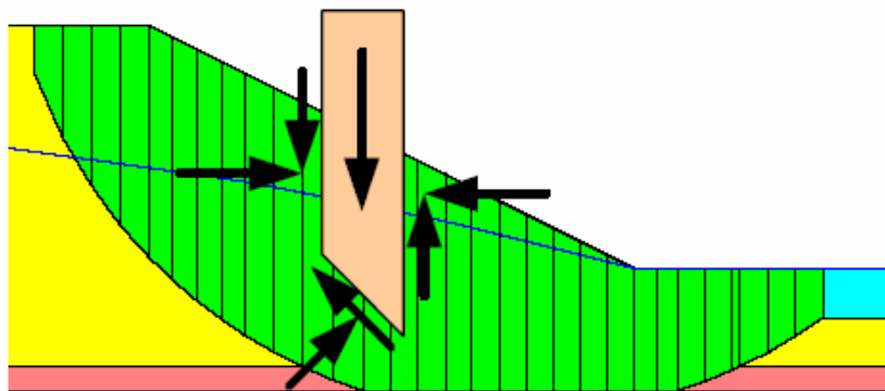
Figure 4.5: Slice discretization and slice forces in a sliding mass.
