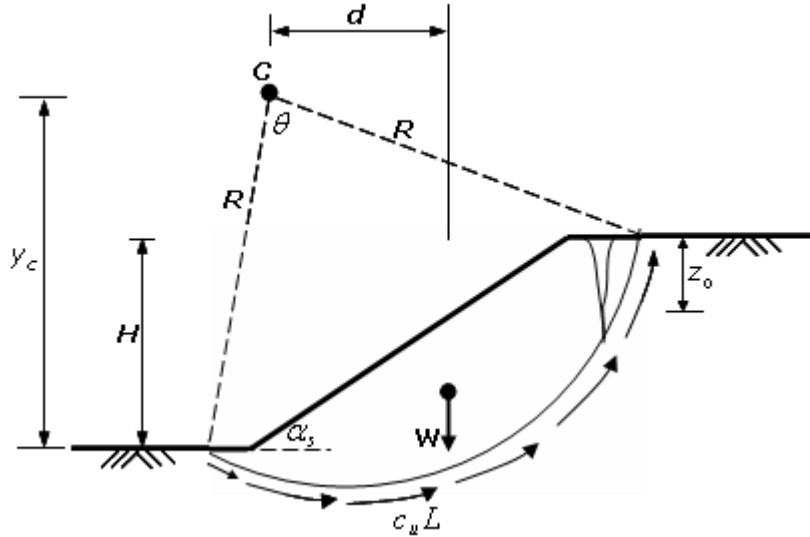
Figure 4.4: Slope failure in c_u, \phi_u = 0 .
