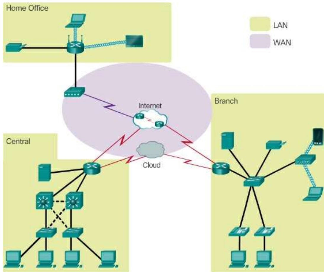
Figure 1-15 LANs and WANs
