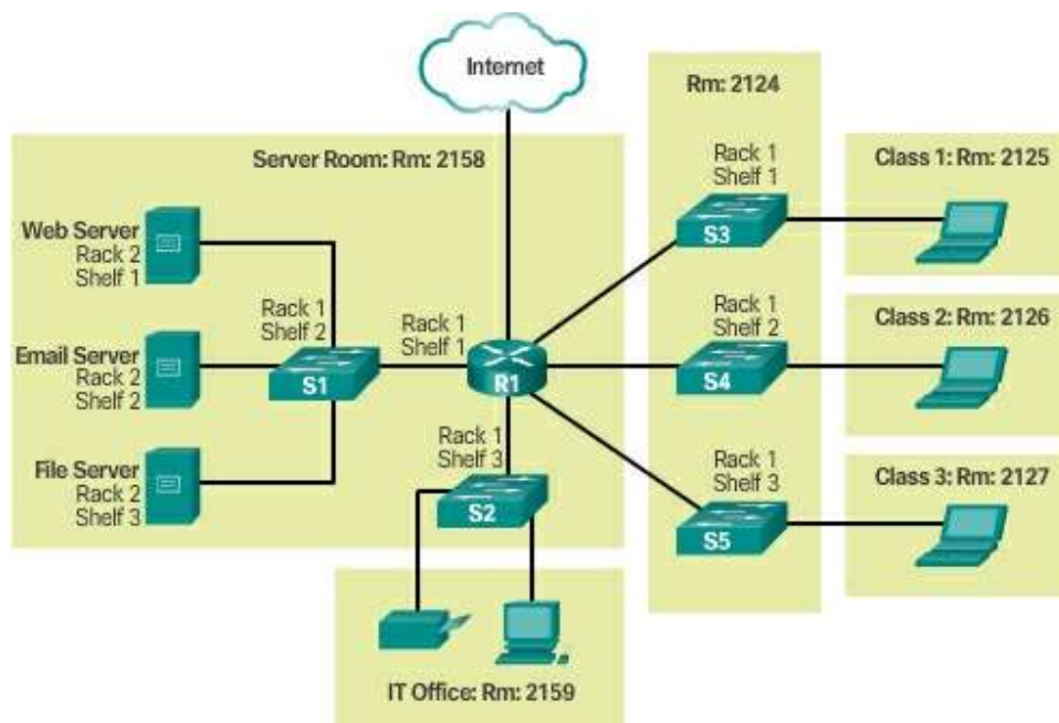
Figure 1-13 Physical Topology
