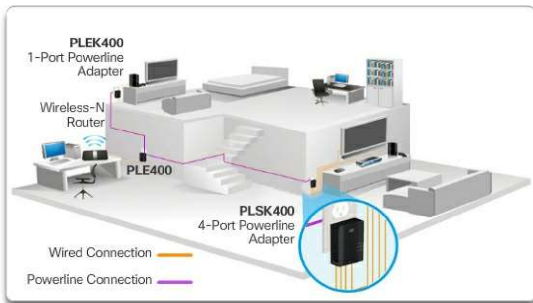
Figure 1-32 Powerline Networking
