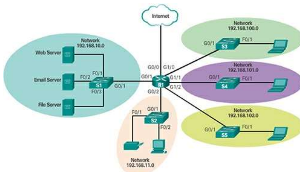
Figure 1-14 Logical Topology
