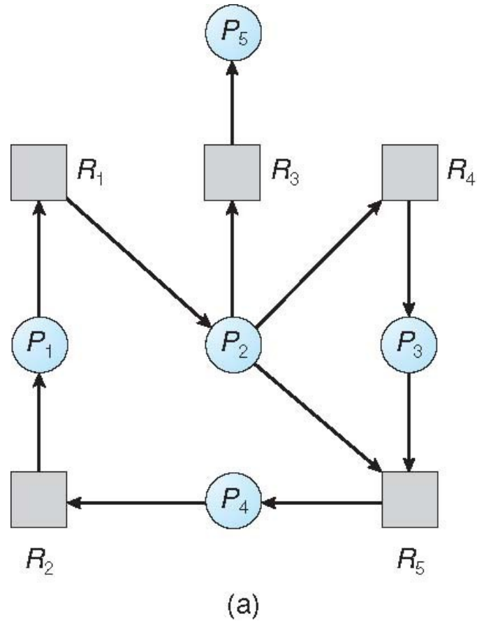
Resource-Allocation Graph
