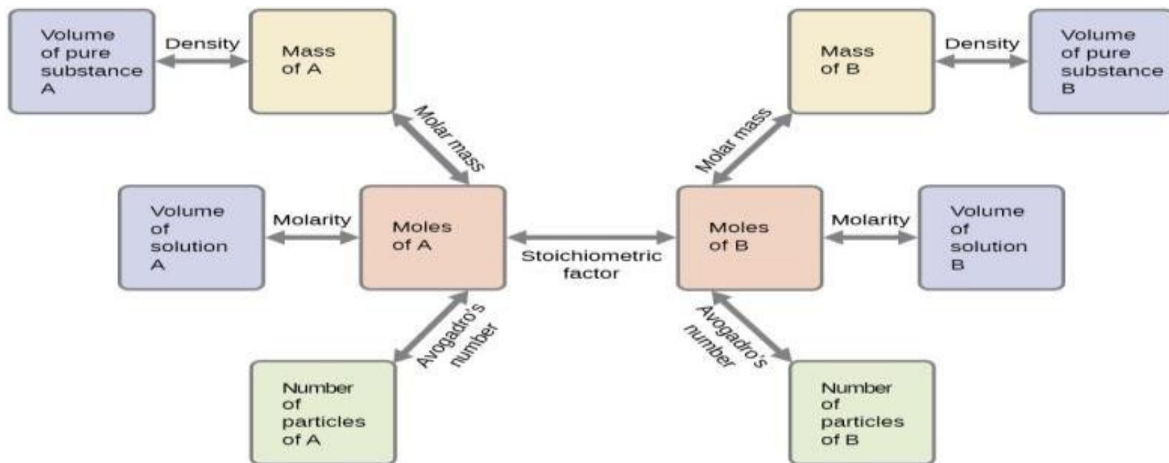
Figure : The flowchart depicts the various computational steps involved in most reaction stoichiometry calculations.
