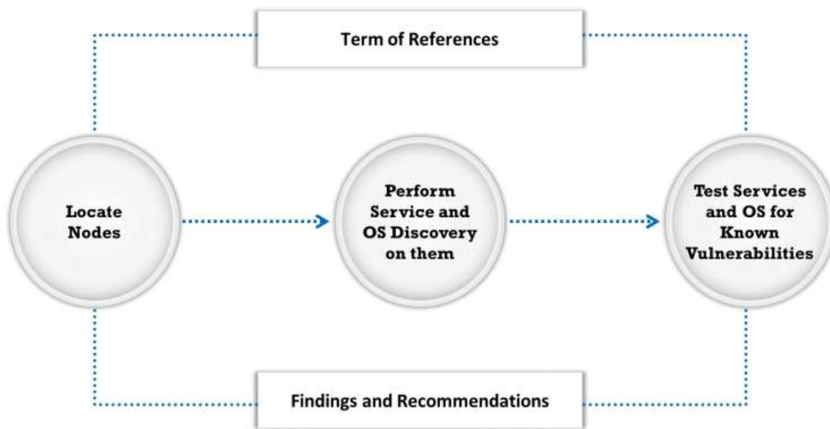
Figure 5.5: The working of vulnerability scanning solutions
