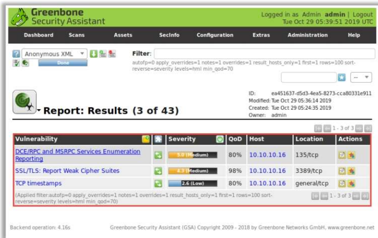
Figure 5.9: Vulnerability scanning using OpenVAS
