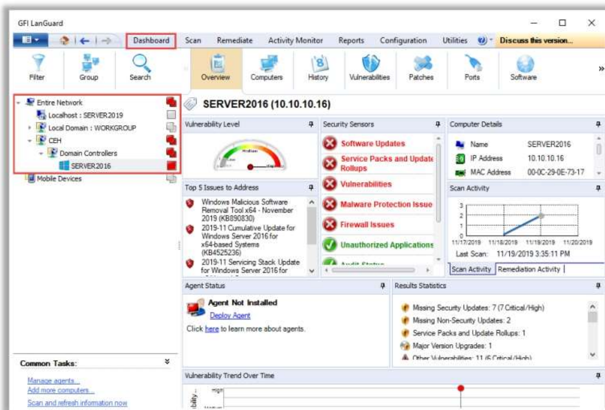
Figure 5.8: Vulnerability scanning using GFI LanGuard
