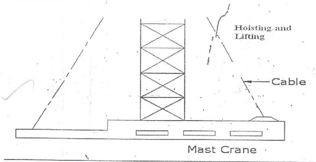
Hoisting of columns
