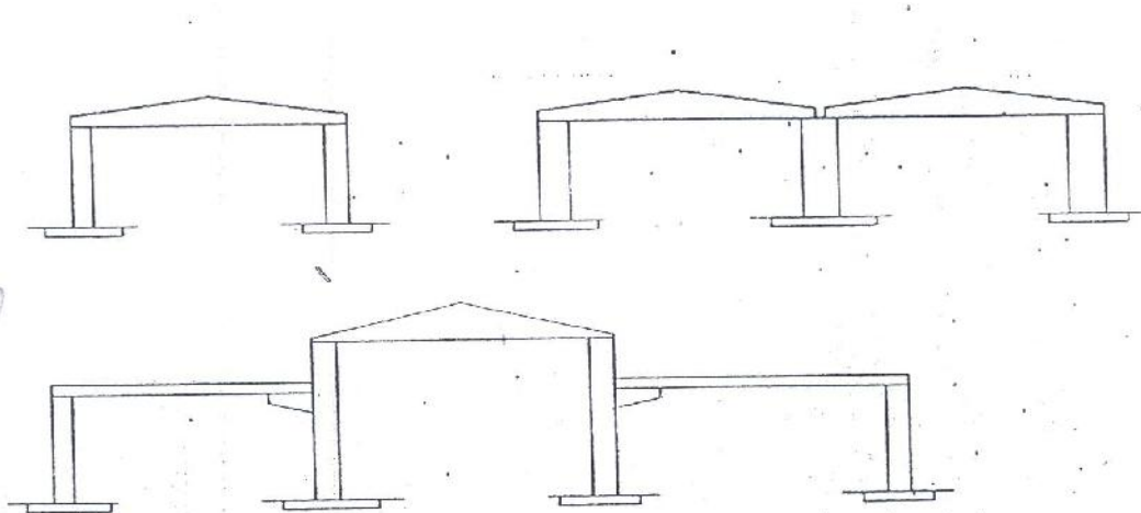
Fig 1.2.Members of frame disunited at the joints
