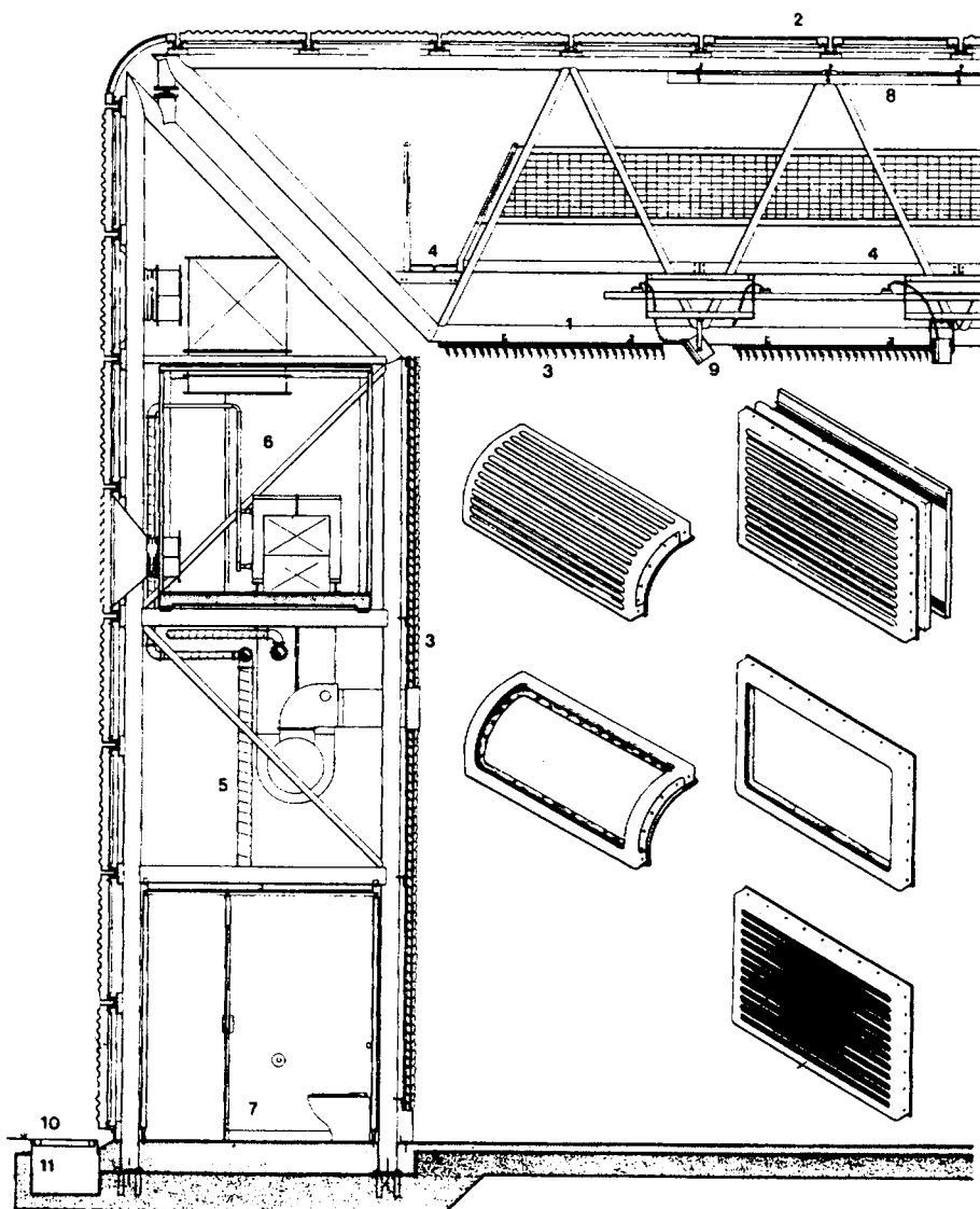
11.09 Foster Associates, Sainsbury Centre for the Visual Arts, University of Norwich, England, 1977. Wall Section.
