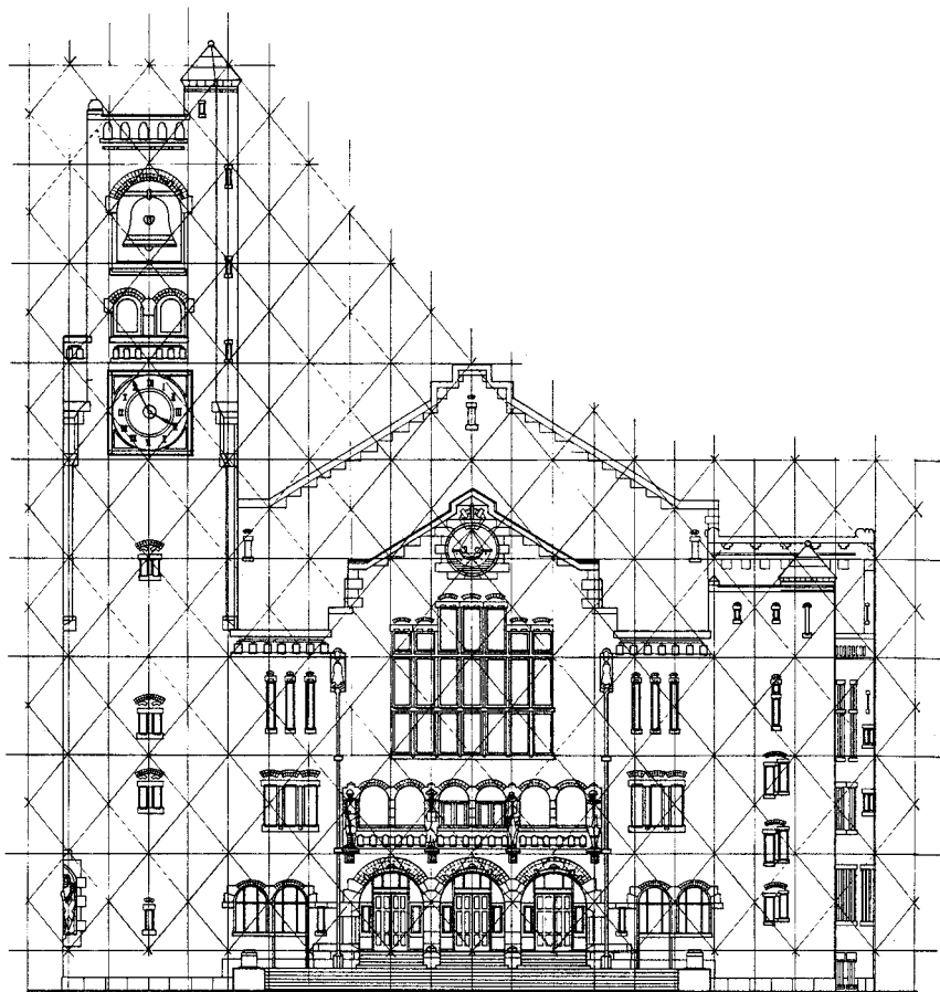
11.05 H.P. Berlage, Stock Exchange, Amsterdam, 1897–1903. South elevation with the system of proportions (1998 drawing).
