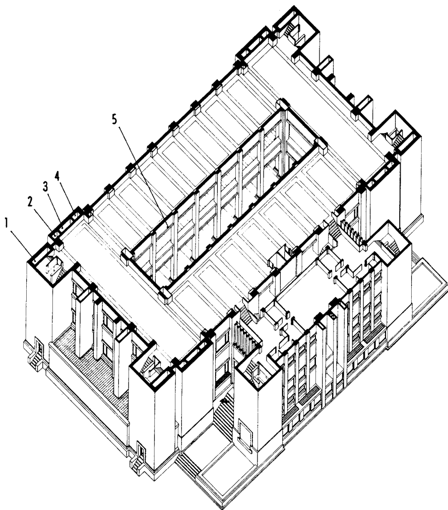
11.06 Frank Lloyd Wright, Larkin Building, Buffalo, 1904. Axonometric at third floor level. Note the service ducts built into the walls of the stair shafts. Numbers indicate built-in services according to the following key: 1. fresh-air intake; 2. utilities; 3. foul air exhaust; 4. miscellaneous ducts and services; 5. tempered air outlets under balcony fronts and ceiling beams.
