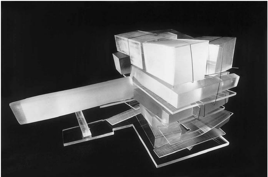
13.17 Boilerhouse Competition, V&A Museum, London: massing model. © Zaha Hadid.
