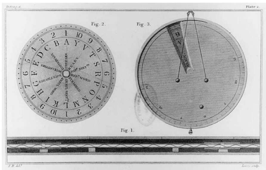
8.05 Text discs and subterranean cable, from R. Ronalds, Descriptions of an Electrical Telegraph , 1823.
