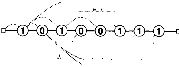
Figure 19.3 Finite state machine for the Knuth-Morris-Pratt algorithm.
