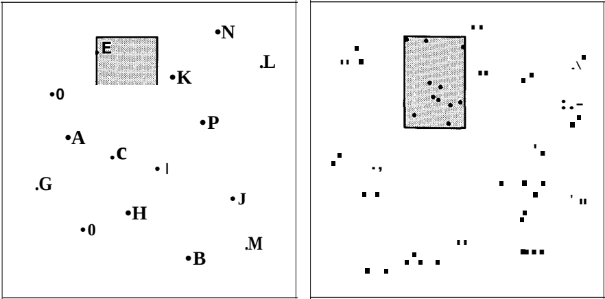
Figure 26.2 Two-dimensional range searching.
