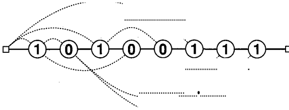
Figure 19.4 Knuth-Morris-Pratt finite-state machine (improved).
