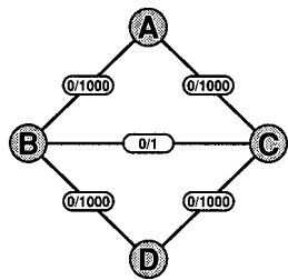
Figure 33.3 A network that could require a large number of iterations.
