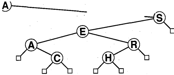
Figure 14.6 A binary search tree.
