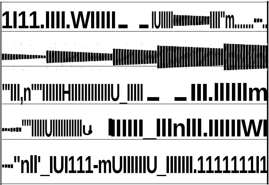
Figure 8.9 Shellsorting a Reverse-Ordered Permutation..
