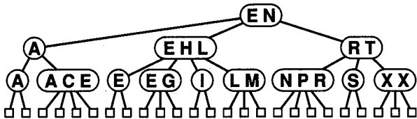
Figure 18.3 A B-tree.
