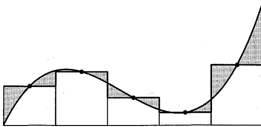
Figure 39.1 Rectangle rule.
