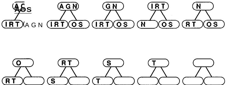
Figure 13.3 Replacement selection for merging, with heap of size three.
