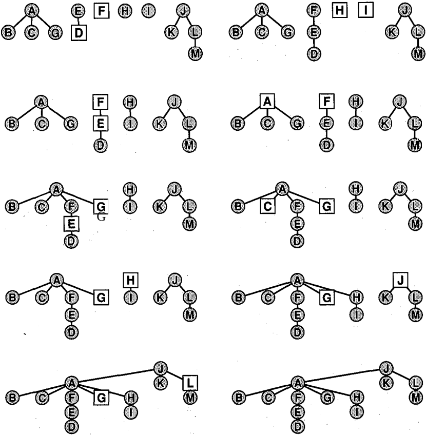
Figure 30.S Completion of union-find.
