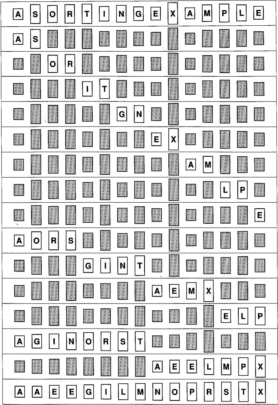
Figure 12.2 Nonrecursive Mergesort.
