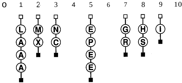
Figure 16.2 Separate chaining.
