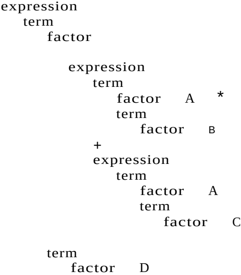
Figure 21.2 Parsing (A*B+AC)D .
