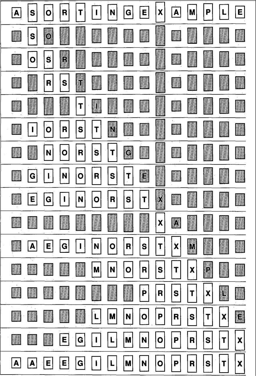
Figure 8.2 Insertion sort.
