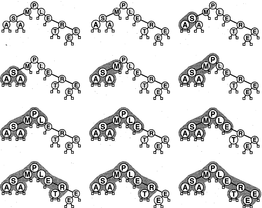
Figure 4.10 Inorder traversal.
