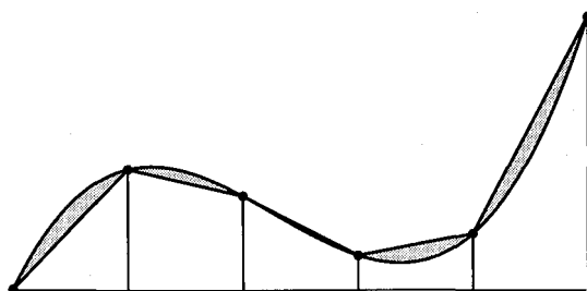
Figure 39.3 Trapezoid rule.
