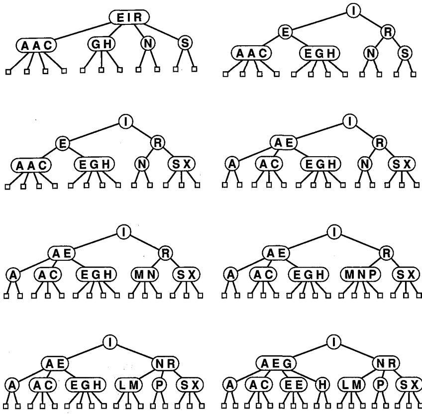
Figure 15.3 Building a 2-3-4 tree.
