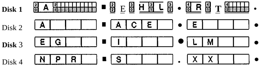
Figure 18.4 B-tree access.
