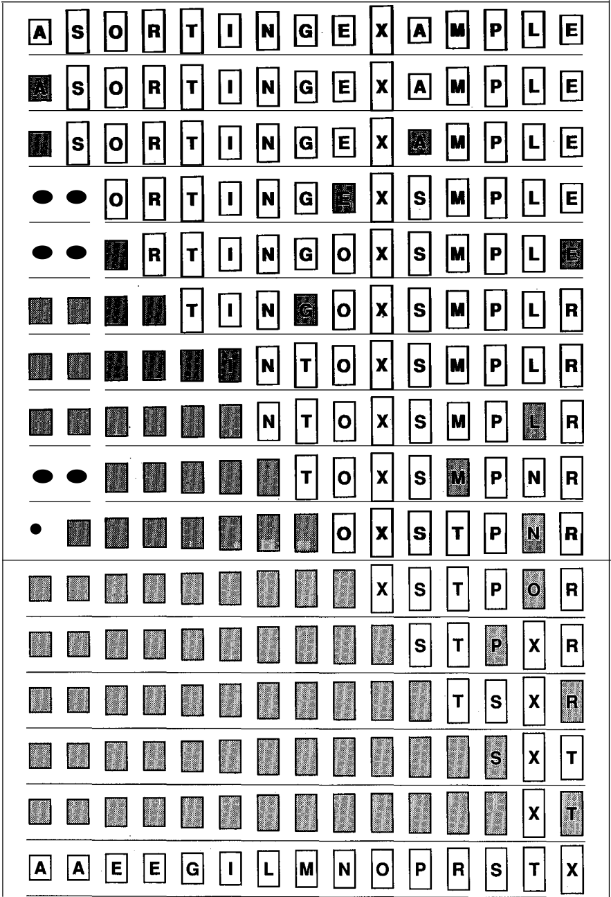
Figure 8.1 Selection sort.
