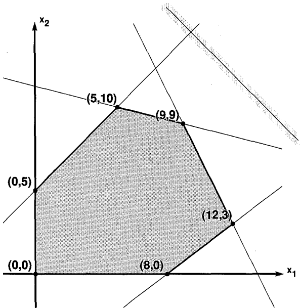
Figure 43.1 A two-dimensional simplex.
