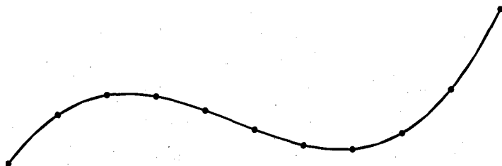
Figure 38.1 A spline through ten knots.
