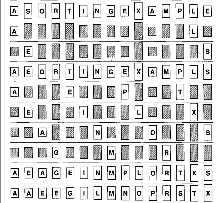
Figure 8.7 Shellsort.
