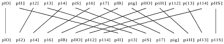
Figure 41.1 Perfect unshuffle for the FFT.
