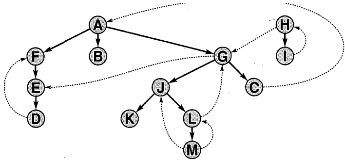
Figure 32.2 Depth-first search forest for a directed graph.
