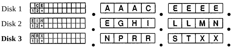
Figure 18.2 Indexed sequential access.
