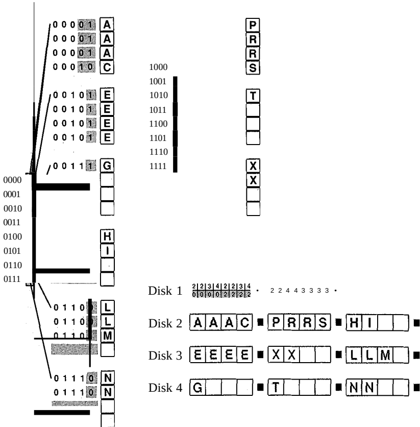
Figure 18.13 Extendible hashing access.
