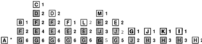
Figure 31.4 Contents of priority queue during minimum spanning tree construction.
