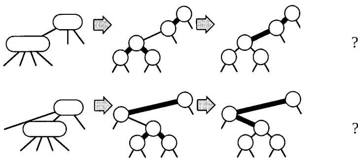
Figure 15.10 Splitting 4-nodes with a color flip: rotation needed.
