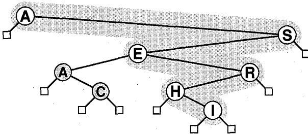
Figure 14.9 Insertion (of!) into a binary search tree.
