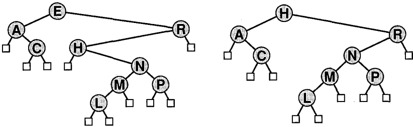
Figure 14.12 Deletion (of E) from a binary search tree.
