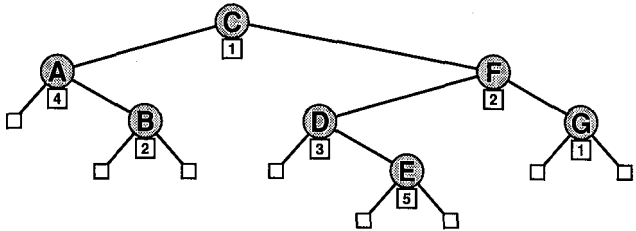
Figure 42.4 A binary search tree with frequencies.
