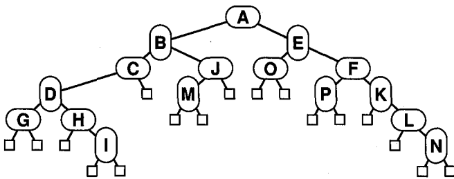
Figure 26.4 A two-dimensional (2D) tree.
