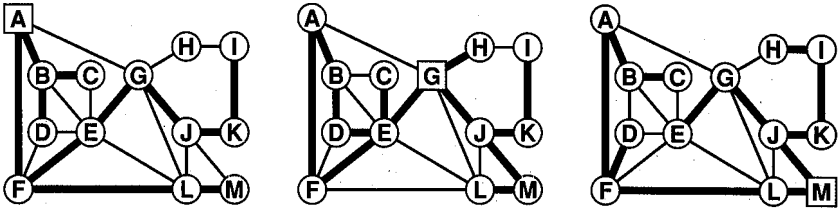
Figure 31.10 Shortest-path spanning trees.
