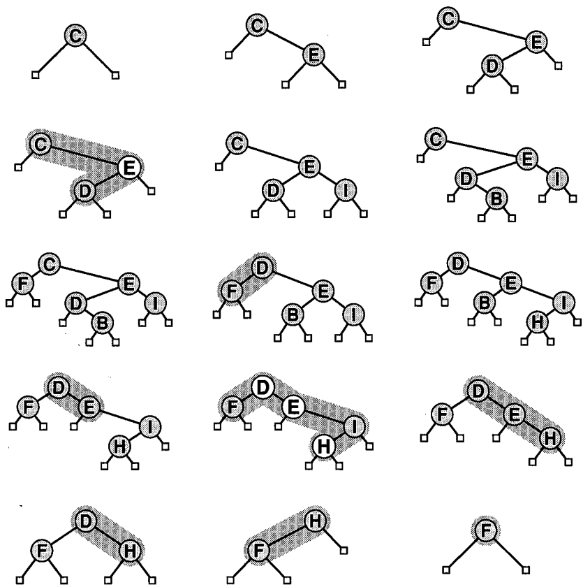
Figure 27.4 Data structure during scan: constructing the x-tree .
