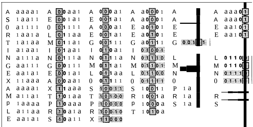
Figure 10.2 Radix exchange sort ("left-to-right" radix sort).
