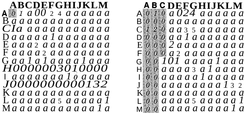
Figure 32.6 Initial stages of Floyd's algorithm.
