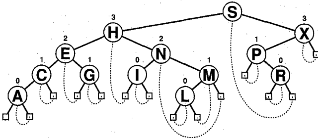
Figure 17.8 A Patricia tree.
