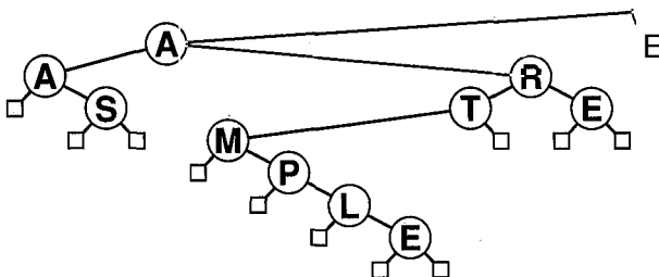
Figure 4.8 Binary tree representation of a tree.
