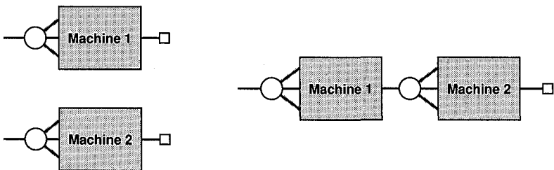
Figure 20.4 State machine construction: concatenation.
