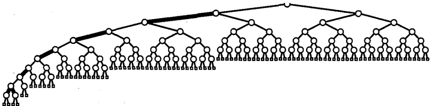
Figure 15.15 A red-black tree for a degenerate case.
