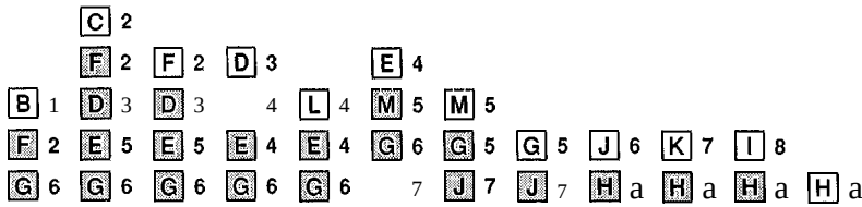
Figure 31.13 Contents of priority queue during shortest-path tree construction.
