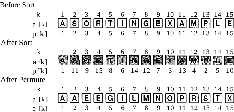
Figure 8.6 Rearranging a "sorted" array.
