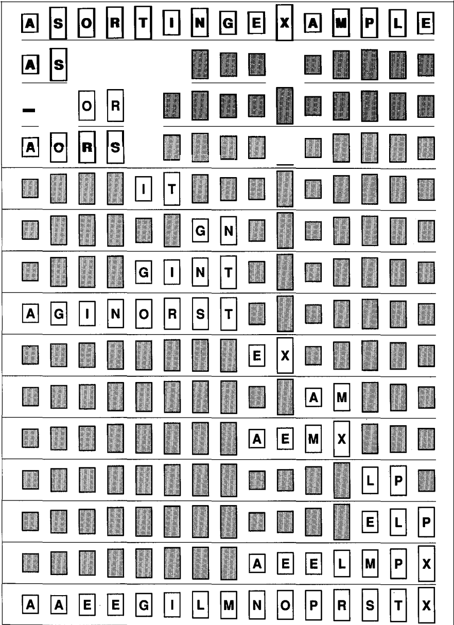
Figure 12.1 Recursive Mergesort.
