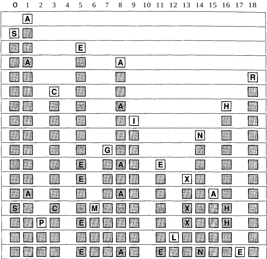
Figure 16.7 Double hashing.
