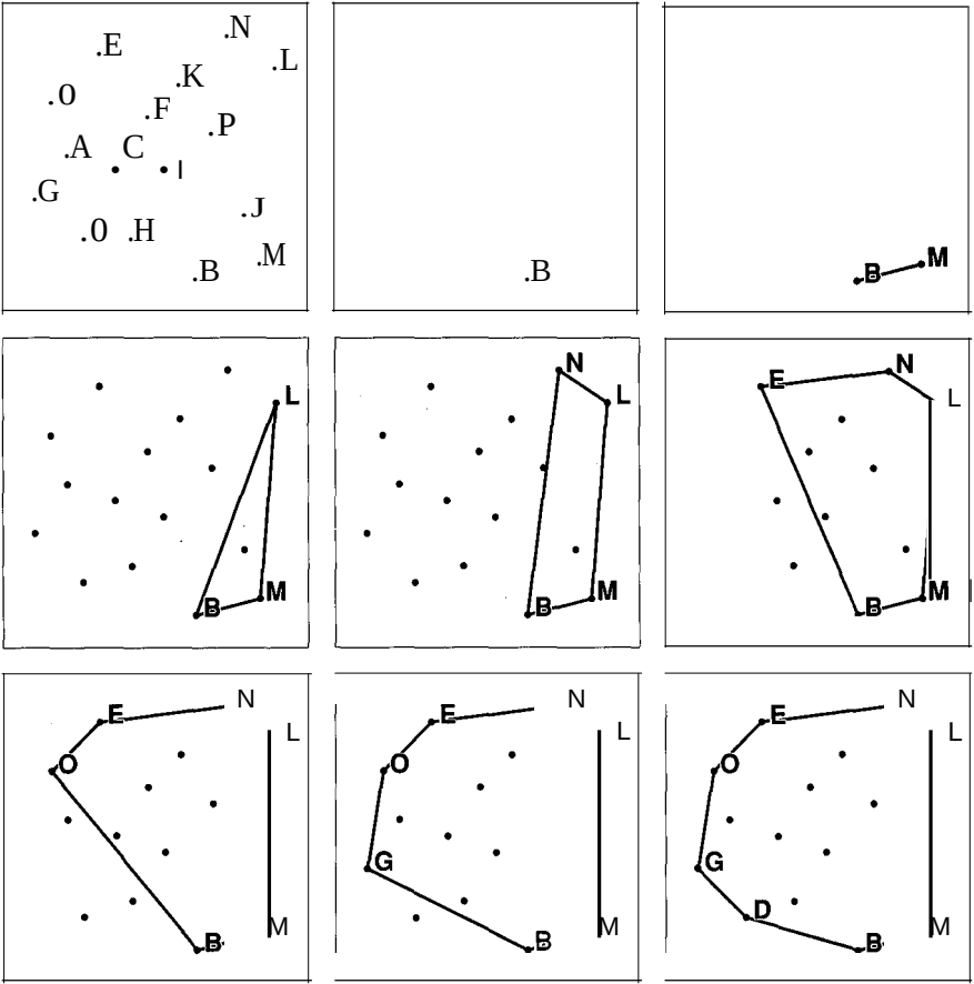
Figure 25.2 Package-wrapping.
