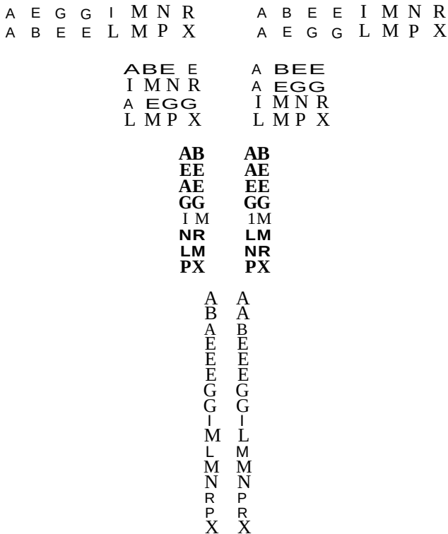
Figure 40.2 Split-and-interleave merging.
