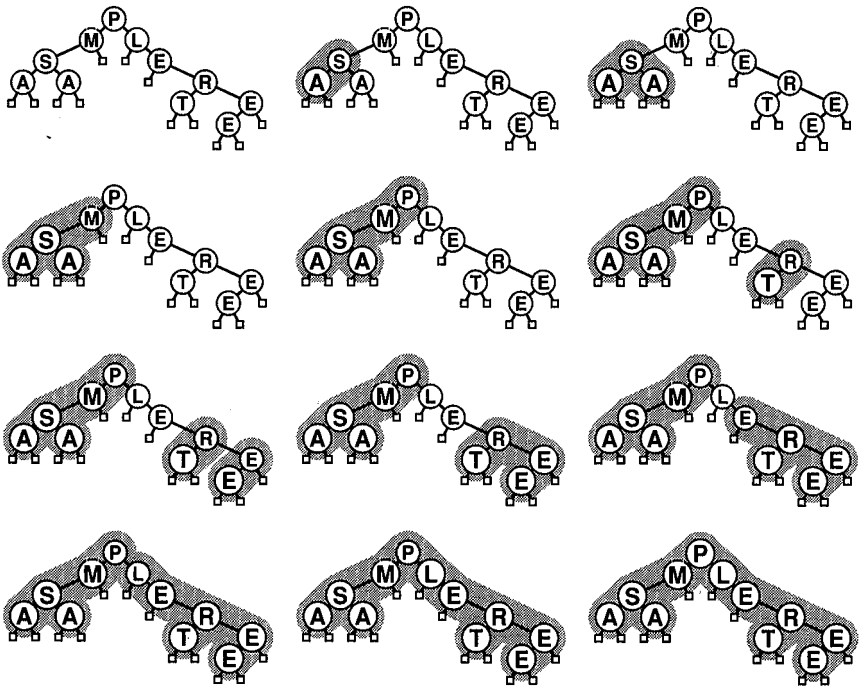
Figure 4.11 Postorder traversal.
