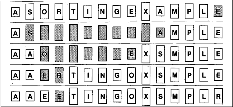
Figure 9.1 Partitioning.
