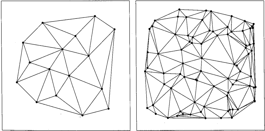
Figure 28.5 Delaunay Triangulation.
