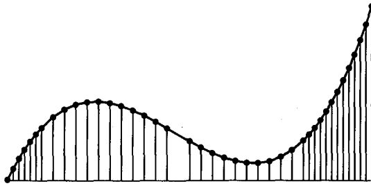
Figure 39.5 Adaptive quadrature.
