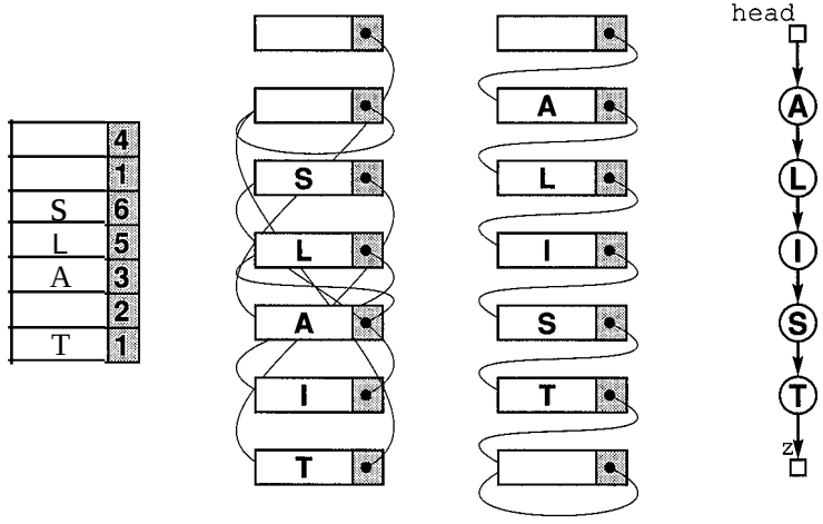
Figure 3.5 Array implementation of a linked list.
