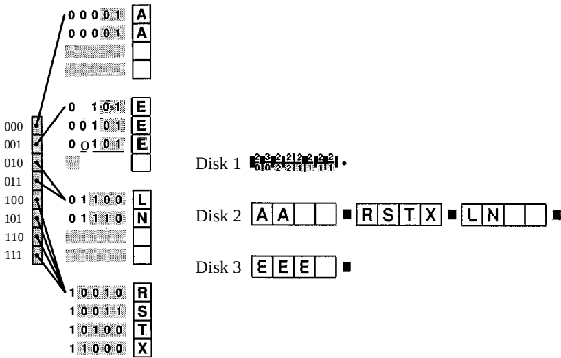
Figure 18.11 Extendible hashing: third split.
