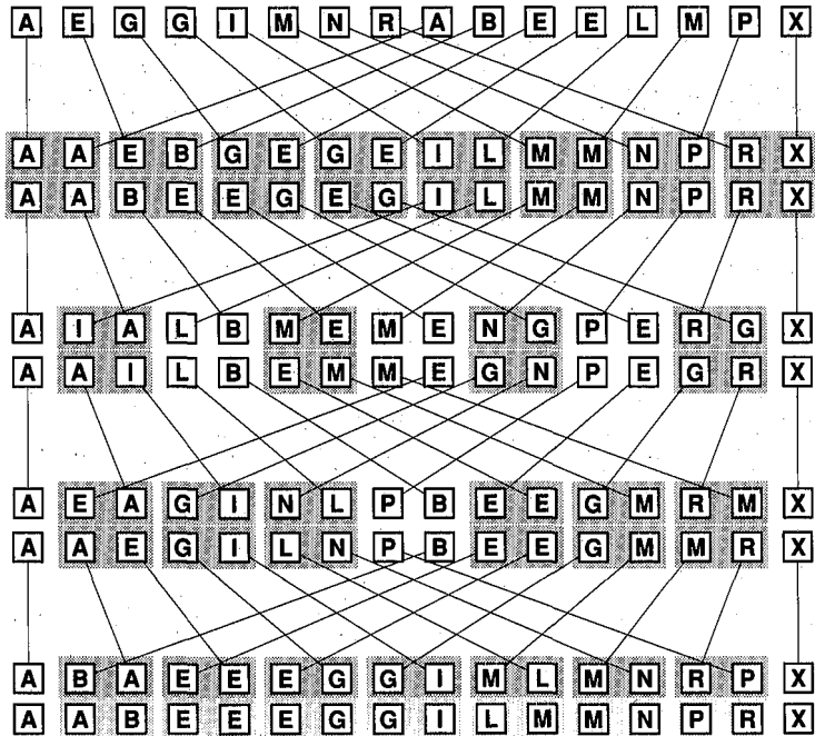
Figure 40.3 Odd-even merging with the perfect shuffle.
