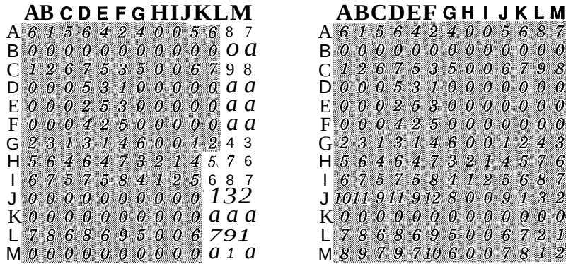
Figure 32.7 Final stages of Floyd's algorithm.
