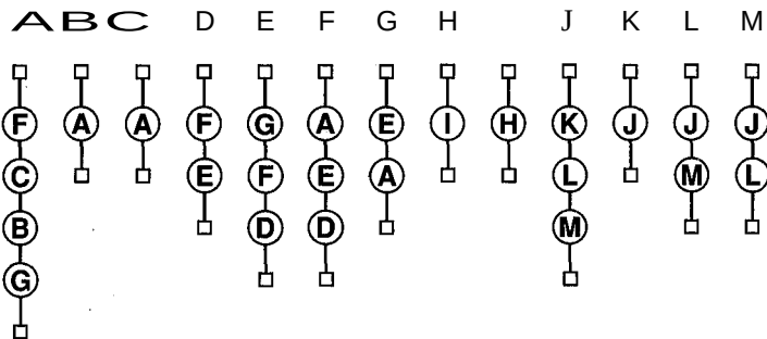
Figure 29.4 An adjacency-structure representation.
