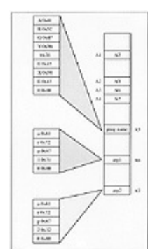
Figure 3.2 Program Organization in Memory
