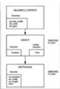
Figure 2.2 Class Structure
