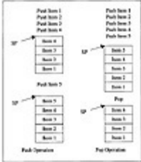
Figure 3.5 Push and Pop in a LIFO Stack
