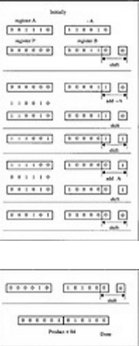
Figure 4.14 Booth Algorithm
