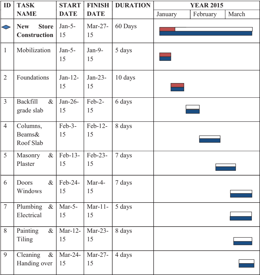
Fig. 11.2 Basic project bar chart (completion period 60 calendar days (except Saturdays and Sundays))
