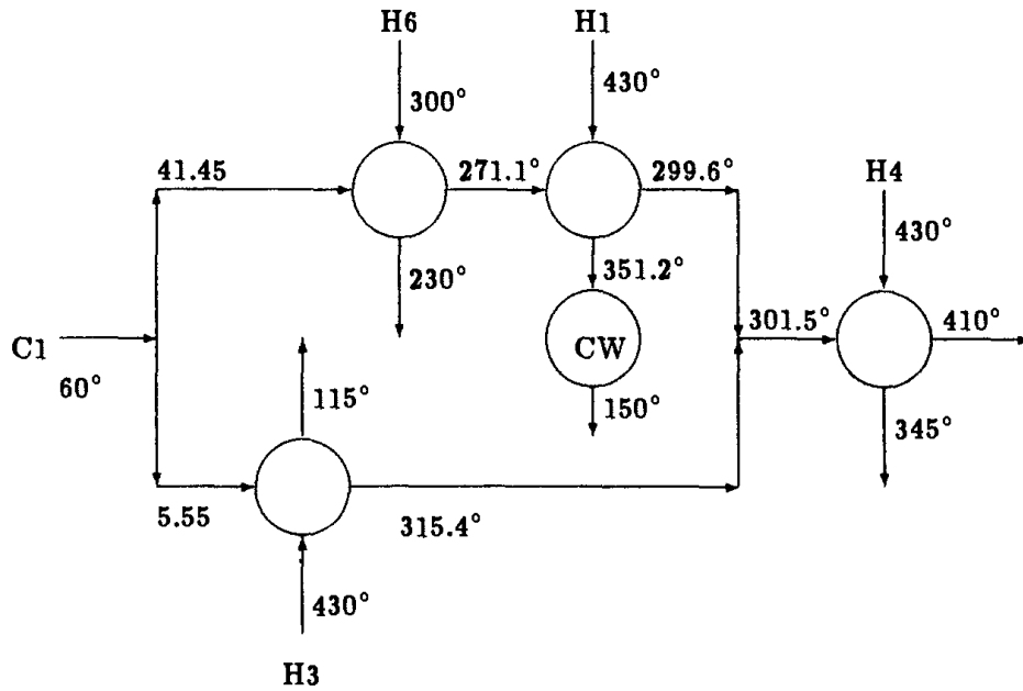
Figure 7.4: Best Known Solution to Test Problem 4
