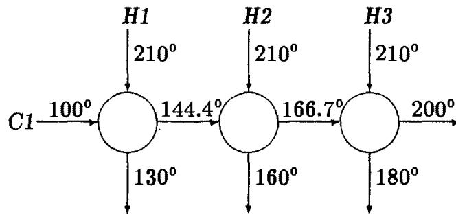
Figure 7.2: Best Known Solution to Test Problem 2
