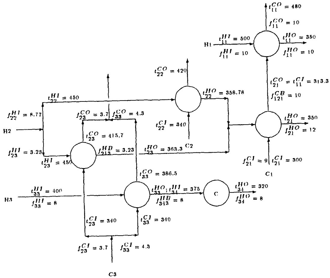
Figure 7.6: Best Known Solution to Test Problem 5
