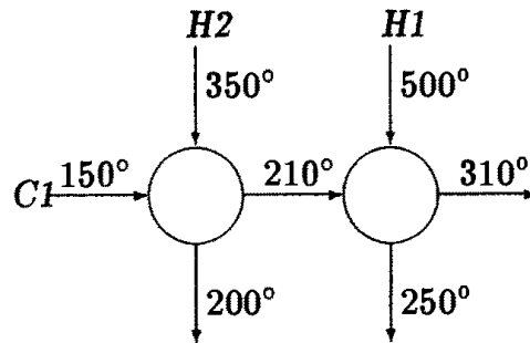
Figure 7.1: Best Known Solution to Test Problem 1
