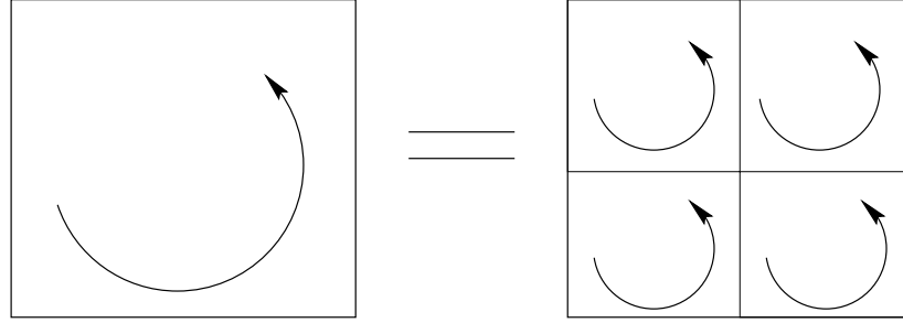
Figure 7.7: Overall boundary is equivalent to the sum of the element boundaries
