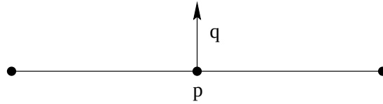
Figure 7.4: Boundary conditions at a smooth boundary
