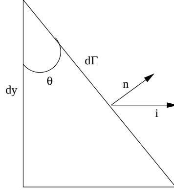
Figure 6.3: Relationship of dy to d\Gamma
