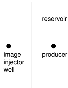
Figure 1.5: Constant pressure boundary
