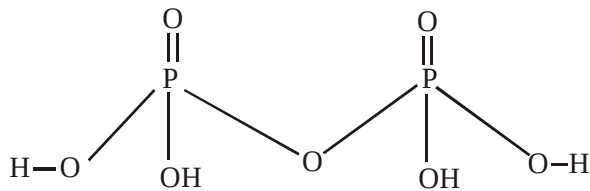
Pyrophosphoric Acid
