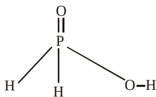
Hypophosphorus Acid
