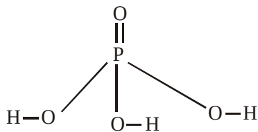
Ortho-phosphoric acid
