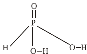
Phosphorous Acid
