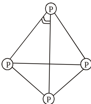
White Phosphorus
