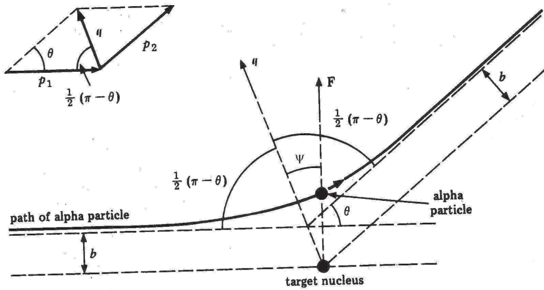
Geometrical relationships in Rutherford scattering.
